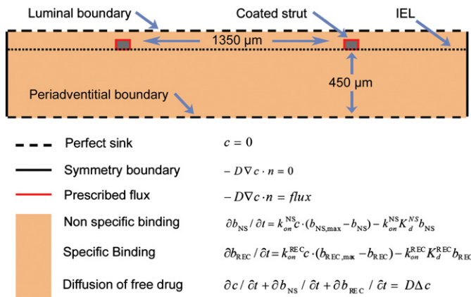
Fig. 1. Scaled schematic representation of the 2D computational domain of a tissue embedded strut pair apposed to the internal elastic lamina (IEL). Depicted here is the baseline case of conformable strut-adherent coating. Notations: t - time since stent implantation; n - unit normal; c - concentration of free drug, b NS and b REC - concentrations of, respectively, non specific - (NS) and receptor - (REC) bound drug; b NS,max and b REC,max - concentrations of NS binding sites and receptors; k on NS and k off NS - respective binding on-rate constants, K d NS and K d REC - respective equilibrium dissociation constants; D - drug diffusion coefficient in arterial tissue (for parameter values see Table S2, Supplemental Materials).
