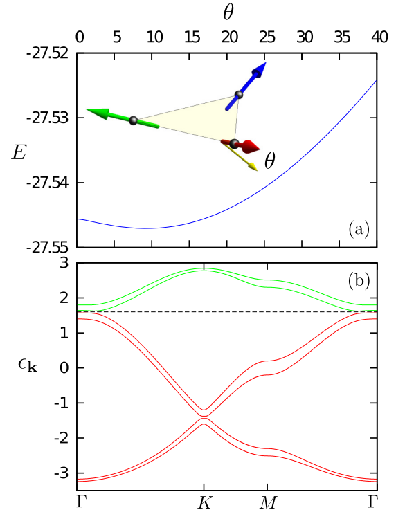
FIG. 11. (Color online) (a) The total energy (arbitrary units) as a function of the canting angle \theta for the \mathbf{Q} = \mathbf{0} umbrella state. The inset shows the three spins of the umbrella state in a triangular unit cell. This curve is obtained using the following parameters: J = 0.2t , t_2 = -0.2t . (b) The corresponding band structure with exchange coupling J = 0.2t , t_2 = -0.2t and canting angle \theta = 10^\circ . The dashed line indicates the Fermi level at f = 2/3 filling.
