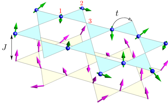
FIG. 1. (Color online) Kondo-lattice model (KLM) on the kagome lattice. The model can be viewed as consisting of two subsystems represented here by two fictitious kagome layers. Conduction electrons hop on the top layer according to a nearest-neighbor transfer integral t . The bottom layer consists of localized spins (magenta arrows) at every kagome site. The electron spins (green arrows) are coupled to the localized moments through an on-site exchange constant J . The numbers 1, 2, 3 denote the three inequivalent sublattices of kagome.
