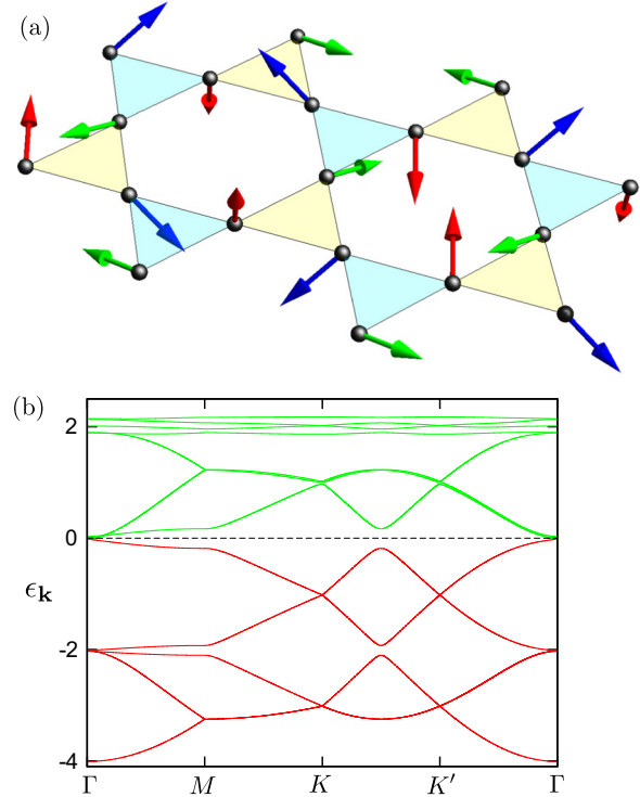
FIG. 7. (Color online) (a) The B_2 symmetry triple- \mathbf{Q} noncoplanar spin order on kagome lattice. Spins at the three inequivalent sublattices are indicated by different colors. This state is the ground state at filling fraction f = 5/12 . (b) shows the corresponding band structure calculated with exchange coupling J = 0.2t . The dashed line indicates the Fermi level at f = 5/12 filling.
