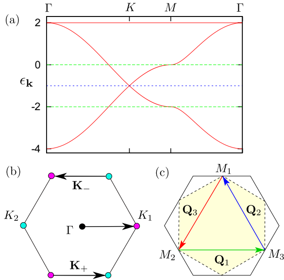
FIG. 2. (Color online) (a) Band structure of the tight-binding model on the kagome lattice. Here and in the following figures, the band energy \epsilon_{\mathbf{k}} is measured in units of NN hopping t . (b) Brillouin zone (BZ) of the kagome lattice. At filling fraction f = 1/3 , the Fermi surface shrinks to two inequivalent Dirac points K_{1,2} at the corners of the BZ. These two Dirac points are connected by wave vectors \mathbf{K}_{\pm} = (\pm 4\pi/3, 0) . (c) The dispersion has three saddle points M_{1,2,3} at the edge of the BZ, giving rise to a logarithmically divergent DOS at filling fractions f = 1/4 and 5/12 . The corresponding Fermi surface is a regular hexagon inscribed within the BZ. Pairs of parallel edges of this Fermi surface are perfectly nested by wave vectors \mathbf{Q}_1 = (2\pi, 0) and \mathbf{Q}_{2,3} = (-\pi, \pm \sqrt{3}\pi) .
