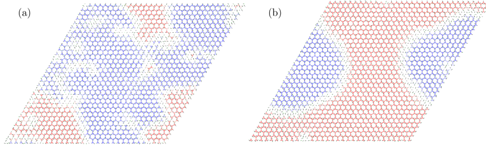
FIG. 6. (Color online) Snapshots of the scalar chirality field obtained from KPM-Langevin simulations of N = 3 \times 32^2 spins at filling fractions (a) f = 1/4 and (b) f = 7/12 . The magnetic ground state at these two filling fractions is the A_2 symmetry state shown in Fig. 4(a). At the intermediate times shown, nonequilibrium features such as chiral domain walls and \mathbb{Z}_2 vortices are apparent, although they will eventually annihilate under the (nearly) zero-temperature KPM-Langevin dynamics. We use a moderate coupling constant of J = 0.5t for these simulations.
