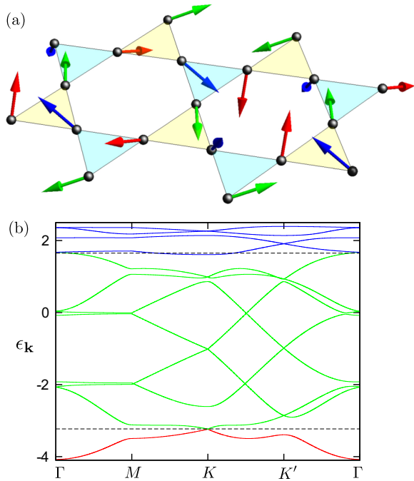
FIG. 10. (Color online) (a) The B_1 symmetry triple- \mathbf{Q} noncoplanar spin order on the kagome lattice. Spins at the three inequivalent sublattices are indicated by different colors. It is the ground state at filling fraction f = 2/3 for weak couplings. The same magnetic order is also the ground state at filling fraction f = 1/12 for intermediate couplings. (b) The corresponding band structure with exchange coupling J = 0.4t . The two dashed lines indicate the Fermi levels at f = 1/12 and f = 2/3 filling fractions.
