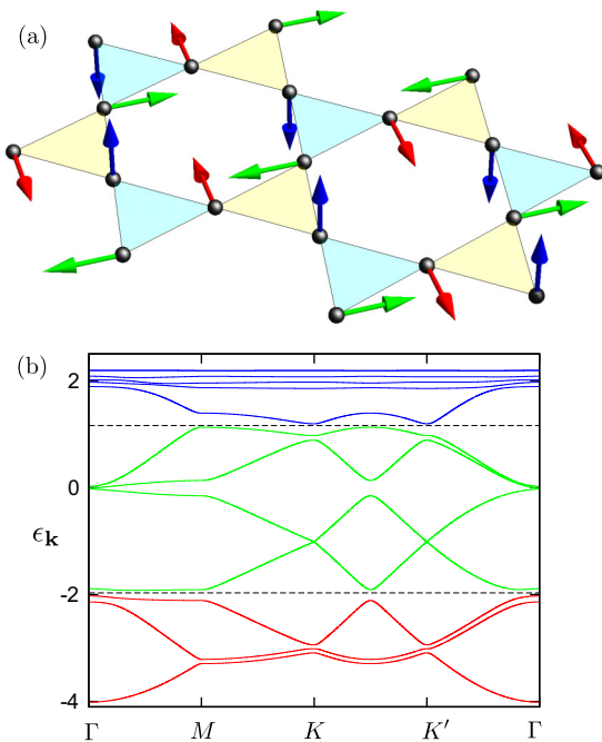
FIG. 4. (Color online) (a) The triple- \mathbf{Q} noncoplanar (orthogonal) spin order on kagome lattice that transforms according to the A_2 irreducible representation of the symmetry group. Spins at the three inequivalent sublattices are indicated by different colors. This A_2 symmetry state is the ground state at filling fraction f = 1/4 (for J \lesssim 2.2t ) and f = 7/12 (for J \lesssim 1.3t ). The corresponding band structure is shown in panel (b). The exchange coupling J = 0.22t is used in the calculation. The dashed lines indicate the Fermi levels at filling fractions f = 1/4 and 7/12 .
