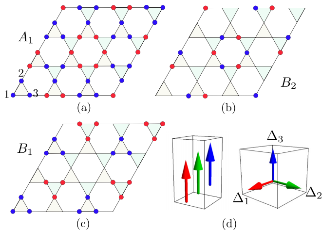
FIG. 3. (Color online) (a)–(c) Schematic diagram showing the triple- \mathbf{Q} scalar order (or collinear spin order) corresponding to the three irreducible representations A_1 , B_2 , and B_1 . The blue (red) circles denote on-site scalar variable \zeta_i = +1 ( -1 ), while empty site corresponds to \zeta_i = 0 . (d) shows the collinear and orthogonal configurations of the triple- \mathbf{Q} vector order parameters.
