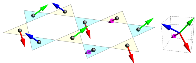
FIG. 5. (Color online) The chiral structure of spin orders at van Hove fillings in the kagome lattice. There is a vector associated with each triangle. The four different orientations of the vectors (indicated by four different colors) point to the corners of a regular tetrahedron. The vectors associated with each triangle correspond to the total spins \mathbf{M}_\Delta = \mathbf{S}_1 + \mathbf{S}_2 + \mathbf{S}_3 in the A_2 symmetry order at f = 1/4 filling [Fig. 4(a)], and to the vector chirality \chi_\Delta = \mathbf{S}_1 \times \mathbf{S}_2 + \mathbf{S}_2 \times \mathbf{S}_3 + \mathbf{S}_3 \times \mathbf{S}_1 in the B_2 symmetry order at the second van Hove filling f = 5/12 [Fig. 7(a)].
