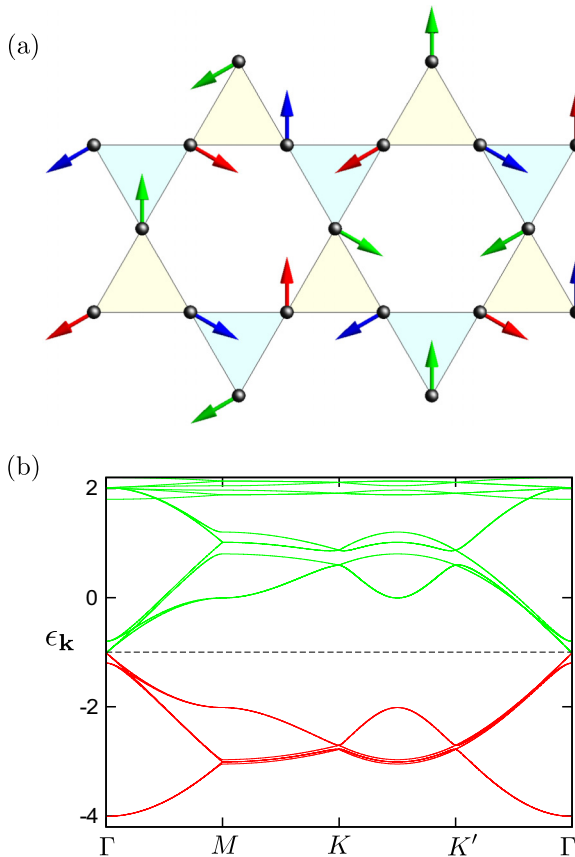
FIG. 9. (Color online) (a) The \sqrt{3} \times \sqrt{3} coplanar spin order on kagome lattice at filling fraction f = 1/3 . Spins at the three inequivalent sublattices are indicated by different colors. (b) The corresponding band structure with exchange coupling J = 0.2t . The dashed line indicates filling fraction f = 1/3 .
