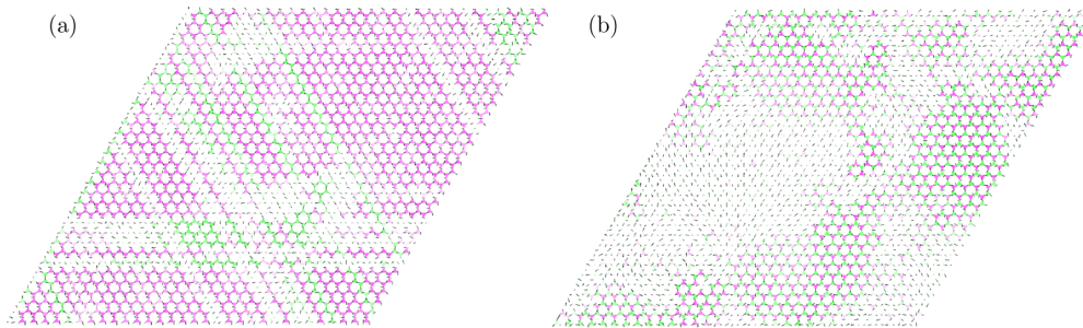
FIG. 8. (Color online) Snapshots of two metastable spin configurations obtained from large-scale KPM-Langevin simulations of N = 3 \times 32^2 spins for filling fraction f = 5/12 . The color indicates the z component of the vector chirality \chi_\Delta = \mathbf{S}_1 \times \mathbf{S}_2 + \mathbf{S}_2 \times \mathbf{S}_3 + \mathbf{S}_3 \times \mathbf{S}_1 . The two panels show (a) ferromagnetic and (b) antiferromagnetic alignments of \chi_\Delta . These two 120^\circ coplanar orderings have nearly identical energy densities, so entropy and nonequilibrium effects determine the ordering found in our KPM-Langevin simulations.
