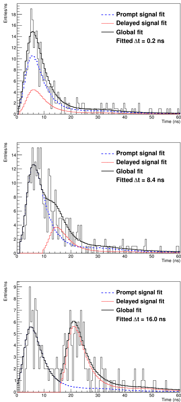
Figure 4. Three examples of o-Ps fit. The dashed blue line represents the fit of the first time profile, the thin red line the fit of the second one and the thick black line is the total fit.
