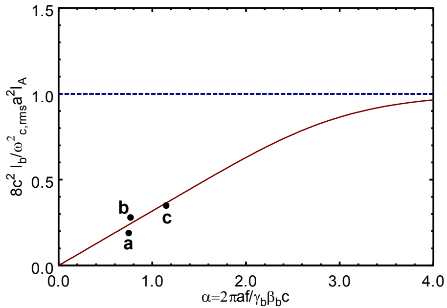
Figure 5-3: Plot of the maximum value of the self-field parameter (solid curve), 8c^2 I_b / \omega_{c,rms}^2 a^2 I_A , for bunched beam confinement as a function of the parameter \alpha = 2\pi a f / \gamma_b \beta_b c . Shown in letters are the operating points for three PPM focusing klystrons: a) 50 MW XL-PPM, b) 75 MW XP, and c) Klystrino. The dashed line denotes the Brillouin density limit for an unbunched beam.
