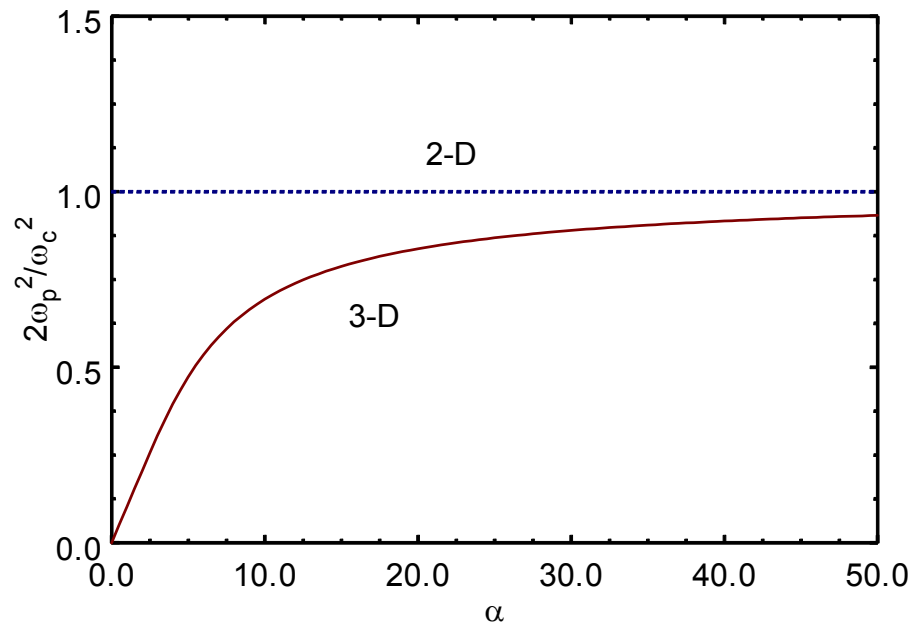
Figure 6-7: Plot of the maximum self-field parameter 2\omega_p^2/\omega_c^2 (solid) for the large bunched beam rigid-rotor equilibrium as a function of \alpha = 2\pi a/\gamma_b L . Also shown is the Brillouin density limit 2\omega_p^2/\omega_c^2 = 1 (dashed), which corresponds precisely to the unbunched rigid-rotor limit.
