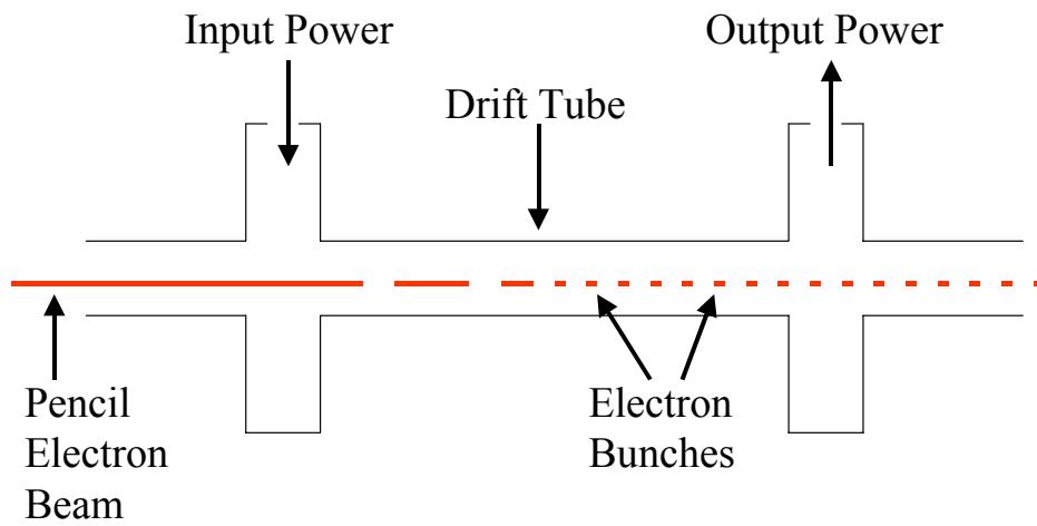
Figure 1-2: Schematic of a klystron amplifier, which shows an unbunched pencil thin electron beam interacting with an input cavity and forming electron bunches in a drift tube. The bunches then excite the output cavity, and generate radiation.
