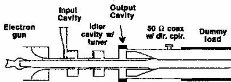
Figure 7-1: Schematic of the LANL RKA experiment (from Fazio, et al. , 1994)
