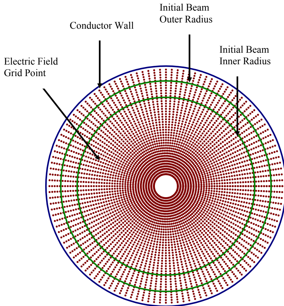
Figure 8-3: Diagram of the electric field grid points chosen for chosen for the LANL RKA simulation. The location of the conductor wall, as well as the initial inner and outer radii for the beam, are labeled in the diagram.
