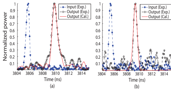
FIG. 5: Pulse shapes for an input pulse of 600 ps at the 35.4 kV operating point. The output pulse at (a) 137.3 GHz has a measured width of 1045 ps and (b) at 138.13 GHz has a measured width of 660 ps.
