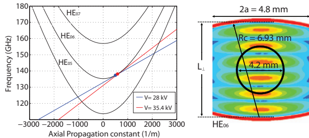
FIG. 1: Diagram of the dispersion relation for the Gyro-TWT interaction in a confocal waveguide (left) and the confocal waveguide shown in cross section (right). The annular electron beam has a 4.2 mm diameter.
