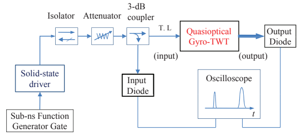
FIG. 2: Schematic diagram of the picosecond pulse amplification in a quasioptical Gyro-TWT.
