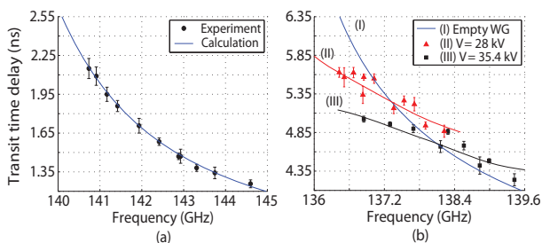
FIG. 4: Measured and calculated transit time delay of 500 ps pulses in (a) WR4 waveguide with a cutoff frequency of 139.25 GHz and (b) the Gyro-TWT confocal waveguide structure with a cutoff frequency of 135.0 \pm 0.3 GHz. Solid lines represent calculated values and filled circles, triangles and squares are experimental results.
