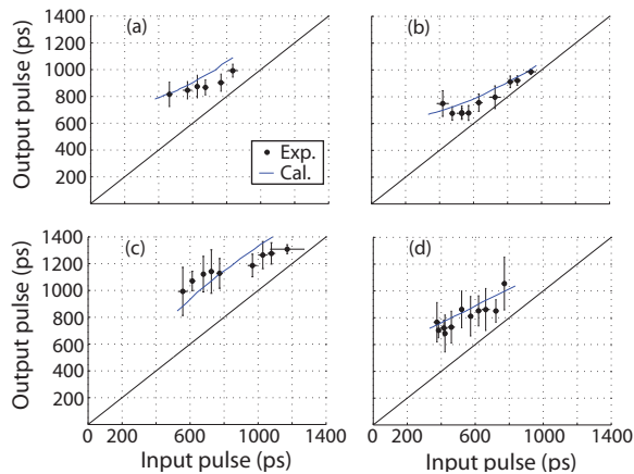
FIG. 6: Measured (dots) and calculated (solid line) output pulse widths after amplification as a function of input pulse width; (a) 28 kV and 137.4 GHz; (b), (c), and (d) are for 35.4 kV and (b) 138.13 GHz, (c) 137.3 GHz, and (d) 138.8 GHz. A solid line is drawn for the output pulse length equal to the input, which applies for long pulses > a few ns.
