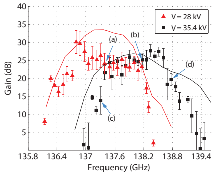
FIG. 3: Measured and calculated gain-bandwidth curves for beam voltages of 35.4 and 28 kV. The points labeled (a), (b), (c), and (d) correspond to the labels in Fig. 6 below.
