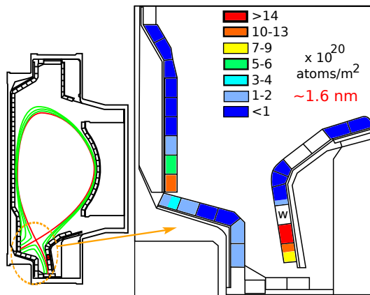
Figure 1: Eroded tungsten from the W row forms a distinct migration pattern with deposition on the C-Mod outer divertor, inner divertor, and divertor dome.
