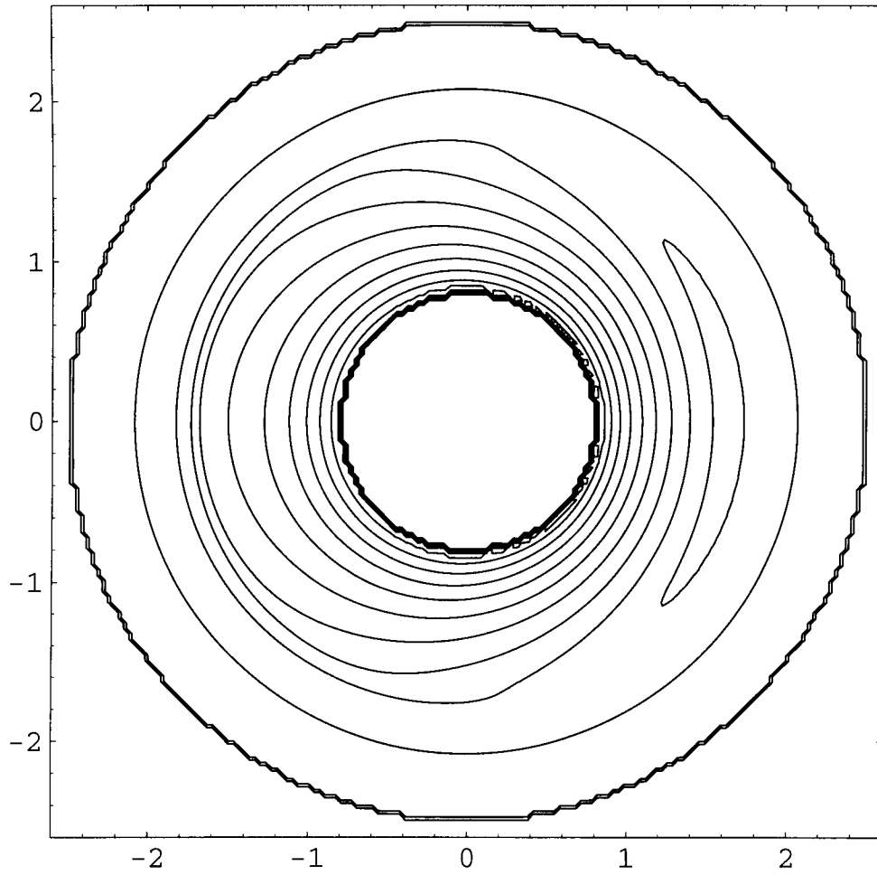
Fig. 4. Midplane Contours of perturbed potential ( f=1.3 KHz)
