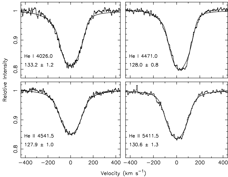
Figure 10. Average profiles of the four helium lines used to determine the rotational velocity (“histograms”), and the best-fitting model profiles for each (smooth curves). The line identification and the derived value of V_{\text{rot}} \sin i in \text{km s}^{-1} are given in each panel.
