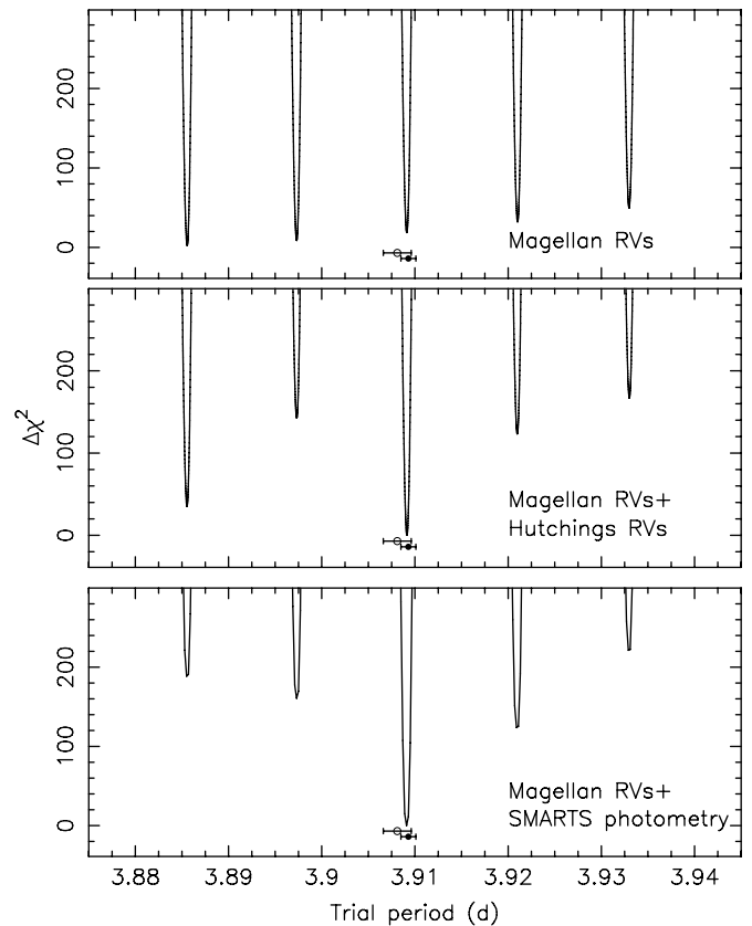
Figure 7. Top: \chi^2 computed using a three-parameter sinusoid vs. the trial period for the Magellan radial velocities. Center: the periodogram (computed in a similar manner as above) for the radial velocities from Hutchings et al. (1983, 1987) combined with the Magellan radial velocities. Bottom: the periodogram derived from the SMARTS photometry and the Magellan radial velocities (see the text). The best-fitting period is found to be 3.90917 \pm 0.00005 , and all other possible alias periods are ruled out at high confidence. In each of the three panels the X-ray period given in Levine & Corbet (2006) is indicated with an open circle, and the refined X-ray period is denoted by the filled circle.
