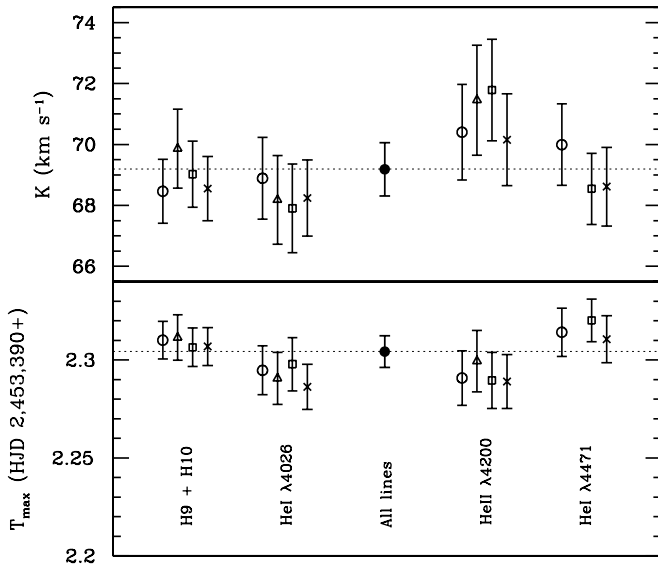
Figure 4. Summary of fitted values of the velocity semiamplitude K (top) and the time of maximum velocity T_{\max} (bottom) for different combinations of bandpasses, template spectra, and modes of filtering. The lines or line group are indicated at the bottom of the figure (see the text). The open and filled circles are for template HD 93843 and Legendre filtering. Triangles: HD 101205, Legendre filtering. Squares: synthetic template, Legendre filtering. Crosses: synthetic template, Fourier filtering. The filled circles and dashed lines correspond to the values of K and T_{\max} given in the text, which were computed for the mean velocities. The uncertainties shown are purely statistical, correspond to \chi^2_{\nu} = 1 , and are at the 1\sigma level of confidence. No results are shown for the He I \lambda 4471 line for HD 101205 because the template spectrum was corrupted in this band.
