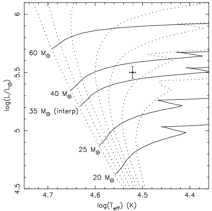
Figure 14. Solid lines show evolutionary tracks for an LMC metallicity on a temperature–luminosity diagram for stars with ZAMS masses of 60 M_{\odot} , 40 M_{\odot} , 25 M_{\odot} , 20 M_{\odot} taken from Meynet et al. (1994). The track for a ZAMS mass of 35 M_{\odot} was crudely interpolated. The dotted lines show isochrones (also for an LMC metallicity; Lejeune & Schaerer 2001) from left to right of 0, 1, 2, 3, 4, 5, and 6 Myr. The location of the LMC X-1 secondary is very close to the interpolated track for the 35 M_{\odot} star and the 5 Myr isochrone.
