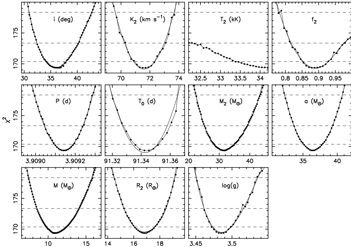
Figure 13. Curves of \chi^2 vs. various fitting and derived parameters of interest for the circular orbit model. The horizontal dashed lines denote the 1, 2, and 3\sigma confidence limits.
