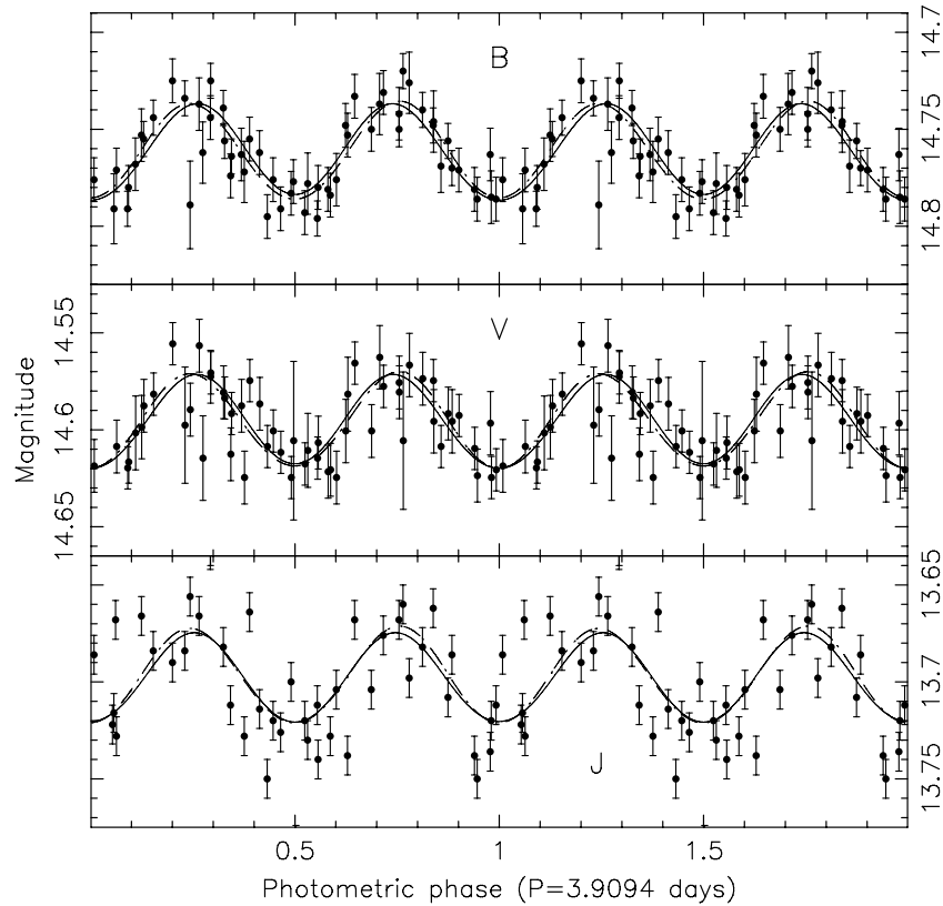
Figure 2. Phased light curves of LMC X-1. Phase zero corresponds to the time of the inferior conjunction of the secondary star. Shown from the top are the B , V , J light curves with the best-fitting ellipsoidal models assuming a circular orbit (solid lines) and assuming an eccentric orbit (dashed lines). Owing to the large scatter, the J -band data were not used in the modeling.
