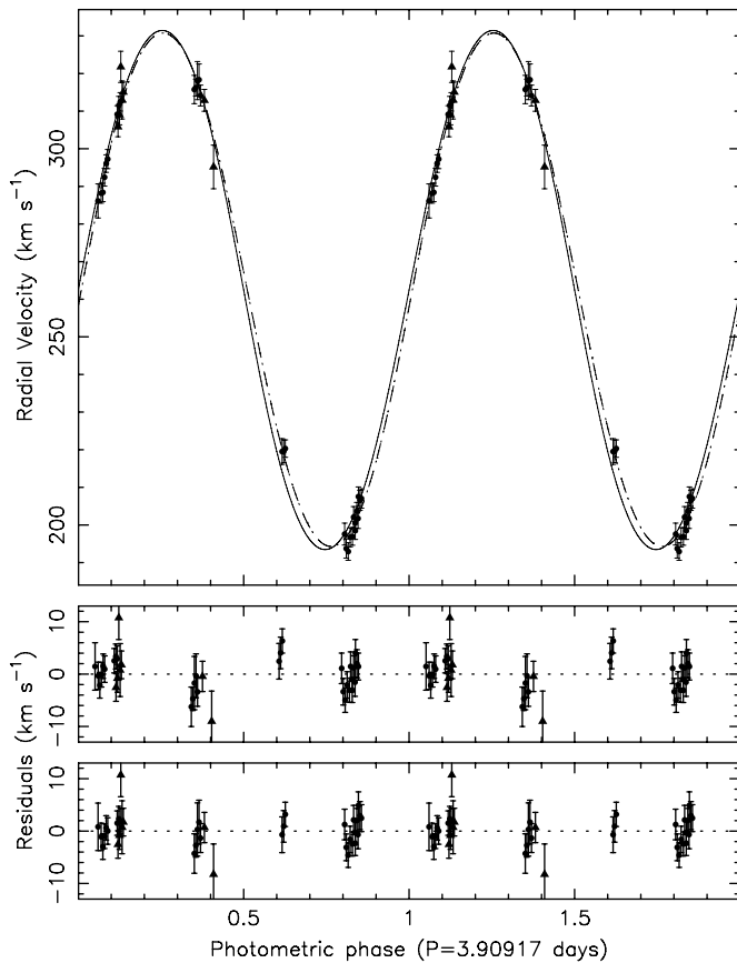
Figure 6. Top: the phased velocity curve of LMC X-1. Phase zero corresponds to the time of the inferior conjunction of the secondary star. The MIKE radial velocities are shown with the filled circles and the MagE radial velocities are shown with the filled triangles. The model curve for the best-fitting orbital model assuming a circular orbit is shown with the solid line, and the model curve for the best-fitting model assuming an eccentric orbit is shown with the dashed lines. Center: the residuals with respect to the circular orbit model. Bottom: the residuals with respect to the eccentric orbit model.
