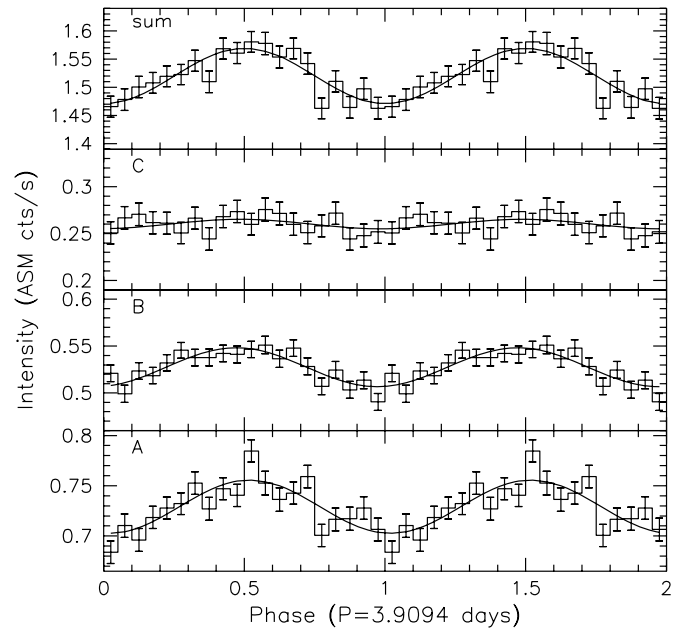
Figure 9. RXTE ASM light curves of LMC X-1 folded using a period of 3.9094 days and an epoch of phase zero of MJD 53390.75174. The four panels from bottom to top show the data from the A (1.5–3 keV), B (3–5 keV), and C (5–12 keV) bands, and the sum of the three bands (nominally comprising photon energies 1.5–12 keV). The error bars indicate \pm 1\sigma statistical uncertainties. The smooth curves are the best-fit functions of the form f(\phi) = a_0 + a_1 \cos(2\pi\phi) + a_2 \sin(2\pi\phi) (see Table 1 for the best-fitting parameters).
