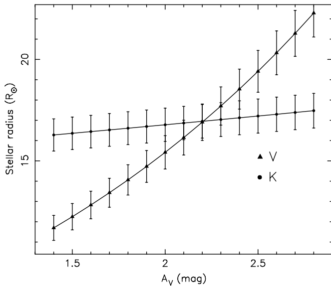
Figure 11. Radius of the companion as a function of the extinction A_V for the V band (triangles) and the K band (circles). The radius is the same for both bands when the extinction is \approx A_V = 2.2 mag.
