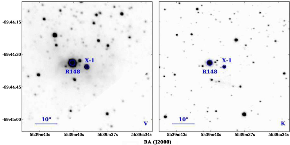
Figure 1. 1 \times 1 arcmin finding charts for the field surrounding LMC X-1 obtained with the Magellan–Baade telescope. The left panel is a V -band image obtained with the IMACS imaging spectrograph, sampled at 0''.22 \text{ pixel}^{-1} under seeing of 0''.8 . The right panel is the same field observed in the K band using the PANIC camera with 0''.125 \text{ pixel}^{-1} sampling and a seeing of 0''.55 . The correct counterpart together with the nearby B5 supergiant R148 are marked.
