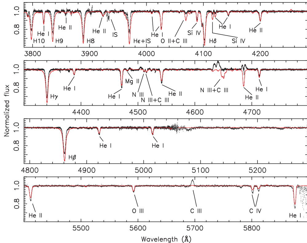
Figure 3. Average spectrum of LMC X-1 in the rest frame of the secondary star (black dots) obtained with the MIKE. Most of the strong features are labeled, and interstellar lines are marked with “IS”. The best-fitting model (red line) has T_{\text{eff}} = 33,225 K, \log g = 3.56 , and V_{\text{rot}} \sin i = 128.0 km s ^{-1} . The noise near 5060 Å is caused by the transition from the blue arm to the red arm.
