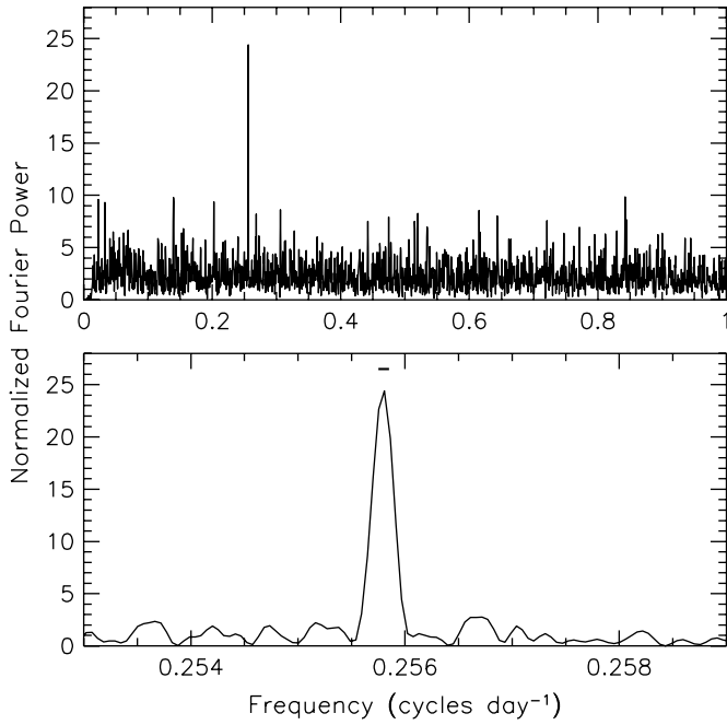
Figure 8. PDS of a 1.5–12 keV ASM light curve of LMC X-1 that has been modified to remove variability on timescales longer than \approx 30 days (see the text). The original FFT was oversampled by a factor of 4 and had approximately 62,000 frequencies from 0 cycles \text{day}^{-1} to the Nyquist frequency of 3.3 cycles \text{day}^{-1} . Top: the low frequency part of a rebinned PDS in which the number of frequency bins was reduced by a factor of 10 by using the maximum power in each contiguous set of 10 frequency bins in the original PDS as the power of the corresponding bin in the rebinned PDS. Bottom: a portion of the original PDS. The horizontal bar above the peak shows our estimate of the possible values of the centroid frequency, i.e., 0.25580 \pm 0.00005 \text{ day}^{-1} . In both panels, the power is normalized relative to the PDS-wide average.
