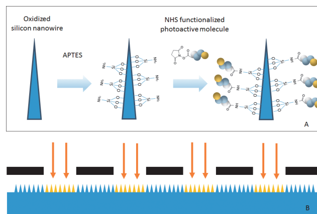
Fig 1. Experimental approach and and set-up for photo-attachment. A: Chemical reaction approach for photo-attachment of biomolecules on nanowire surface. B: Simple set up for photo-attachment. The black parts in Fig. 1B represents opaque region of photomask. The yellow region represents photo-attached nanowires.
