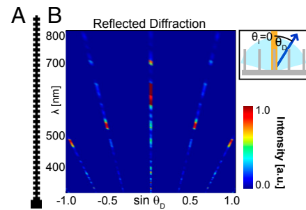
Fig. 4. Diffraction discretization. (A) One- \mu\text{m} -wide unit cell for diffraction grating simulated via FDTD. (B) Reflected spectra calculated from FDTD simulation of A showing bright spots in each diffracted order with discrete jumps in the diffracted wavelength.
