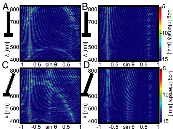
Fig. 3. Modeling of the expected diffraction patterns originating from the ordered array of gratings with 45^\circ illumination. (A) Calculated diffraction pattern for upright plates with scallops. (B) Calculated diffraction pattern for upright plates without scallops. (C) Calculated diffraction pattern for 23^\circ tilted plates with scallops. (D) Calculated diffraction pattern for 23^\circ tilted plates without scallops.
