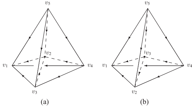
FIG. 2. (a) Defining graph of the 4-cocycle [v_1v_2, v_2v_3, v_3v_4, v_4v_5] . (b) For [v_1v_2, v_2v_3, v_3v_4, v_4v_5]^{-1} .
