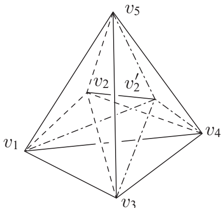
FIG. 3. Topology of the action of A_v^g . The arrows are omitted for simplicity because the vertex ordering is explicit.
