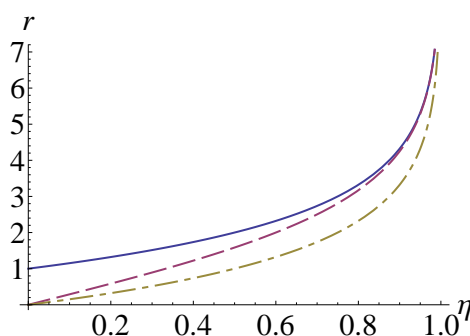
Figure 2. Secret-key rate (in bits per transmitted mode) vs channel transmissivity. Blue solid line: Achievable secret-key rate by quantum data locking (20). Red dashed line: Upper bound for the secret-key rate (assisted by two-way public communication) according to the standard security definition [2]. Yellow dash-dotted line: Achievable secret-key rate according to the standard security definition as given by the reverse coherent information [22].
