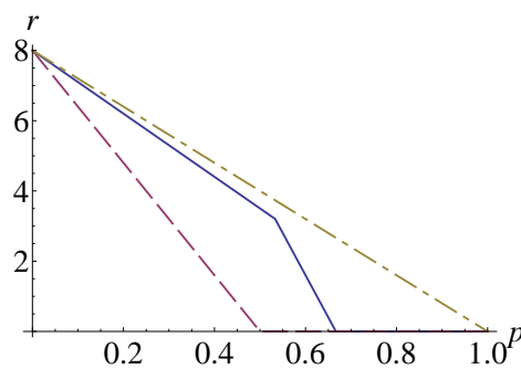
Figure 1. Comparison of several communication rates (in bits per channel use) for the qudit erasure channel with erasure probability p , with d = 256 . Weak-locking rate (solid line); private capacity (dashed line); classical capacity (dot-dashed line).
