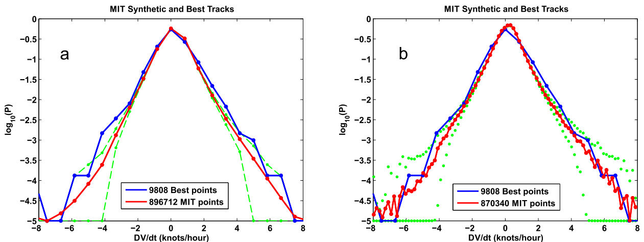
FIG. 2. As in Fig. 1, but including all intensities of tropical storm strength or larger.
