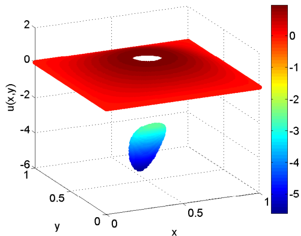
Figure 6: Example 1 - numerical solution with 193 \times 193 nodes.
