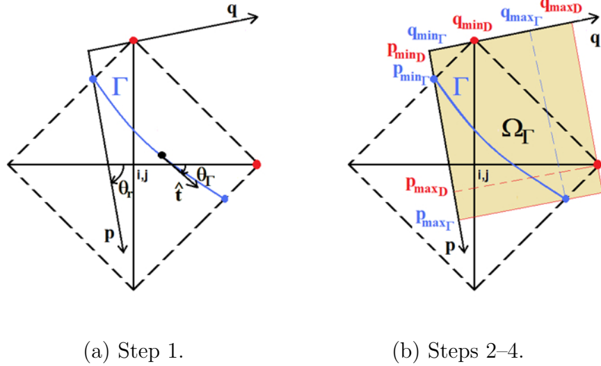
Figure C.2: The set \Omega_\Gamma^{i,j} for the situation in figure C.1.
