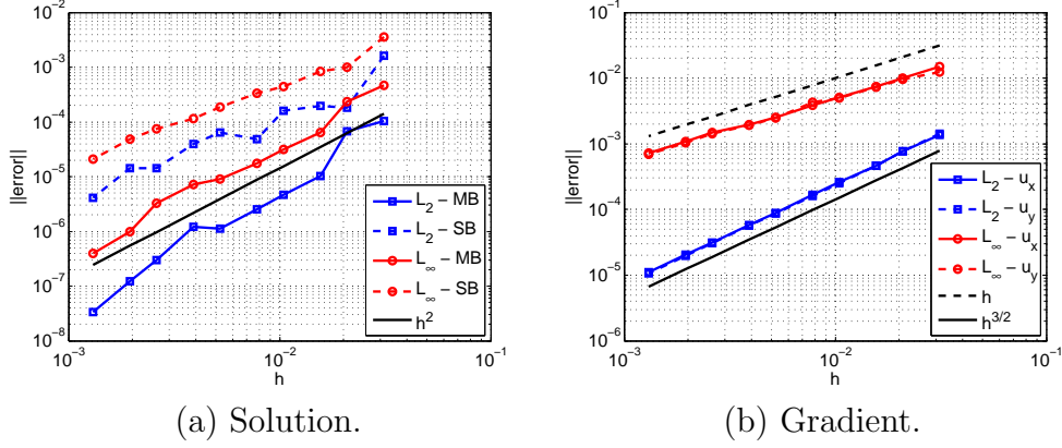
Figure C.4: Example 1 s - Error behavior of the solution and its gradient in the L_2 and L_\infty norms.
