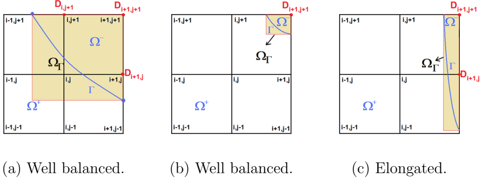
Figure B.2: \Omega_{\Gamma}^{i,j} as defined by the compact grid-aligned stencil-centered approach.
