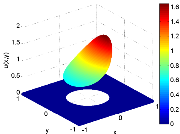
Figure C.7: Example 3 s . Numerical solution with 161 \times 161 nodes.
