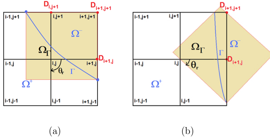
Figure B.3: \Omega_\Gamma^{i,j} as defined by the free stencil–centered approach.
