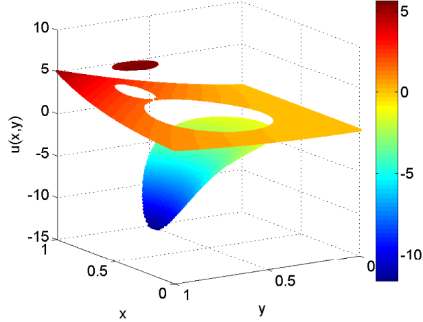
Figure 12: Example 4 - numerical solution with 193 \times 193 nodes.
