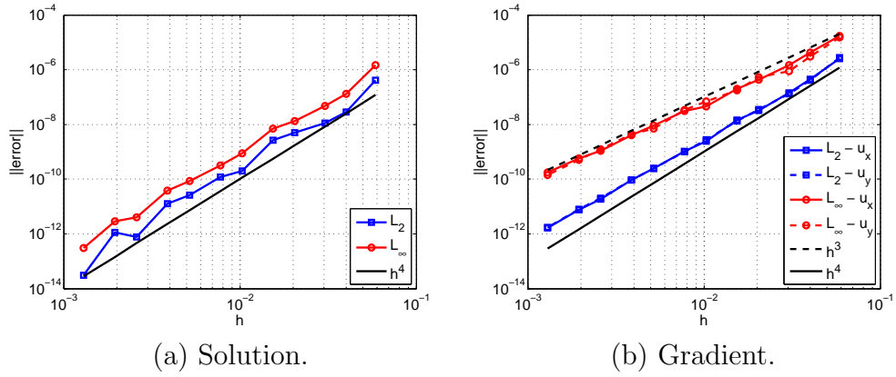
Figure 9: Example 2 - Error behavior of the solution and its gradient in the L_2 and L_\infty norms.
