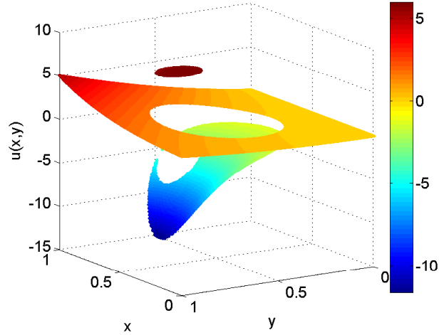
Figure 14: Example 5 - numerical solution with 193 \times 193 nodes.
