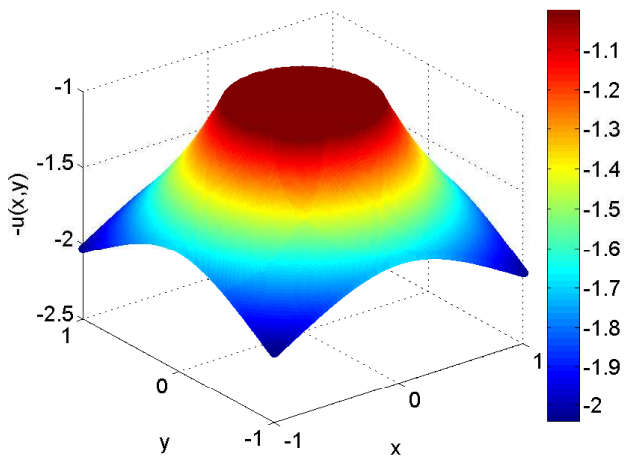
Figure C.5: Example 2_s . Numerical solution with 161 \times 161 nodes.
