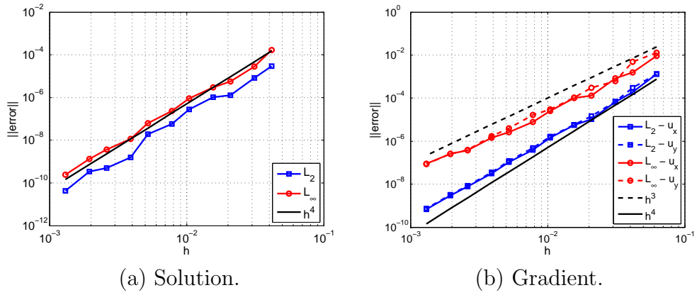
Figure 15: Example 5 - Error behavior of the solution and its gradient in the L_2 and L_\infty norms.
