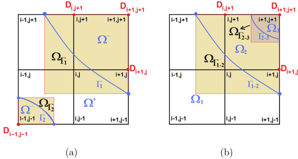
Figure 5: Configuration where multiple \Omega_{\Gamma}^{i,j} are needed in the same stencil. (a) Same interface crossing the stencil multiple times. (b) Distinct interfaces crossing the same stencil.
