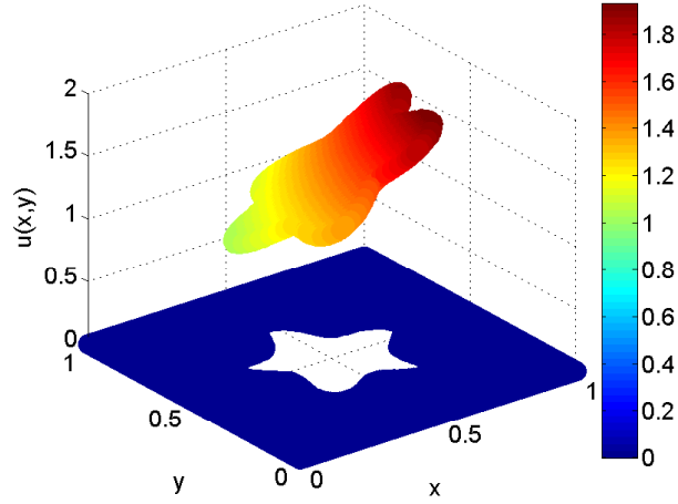
Figure 8: Example 2 - numerical solution with 193 \times 193 nodes.
