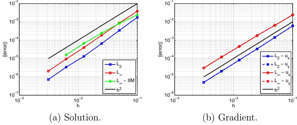
Figure C.6: Example 2 s - Error behavior of the solution and its gradient in the L_2 and L_\infty norms. IIM refers to results obtained with the Immersed Interface Method in [3] (Copyright ©1994 Society for Industrial and Applied Mathematics. Data compiled with permission. All rights reserved).
