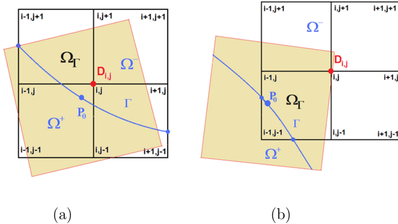
Figure B.4: \Omega_\Gamma^{i,j} as defined by the node-centered approach.
