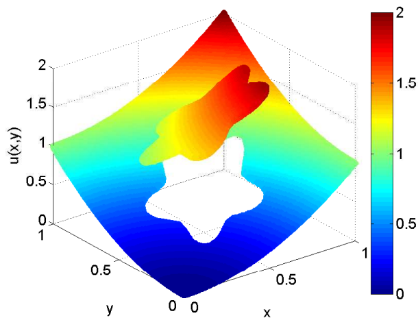
Figure C.3: Example 1_s . Numerical solution with 193 \times 193 nodes, 2^{\text{nd}} order scheme, modified bilinear version.
