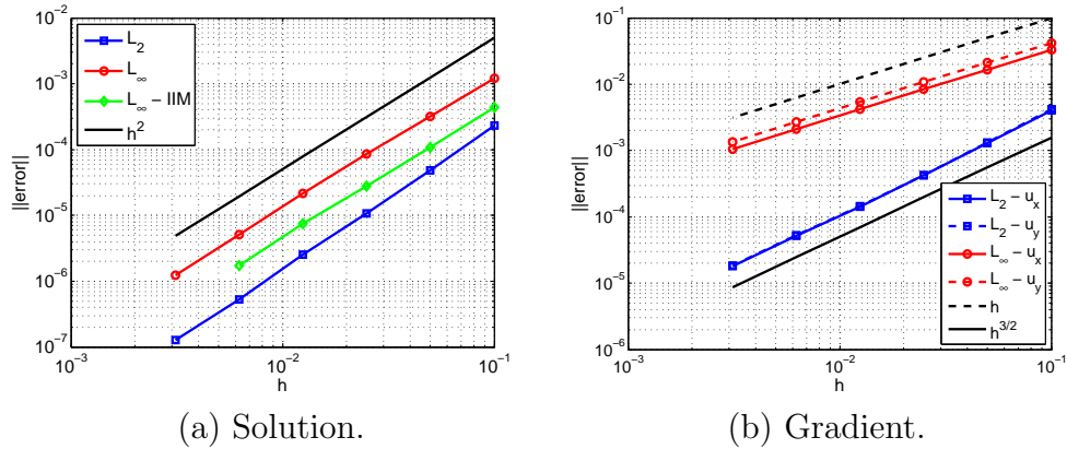
Figure C.8: Example 3_s - Error behavior of the solution and its gradient in the L_2 and L_\infty norms. IIM refers to results obtained with the Immersed Interface Method in [3] (Copyright ©1994 Society for Industrial and Applied Mathematics. Data compiled with permission. All rights reserved).
