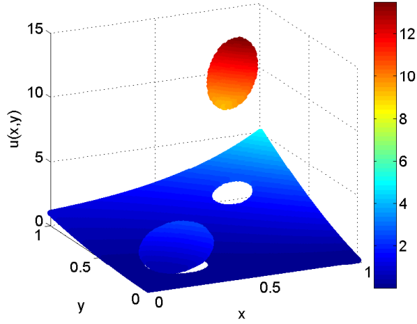
Figure 10: Example 3 - numerical solution with 193 \times 193 nodes.
