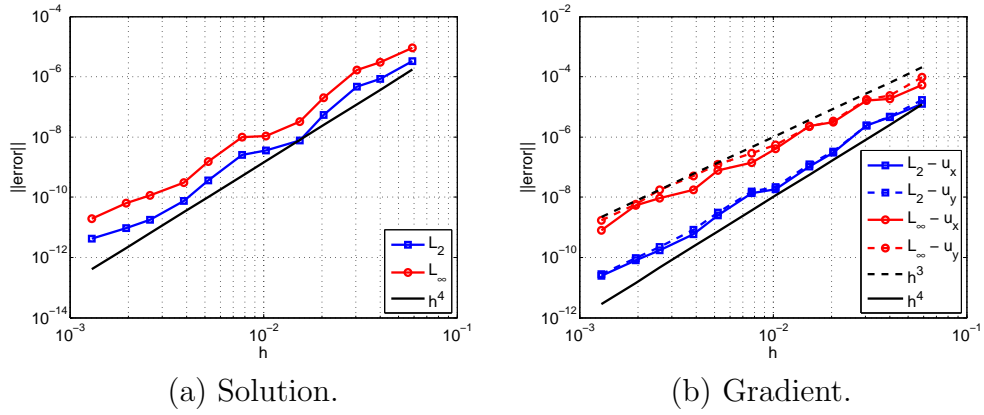
Figure 11: Example 3 - Error behavior of the solution and its gradient in the L_2 and L_\infty norms.
