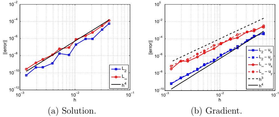
Figure 13: Example 4 - Error behavior of the solution and its gradient in the L_2 and L_\infty norms.
