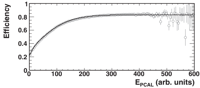
FIG. 4. The event selection efficiency as a function of the E_{\text{PCAL}} centrality variable. Points represent the ratio between the number of events in an E_{\text{PCAL}} bin and the number of events expected for a perfectly efficient detector, obtained using the E_{\text{ring}} efficiency function (see text for details). The black line is a smooth fit to the points.
