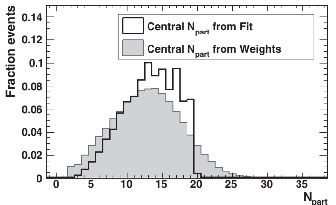
FIG. 7. The N_{\text{part}} distribution in the 0%–20% central E_{\text{PCAL}} bin found using the N_{\text{part}} vs E_{\text{ring}} fit method (open histogram) compared to that from the weighting method (gray histogram). Each distribution is (independently) normalized.
