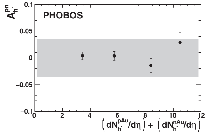
FIG. 18. The asymmetry of negative hadrons between p + Au and n + Au collisions at \langle \eta \rangle = 0.8 as a function of centrality. The gray band shows the systematic uncertainty in the overall scale of the ratio.
