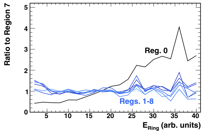
FIG. 9. (Color online) The ratio of the E_{\text{ring}} distribution for events in each region of Fig. 8 to that of region 7, which is partially under the proton peak. The color of the lines follows the same scheme as used in Fig. 8. Region 0, in which no energy is deposited into the d-PCAL, shows a bias toward higher values of E_{\text{ring}} , which is associated with more central collisions.
