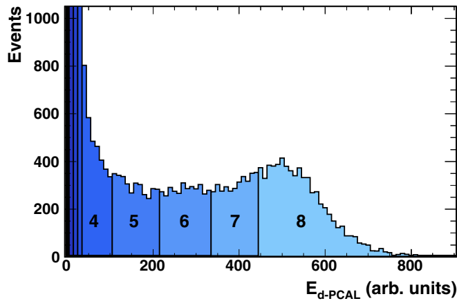
FIG. 8. (Color online) Regions used to study the characteristics of events with different total charge deposited in the d-PCAL. Region 0 is the black colored bin located at the lowest detected E_{d\text{-PCAL}} signal.
