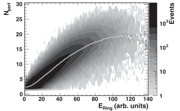
FIG. 6. N_{\text{part}} dependence on E_{\text{ring}} in the MC. The white line shows the fit to the mean N_{\text{part}} in each E_{\text{ring}} bin.
