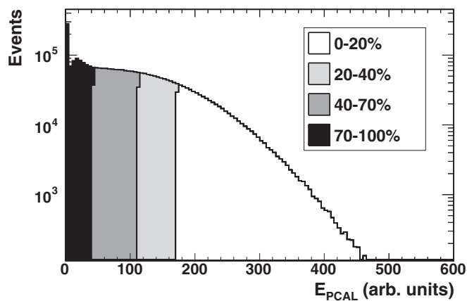
FIG. 5. The centrality bins obtained using the known E_{\text{ring}} efficiency. Each slice of the histogram shows the distribution of E_{\text{PCAL}} within the specified fractional cross-section bin. The kinks in the shaded histograms arise from the edge of a fractional cross section bin falling inside a histogram bin.
