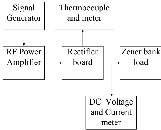
Figure 19. Block diagram of the experimental setup for the diode performance evaluation.
