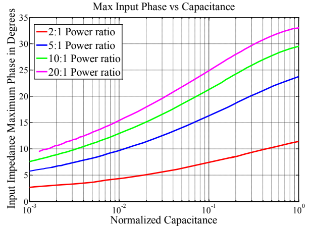
Figure 3. Worst-case phase angle magnitude across the specified operating conditions vs. normalized capacitance for different power ranges ratios ( P_{o,max}:P_{o,min} ).
