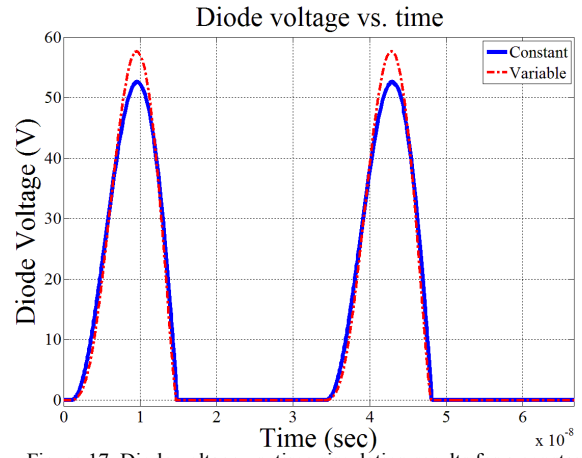
Figure 17. Diode voltage vs. time simulation results for a constant capacitance and for a variable capacitance. For the variable-capacitance case, the range of the diode capacitance is 210 to 19 pF according to instantaneous voltage, while the capacitance for constant-capacitance case is 47 pF. The external capacitance is 86 pF. At higher instantaneous voltage, the variable capacitance is lower and thus the reverse voltage peaks higher.
