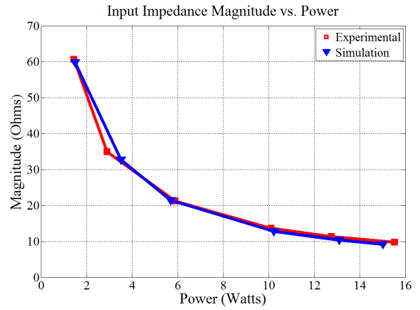
Figure 13. Input impedance magnitude vs. output power for the high-capacitance rectifier circuit described in Table II. The red curve is the measured experimental data and the blue curve is the simulation data.
