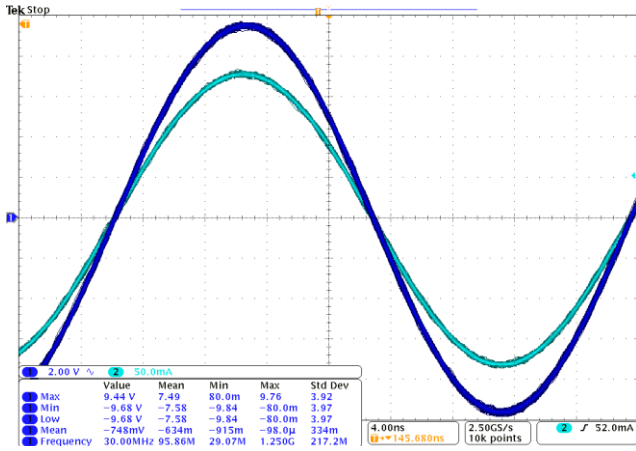
Figure 11. Calibration circuit voltage (dark blue) and current (light blue) waveforms. The oscilloscope is calibrated so that the waveforms are in phase with a 50 \Omega load at 30 MHz.
