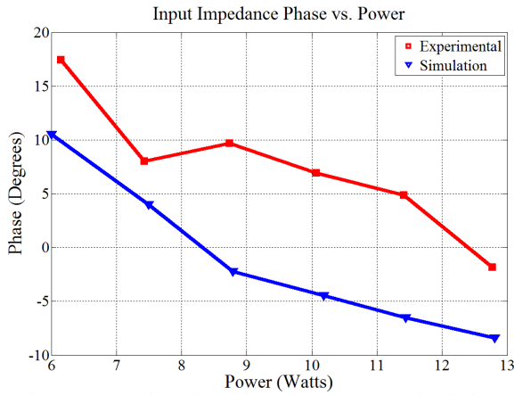
Figure 15. Input impedance phase vs. output power for the low-capacitance rectifier circuit described in Table III. The red curve is the measured experimental data and the blue curve is the simulation data.
