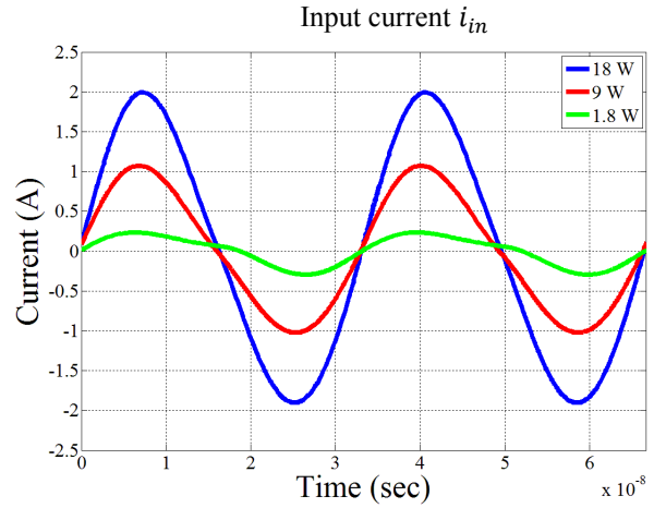
Figure 7. SPICE simulation results. Time-domain simulation of ac input current at 18 W, 9 W and 1.8 W of output power.
