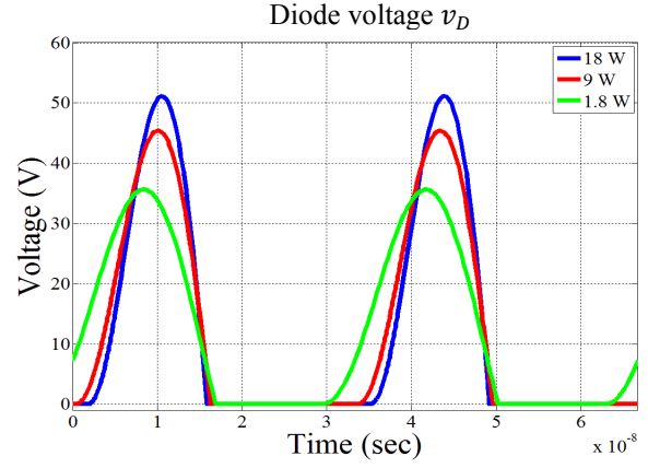
Figure 6. SPICE simulation results. Time-domain simulation of the diode voltage at 18 W, 9 W and 1.8 W of output power.
