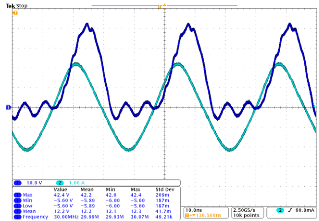
Figure 14. Diode voltage (dark blue) and input current (light blue) at full power, 15.53 W for the circuit of Fig. 10 and values in Table II. The peak diode voltage is 42 V.
