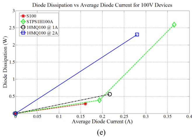
Figure 20. Diode testing results at 30 MHz. Diode dissipation vs. average current for class E rectification into a dc output voltage of 0.2 times the diode rated voltage. The parameters of the rectifiers are listed in Table V. From top to bottom: (a) 40 V, 1-2 A; (b) 60 V, 1A, (c) 2A, and (d) 3 A; and (e) 100 V, 1-2 A.
