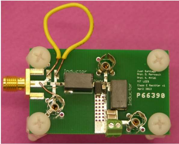
Figure 10. Class E resonant rectifier rated for 12 W, 12 V output voltage and 30 MHz switching frequency.
