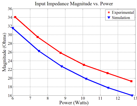
Figure 16. Input impedance magnitude vs. output power for the low-capacitance rectifier circuit described in Table III. The red curve is the measured experimental data and the blue curve is the simulation data.
