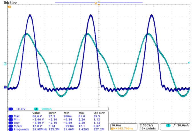
Figure 18. Diode voltage (dark blue) and input current (light blue) at full power, 12.77 W for the circuit of Fig. 3.1 and values in Table III. The peak diode voltage is 60.6 V.
