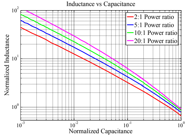
Figure 5. Normalized inductance vs. normalized capacitance for different power ranges ratios ( P_{o,max}:P_{o,min} ).
