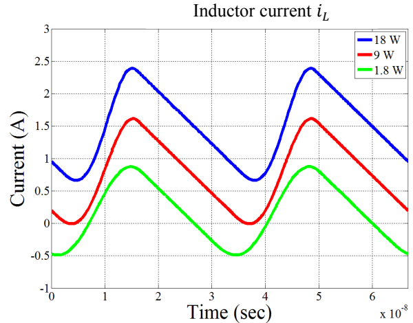
Figure 8. SPICE simulation results. Time-domain simulation of inductor L_r current at 18 W, 9 W and 1.8 W of output power.
