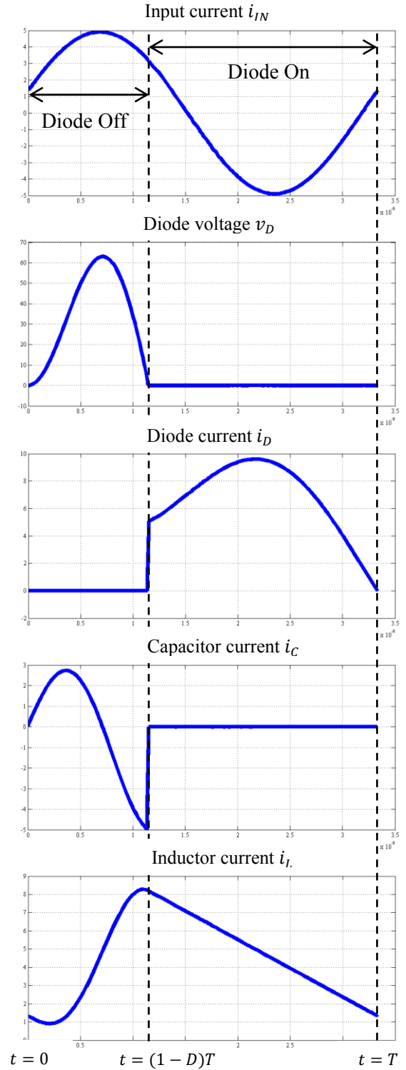
Figure 2. Class E resonant rectifier waveforms; from the top: (a) ac input current through L_S , (b) diode voltage, (c) diode current, (d) capacitor current, and (e) inductor L_r current.
