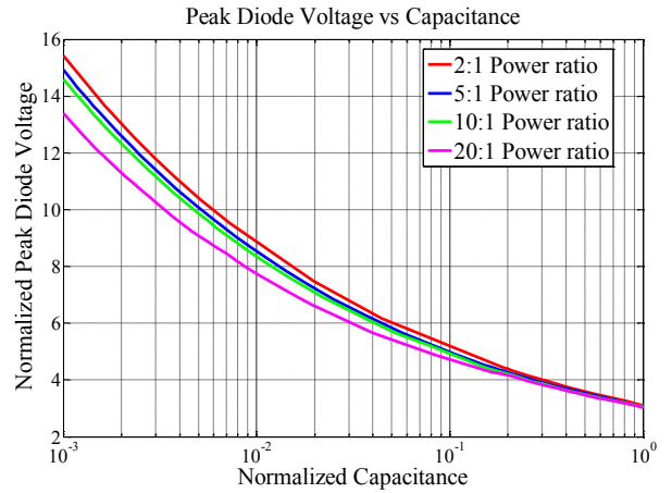
Figure 4. Maximum normalized peak diode voltage vs. normalized capacitance for different power range ratios ( P_{o,max}:P_{o,min} ).
