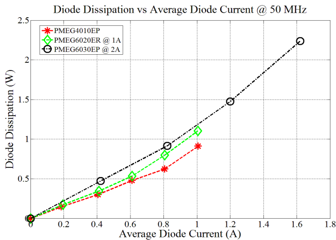
Figure 21. Diode testing results at 50 MHz. Diode dissipation vs. average diode current for class E resonant rectification into a dc output voltage of 0.2 times the diode rated voltage. The parameters of the rectifiers are listed in Table VI.
