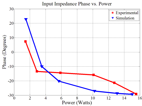
Figure 12. Input impedance phase vs. output power for the high-capacitance rectifier circuit described in Table II. The red curve is the measured experimental data and the blue curve is the simulation data. The maximum absolute phase magnitude over the specified power range is 30°.
