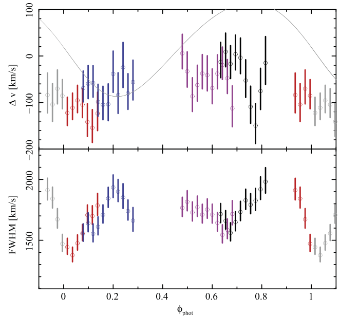
Figure 9. Mean emission line Doppler velocity (top, points with error bars), primary radial velocity (top, sinusoidal curve), and mean line width for Ne x (bottom) derived by fitting spectra in phase bins with an APEC template, allowing the Doppler shift, line width, and normalization to vary freely. Data from the individual Chandra observations are differentiated with colors. Error bars ( 1\sigma ) are correlated over several bins since a running average was used over 3–10 ks bins.
