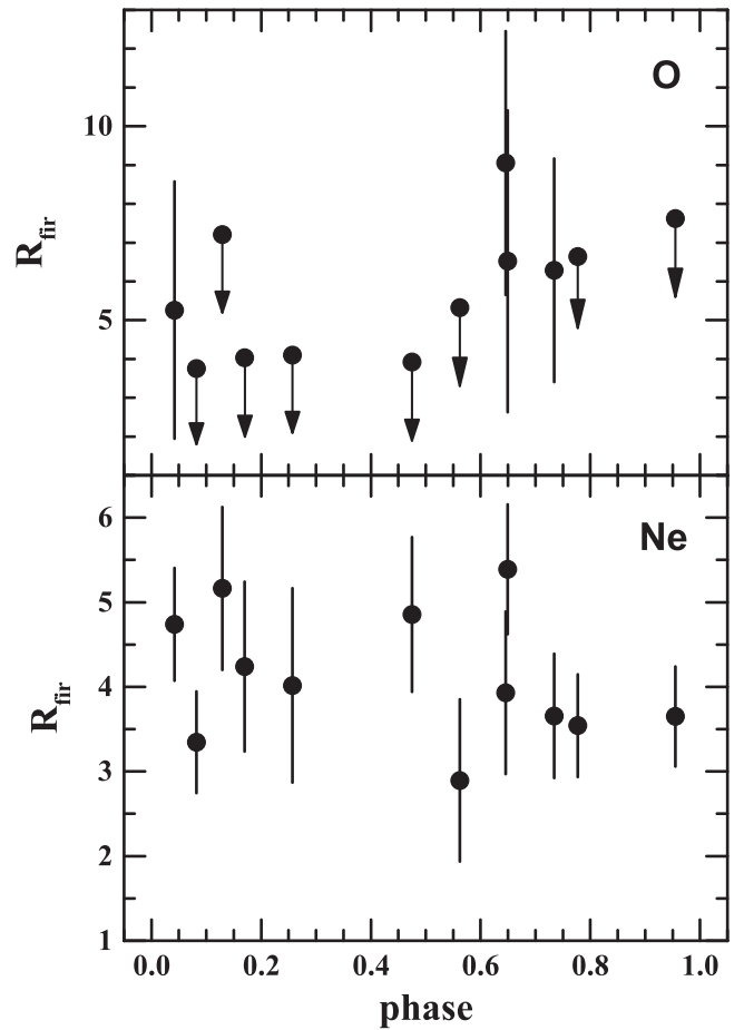
Figure 14. Phase dependence of the derived O and Ne fir -inferred radii ( R_{fir} ) for the 12 time-sliced spectra. Upper and lower limits are shown as arrows. See the text for model details.
