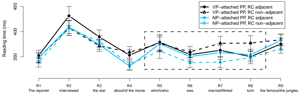
Figure 4: Reading-time results as a function of region and condition for Experiment 2. Onset of the relative clause (first four words) is boxed.
