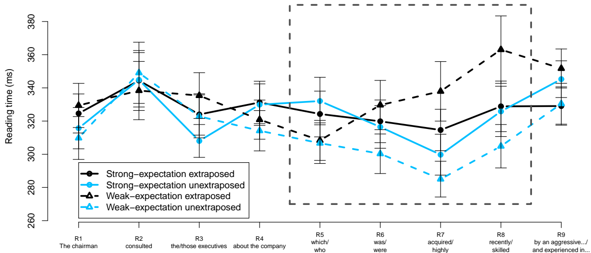
Figure 6: Region-by-region reading times for Experiment 3
