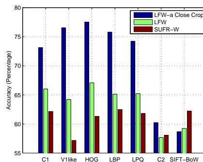
Figure 6: Results on natural image tasks (LFW-a closely cropped, LFW original and SUFR-W). The x axis is type of features. All the results are from our experiments, except that the LFW V1like is from Pinto et al. (2008b) and LFW-a close crop V1like is reported in Pinto et al. (2009). Our attempts to replicate these were stymied by a lack of computational resources
