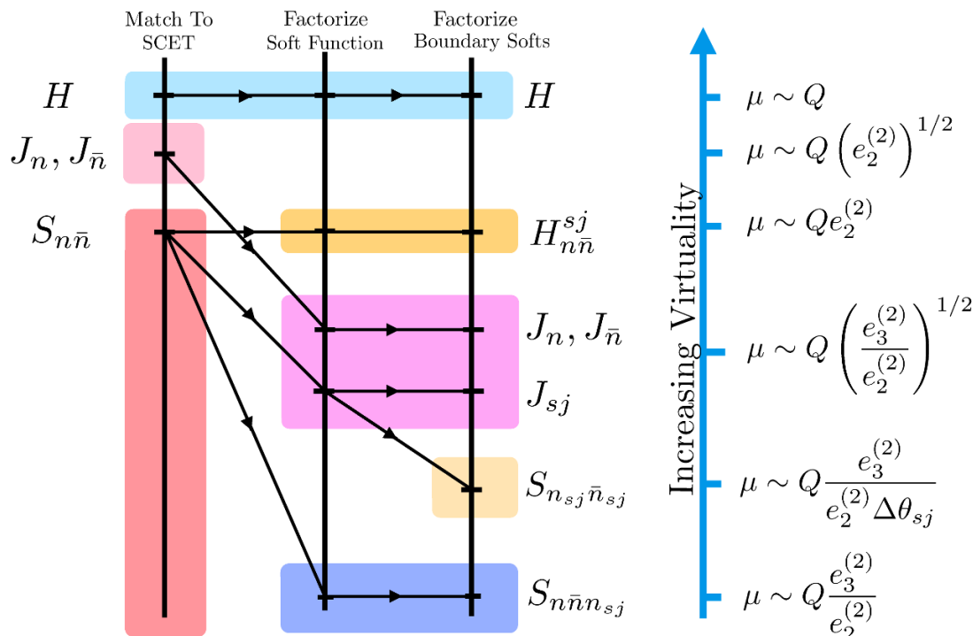
Figure 4. A schematic of the multi-stage matching procedure used to prove the factorization theorem of eq. (3.10) for the soft subjet region of phase space. As discussed in the text, the matching proceeds in three stages: matching to SCET, refactorizing the soft function to describe the soft jet production, and factorizing the boundary soft mode. The canonical scales of the modes in the final factorization theorem are shown on the right, ordered in virtuality. Here we have chosen an angular exponent \alpha = 2 for concreteness.
