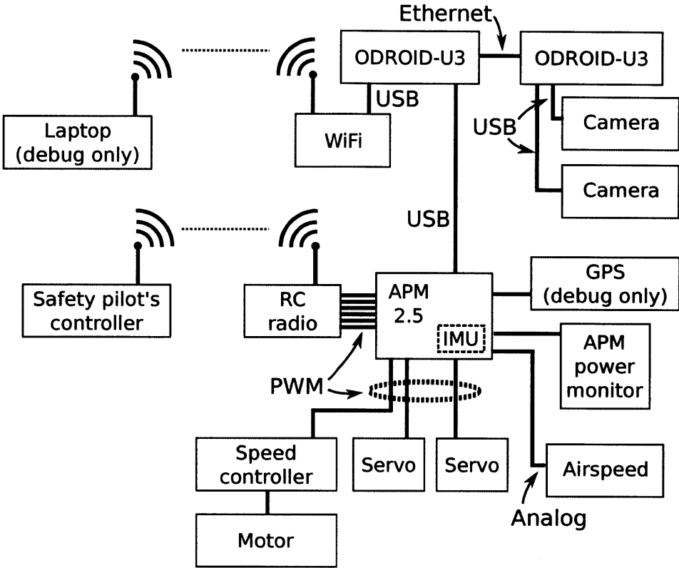
Figure B-1: Information flow diagram for the aircraft.
