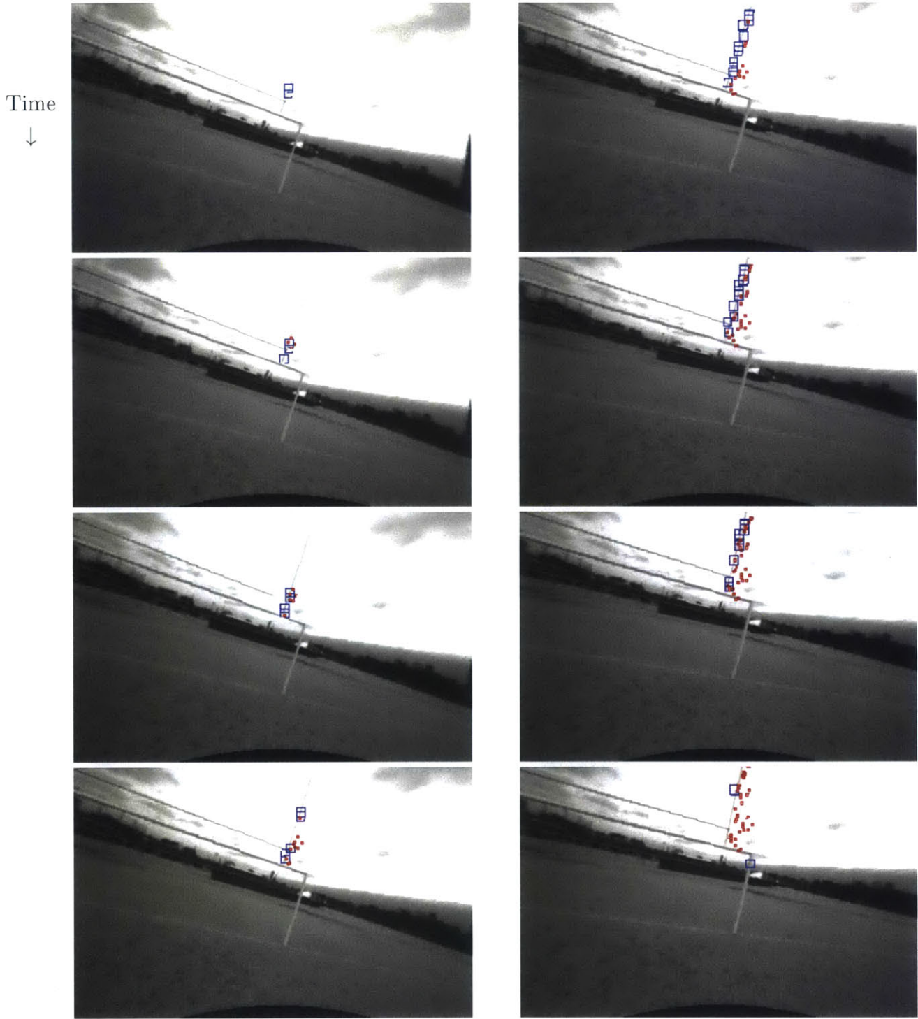
Figure 2-8: Sequence of stills from an obstacle detection. Each image is 0.02 seconds (20ms) after the previous. The entire set captures 0.16 seconds. Here, the fieldgoal is detected in the first frames (blue boxes). Afterwards, the position of those detections is estimated via the state estimator and reprojected back onto the image (red dots).
