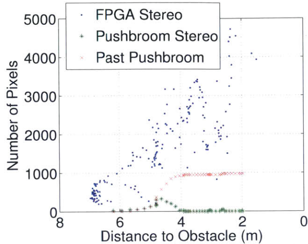
Figure 2-13: Number of pixels detected while flying towards the fieldgoal obstacle. The FPGA system produces an increasing number of detections as the obstacle nears (blue dots), while the pushbroom system only detects the obstacle around the set distance of 4.8 meters (green stars). Past that, pushbroom detections (red crosses) remain in memory for avoidance. Note that the x -axis is reversed allowing time to flow left-to-right.
