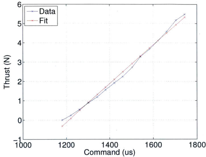
Figure 3-5: Thrust data (blue) with a linear fit (red). The x -axis shows the commanded pulse length in micro-seconds to the speed controller. Clearly the linear model is not valid below 1250 \mu\text{s} because the system can not generate negative thrust.
