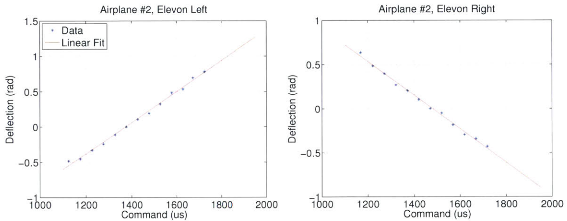
Figure 3-4: Linear model fitting elevon command (PWM pulse length in microseconds) to elevon deflection in radians.
