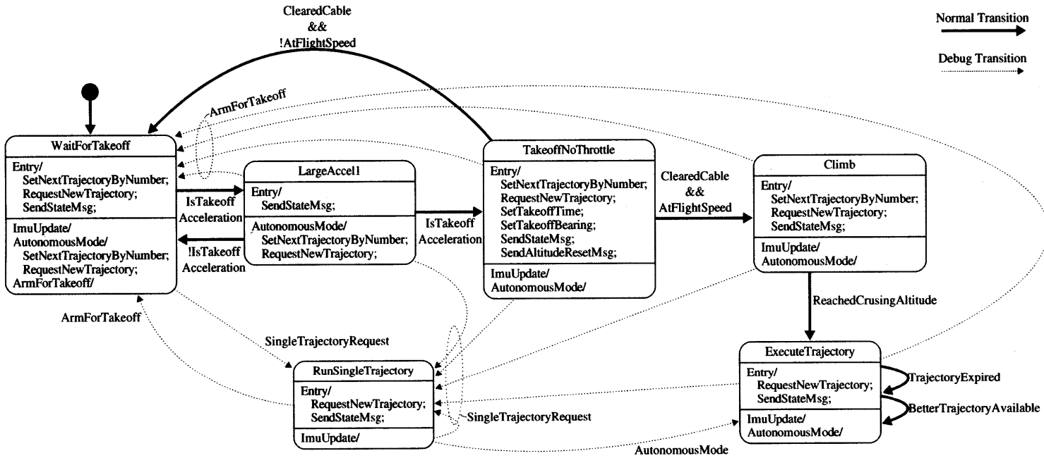
Figure 3-15: State transition diagram. The system starts in the WaitForTakeoff state, transitions through LargeAccel1, TakeoffNoThrottle, and Climb before running the main autonomous state, ExecuteTrajectory. The RunSingleTrajectory state is provided for debugging and testing. Transitions activated by the user for debugging are marked with dotted lines.
