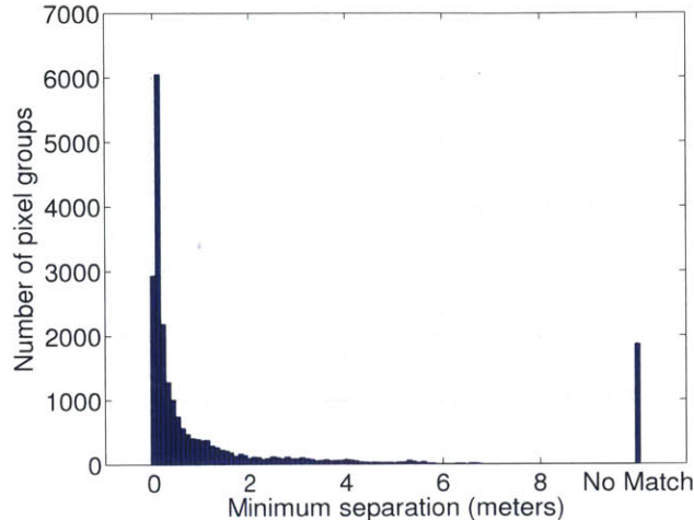
Figure 2-6: Results of the false-positive benchmark described in Figure 2-5 on 23,000+ frames. No Match indicates single-disparity points where there was no matching StereoBM point on the frame. We find that 8.2% of detected pixels fall into this category.
