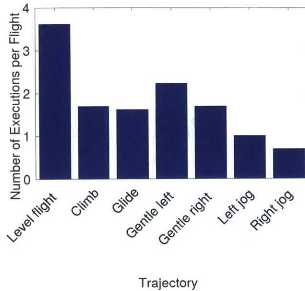
Figure 4-9: Graph of number of times each trajectory in the library was executed per successful flight near trees. Level flight is executed the most, since it is the default trajectory when there are no obstacles.
