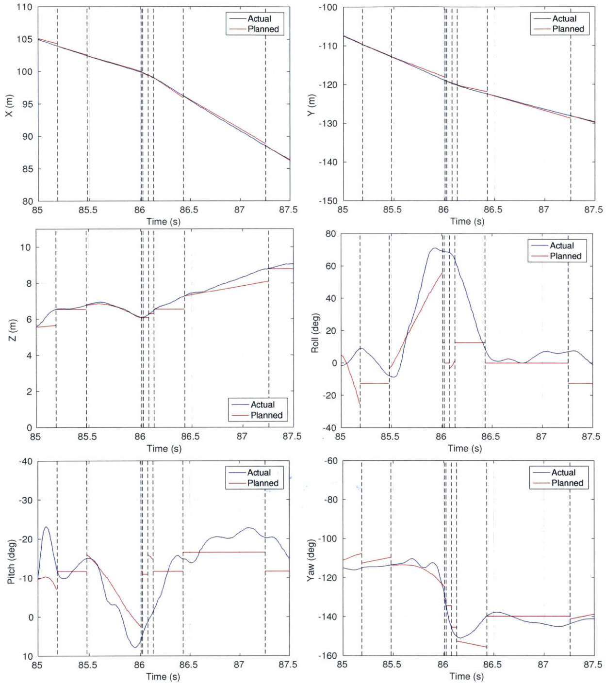
Figure 4-13: Planned and estimated tracking for an obstacle avoidance maneuver. Vertical dashed lines indicate a trajectory change. The first obstacle detection happens at t = 85.15 seconds. Notice the significant turn at t = 86 seconds where the aircraft dramatically alters its yaw angle to avoid an obstacle.
