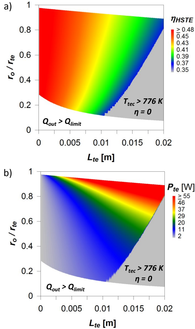
Figure 8. Optimization results for a PbTe HSTE at C = 50 and T_c = 700\text{ K} showing a) system efficiency and b) TE power. An increase in TE leg length ( L_{te} ) decreases efficiency and increases TE power due to a larger TE thermal gradient. As the TE leg length increases, the maximum operating temperature (776 K) is reached, at which point the performance decreases to zero (gray area). In addition, for small thermosyphon radii (bottom white area), heat pipe limitations (e.g., sonic limit) prohibit operation.
