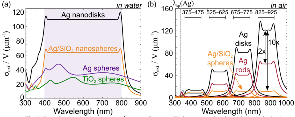
Fig. 1. Broadband extinction cross-section per volume, \sigma_{\text{ext}}/V , by computationally optimized distributions of nanoparticles (solid lines), alongside theoretical limits to broadband response from subwavelength particles (dashed lines). (a) Over visible wavelengths, tailored distributions of silver nanodisks are better than distributions of more common alternatives, including core-shell ( \text{SiO}_2\text{-Ag} ) particles and dielectric ( \text{TiO}_2 ) or metal (Ag) spheres. (b) Across tunable wavelength windows, nanodisks offer significant and increasing enhancements away from silver's bulk plasma wavelength, \lambda_p(\text{Ag}) \approx 324\text{nm} . Detailed theoretical aspect-ratio data is given in Appendix B.
