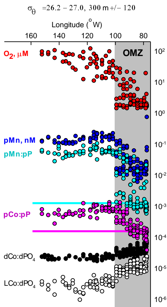
Figure 9. Redox control of Co and Mn scavenging. Within mesopelagic waters ( \sigma_\theta = 26.2 – 27.0 \text{ kg m}^{-3} , mean depth of 300 m), high \text{O}_2 in ventilating water masses results in a sharp redox boundary at the edge of the OMZ (red circles, scale in \mu\text{M} ). Particulate Mn ( p\text{Mn} ) increases across the oxic–anoxic boundary at 100^\circ \text{W} (blue circles, in nM) and implies stabilization of Mn oxides. Both p\text{Mn} : p\text{P} and p\text{Co} : p\text{P} (cyan and pink circles, respectively; units are \text{MM}^{-1} ) increase across the OMZ boundary, exceeding predicted values from remineralization of biogenic material from the surface ocean ( 1.26 \times 10^{-3} mean p\text{Mn} : p\text{P} and 1.57 \times 10^{-4} p\text{Co} : p\text{P} for 0–50 m ( \text{MM}^{-1} ), cyan and pink lines, respectively). Dissolved-phase d\text{Co} : d\text{PO}_4 (black circles) and \text{LCo} : \text{PO}_4 (white circles) also decrease west of the OMZ boundary and show scavenging of d\text{Co} and \text{LCo} in the mesopelagic zone (units are \text{MM}^{-1} ).
