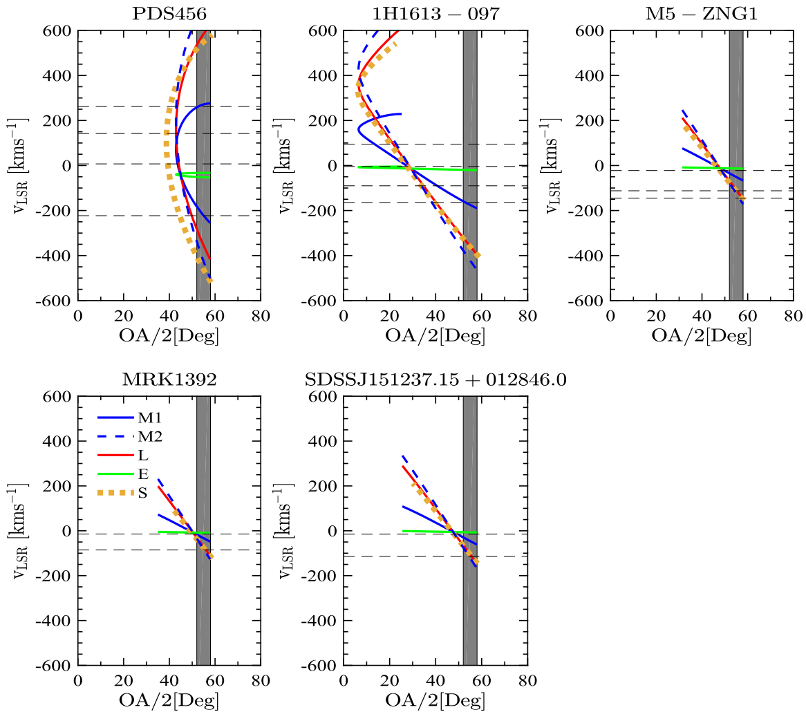
Figure 5. Kinematic models of the Galactic biconical nuclear outflow, some of which can explain the observed absorption-line centroids for the five lines of sight. The centroids of the observed absorption components in the five spectra are shown with horizontal dashed lines. The colored lines correspond to the predicted velocities as a function of distance from the Sun, along that sightline. The colored lines at negative and positive v_{\text{LSR}} correspond to the nearside and the far side of the outflow bicone, respectively. v_{\text{LSR}} \approx 0 corresponds to a distance directly above the GC. The gray band shows the opening angle range that matches the X-ray bicone. If a horizontal dashed line intersects a solid line (model prediction) to the left of the dashed band, the model predicts the kinematics of the observed absorption component along that line of sight. Models M1 and M2 are momentum driven models with launch velocities of \approx 1000 and 1300 \text{ km s}^{-1} , respectively. Model E is the constant energy, and model L is the constant luminosity model, respectively. Model S is a momentum driven model with a launch velocity \approx 1000 \text{ km s}^{-1} from a circular zone of radius 200 \text{ pc} around the GC.
