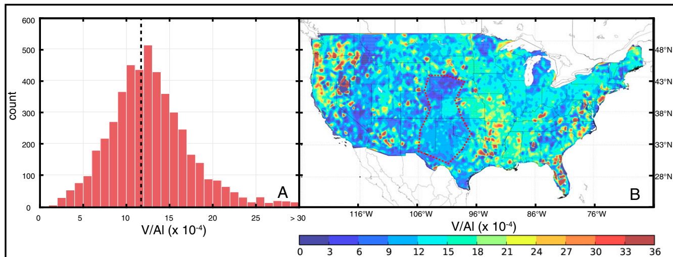
Fig. 1. V/Al ratios of topsoils (0–5 cm depth) across the continental United States. (A) Variation in V/Al ratios from (9). The mean V/Al ratio is 13.28 \pm 12.76 (2 SD), whereas the crustal average of Zhang et al. (1) (11.9) is shown by the dashed line. (B) V/Al ratios of topsoils across the United States. Dashed area represents an area of \sim 816,200 km 2 with a mean V/Al ratio of 10.1. Data are from ref. 9.
