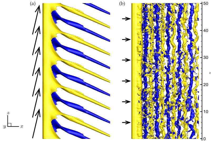
Figure 1. Instantaneous iso-surfaces of the spanwise vorticity in the (a) inclined ( Re = 500 , \omega_{zn} = \pm 0.48 ) and (b) normal ( Re_n = 500 , \omega_{zn} = \pm 1.73 ) fixed rigid cylinder configurations. Arrows represent the oncoming flow. Part of the computational domain is shown.
