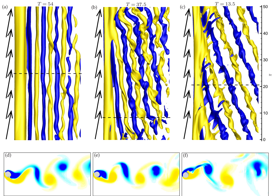
Figure 5. Instantaneous (a-c) iso-surfaces ( \omega_{zn} = \pm 0.58 ) and (d-f) iso-contours in the (x, y) plane ( \omega_{zn} \in [-1.04, 1.04] ) of the spanwise vorticity in the inclined cylinder configuration, for (a,d) T = 54 , (b,e) T = 37.5 and (c,f) T = 13.5 . In (a-c), arrows represent the oncoming flow and the spanwise locations selected in (d-f) are indicated by dashed lines. Part of the computational domain is shown.
