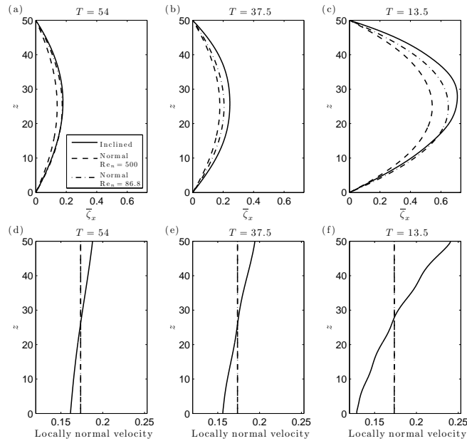
Figure 2. (a-c) Mean in-line displacement of the cylinder and (d-f) inflow velocity component locally normal to the cylinder, along the span, for (a,d) T = 54 , (b,e) T = 37.5 and (c,f) T = 13.5 .
