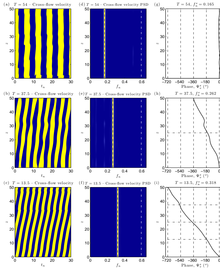
Figure 6. (a-c) Selected time series of the cross-flow component of flow velocity 10D downstream of the inclined cylinder (positive/negative values in yellow/blue) and associated (d-f) PSD and (g-i) unwrapped spatial phase, along the span, for (a,d,g) T = 54 , (b,e,h) T = 37.5 and (c,f,i) T = 13.5 . In (d-f), the PSD is normalized by the magnitude of the largest peak at each spanwise location and the colorbar levels range from 0 (blue) to 1 (yellow); the cross-flow vibration frequency is indicated by a black dashed line and the vortex shedding frequency observed in the absence of structural oscillation by a white dashed-dotted line. In (h,i) dashed-dotted lines denote the minima of the cross-flow vibration envelope.
