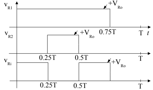
Figure 10: Voltage waveforms at the rectifier input during mode 2.
