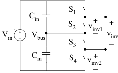
Figure 1: Stacked bridge inverter with input voltage V_{in} and output voltage v_{inv} .
