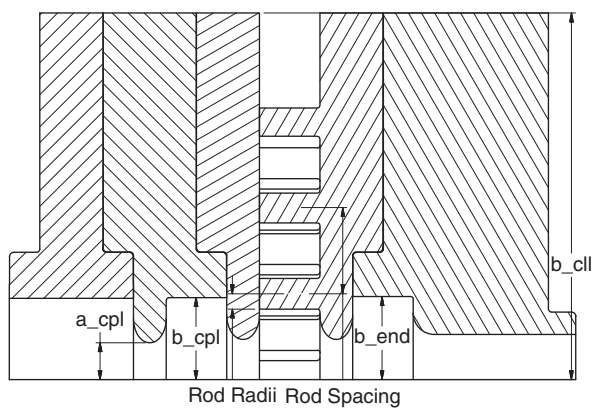
FIG. 3. Axisymmetric views of the assembly drawing of the 17.1 GHz PBG structure showing the tuning parameters for the structure.
