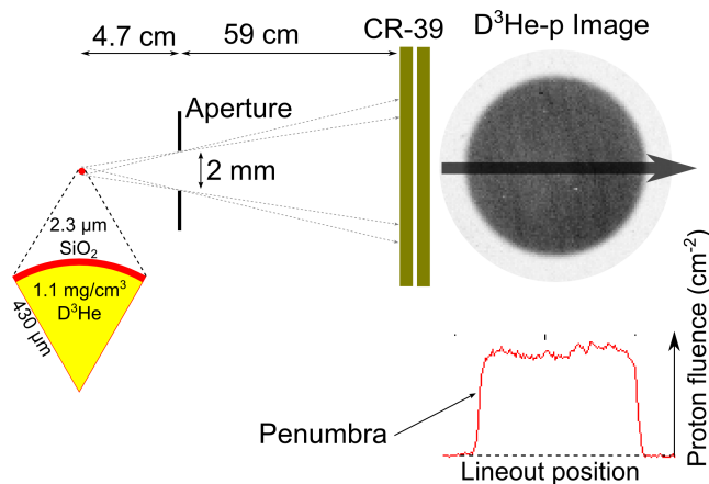
FIG. 2. (Color online) Experimental setup for penumbral fusion burn imaging using the Proton Core Imaging System (PCIS), for an implosion with 1.1 \text{ mg/cm}^3 \text{D}^3\text{He} . DD-p and \text{D}^3\text{He-p} are detected on separate pieces of CR-39, though only a \text{D}^3\text{He-p} image is shown. The penumbra are analyzed to infer profiles of proton emission. While in this diagram a horizontal lineout is depicted, in analysis the penumbra is azimuthally averaged around the image and is much smoother than what is shown here.
