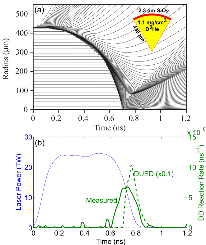
FIG. 4. (Color online) (a) Lagrangian mass-element trajectories and DD fusion reaction rate per unit volume in 1D DUED simulations of an implosion with 1.1 \text{ mg/cm}^3 \text{ D}^3\text{He} , originally presented in Ref. [6]. (b) The DUED-predicted DD burn history (green dashed) compared to the measured burn history (green solid) and the incident laser power (blue solid). (a) is reproduced with permission from Phys. Rev. Lett. 112 , 185001 (2014).
