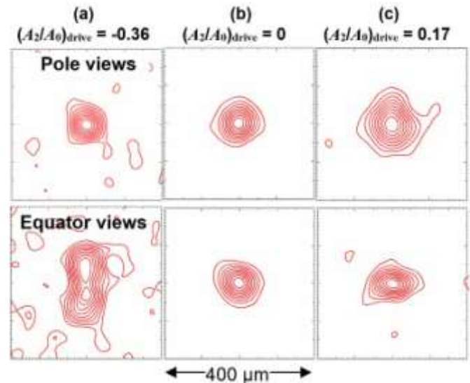
FIG. 3 (color online). Contour plots of burn images of spherical capsules show that asymmetries in the burn result in a predictable way from asymmetries in the drive. The contours are linearly spaced at 10%, 20%, ..., 90% of the peak value. The data come from (a) OMEGA shots 35172 and 35173 (summed), (b) 36020 and (c) 35174. As discussed in the Appendix, the statistics-constrained spatial resolutions of these burn distributions are 20 \mu\text{m} for (b) and (c) but 35 \mu\text{m} for (a), because of the very low proton yield for this case. The noise structures outside the main burn region indicate the spatial scale and amplitude of noise-generated spurious structure in the inferred burn distribution.
