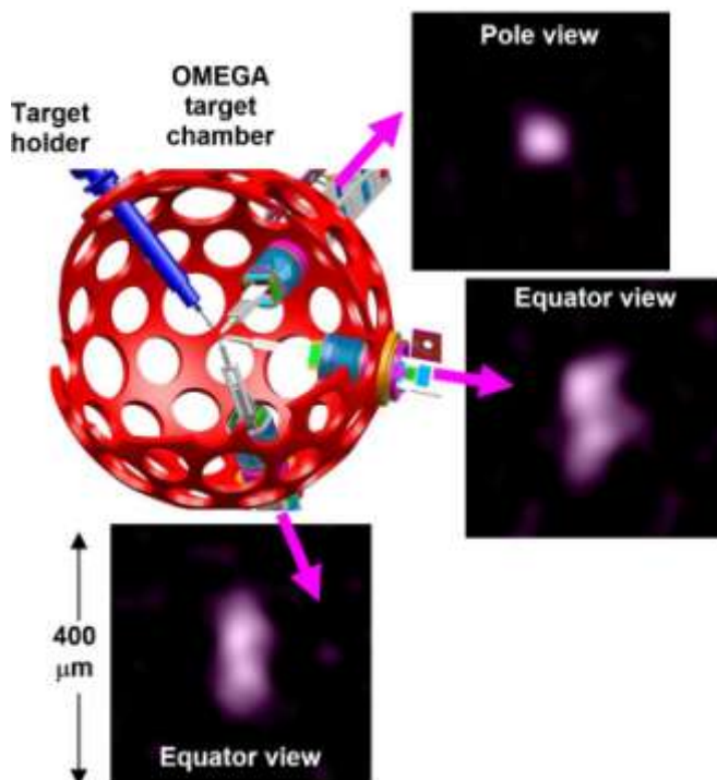
FIG. 1 (Color). Three proton-emission images recorded from orthogonal directions show how asymmetric D^3He burn results from (intentional) drive asymmetry in experiments at OMEGA (lighter color means more D^3He reactions). The target capsule was spheroidal (Fig. 2b). Laser intensity was axially symmetric, and lower than average in the pole directions (see Fig. 2a, curve A_2/A_0 = -0.36 ), resulting in an elongated, or prolate, burn distribution.
