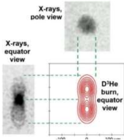
FIG. 4 (color online). X-ray emission images of the shell near peak burn time from OMEGA shot 35173, compared to the inferred distribution of fusion burn from shots 35172 and 35173 with drive asymmetry (A_2/A_0)_{\text{drive}} = -0.36 . The x-ray images have a spatial resolution of about 10\ \mu\text{m} . The original burn images, shown in Figs. 1 and 3a, have a resolution of 35\ \mu\text{m} (because very low yield required serious filtering) so for comparison the burn distribution shown here is an estimate of the true burn distribution derived as discussed in the Appendix. (This estimation process was not necessary for the burn images shown in Fig. 5, which come from a higher-yield shot.)
