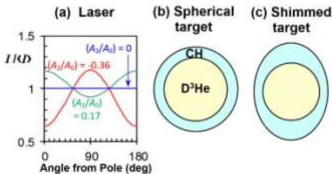
FIG. 2 (color online). Three angular distributions of laser intensity I on target (a), and structures of spherical (b) and shimmed (c) targets. Each intensity distribution is labeled with the ratio of its 2 nd and 0 th Legendre amplitudes. The burn images shown in Fig. 1 resulted from the drive intensity distribution labeled “ (A_2/A_0) = -0.36 ” together with a spherical target capsule (b).
