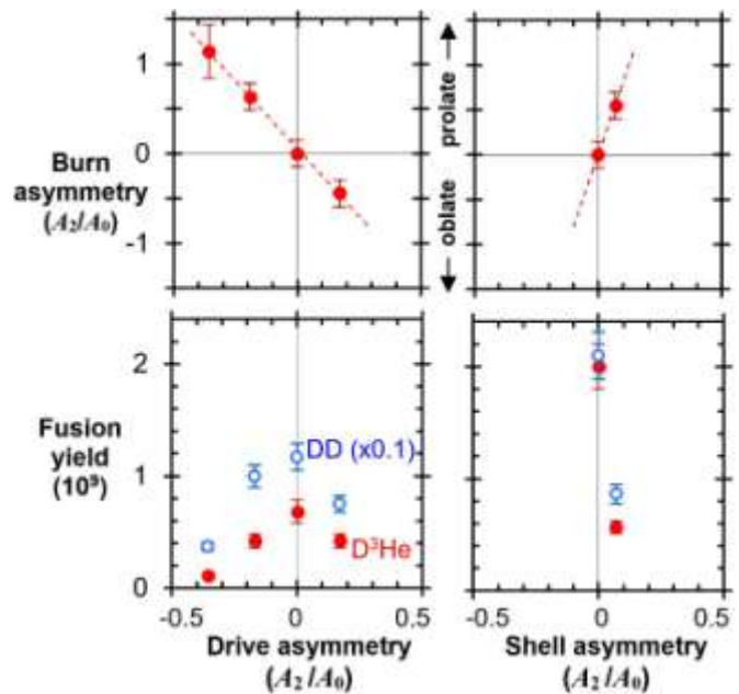
FIG. 6 (color online). Measured dependence of nuclear burn asymmetry (top plots) and fusion yield (bottom plots) on drive asymmetry for spherical capsules (left) and on shell-thickness asymmetry for spherical drive (right). The dashed lines indicate trends, and are not quantitative fits or predicted extrapolations. All yields decrease quickly as the burn region loses spherical symmetry.
