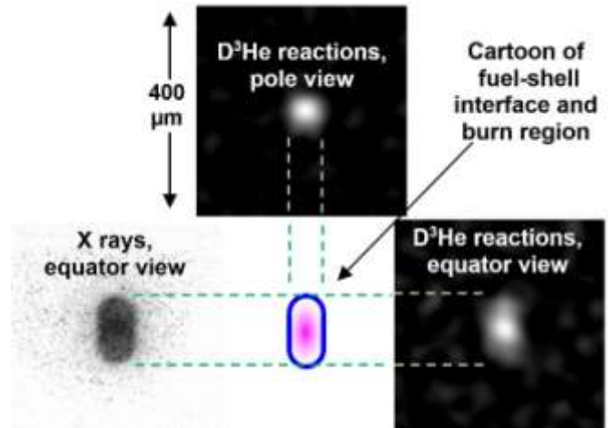
FIG. 5 (color online). Images of the spatial distribution of \text{D}^3\text{He} reactions in the compressed fuel (top and right), and the spatial distribution of 4–5 keV x-rays from the fuel-shell interface (left), at peak burn time for OMEGA shot 40532 utilizing the shimmed target.
