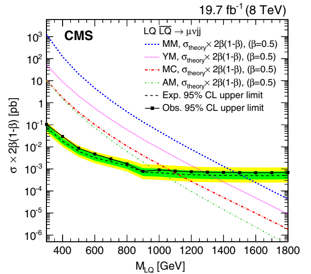
FIG. 14. Frame on top (bottom): the expected and observed upper limits at 95% CL on the vector leptoquark pair production cross section times \beta^2 ( 2\beta(1-\beta) ) as a function of the second generation vector leptoquark mass, obtained with the \mu\mu jj ( \mu\nu jj ) analysis for the four coupling scenarios (MC, YM, MM, and AM). The expected limits and uncertainty bands represent the median expected limits and the 68% and 95% confidence intervals using the MC scenario. Because of the kinematic similarity between the MC scenario and the other coupling scenarios, cross section limits are found to be the same within the uncertainties.
