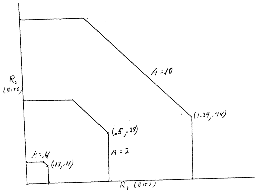
ACHIEVABLE RATE REGION AS FUNCTION OF SIGNAL/NOISE A
