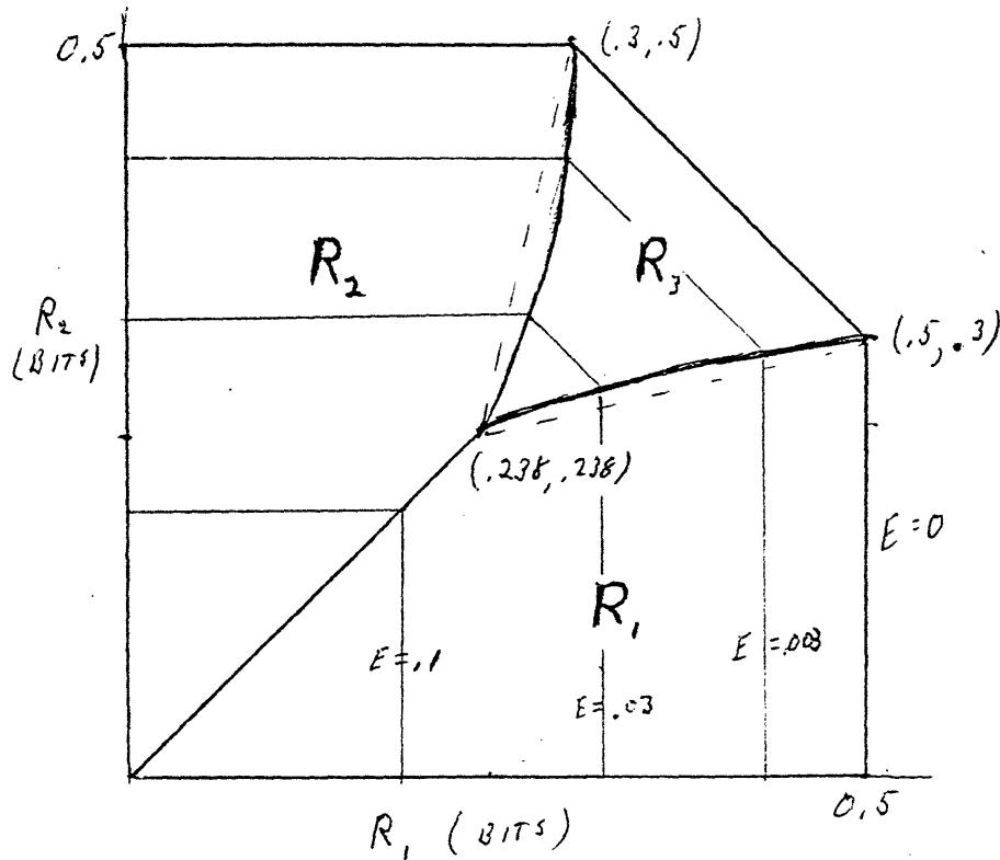
REGIONS R_i WHERE E_{r_i} DOMINATES ERROR BOUND; FOR A=1 .
