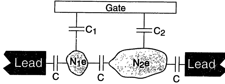
Figure 3-15: Capacitances, as defined by Ruzin.
