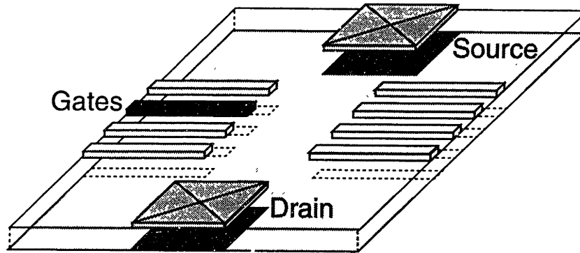
Figure 3-14: Schematic of the double dot structure. The center-to-center distance between tunneling barriers is 200 nm and 400 nm for the two dots. The gate indicated in dark is swept.
