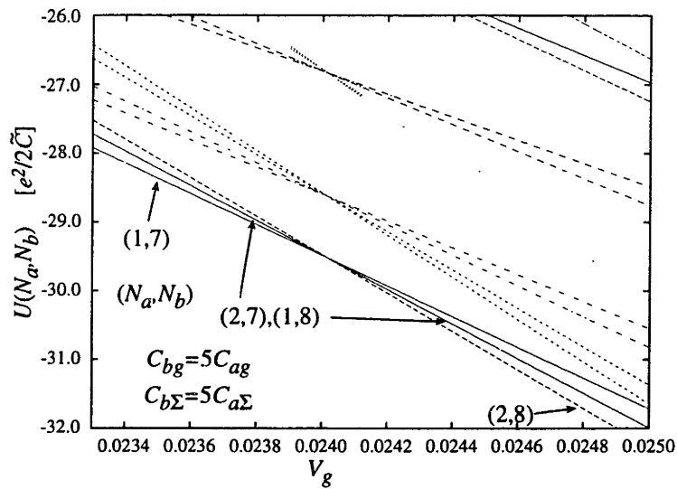
Figure 3-23: Close-up of charging energy as a function of gate voltage for two unequal dots.
