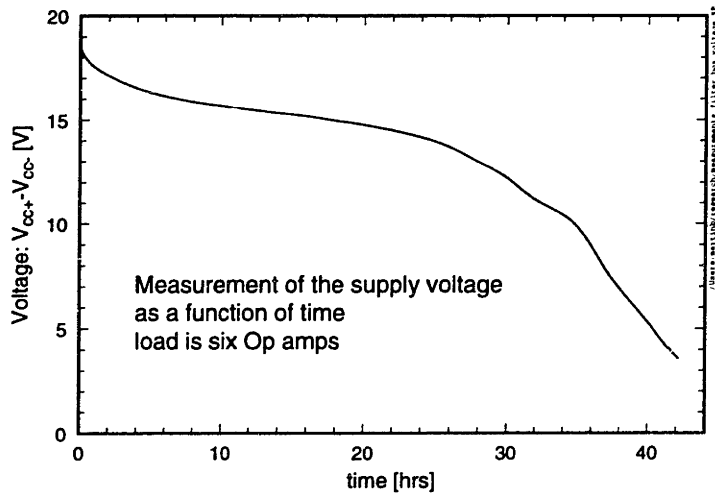
Figure H-5: Supply voltage versus time.
