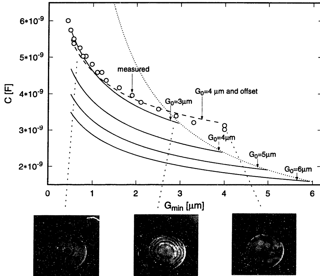
Figure 2-7: Plot of capacitance versus minimum gap. The full lines correspond to theoretical capacitances for different initial gaps between 3 and 6 \mu\text{m} . The measured points are determined by measuring the initial gap and then counting interference fringes. The dashed line is the capacitance for a 4 \mu\text{m} initial gap with an additional offset accounting for uncertainty in C_{\text{mesa}} . The dotted line gives the capacitance of a parallel plate capacitor for comparison. The images on the bottom are photographs of the setup at different values of minimum gap.
