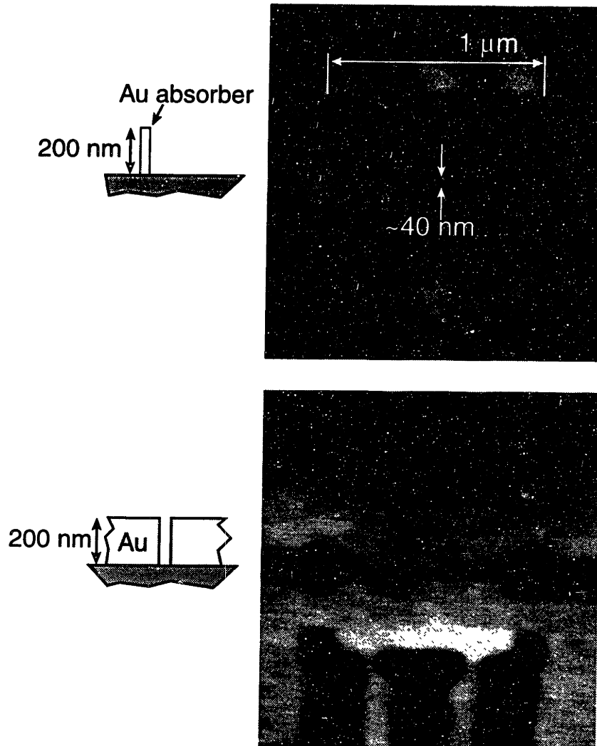
Figure 2-8: Scanning electron micrographs of parent and daughter masks of a pattern containing 40 nm features. The gold absorber is plated to a thickness of 200 nm.
