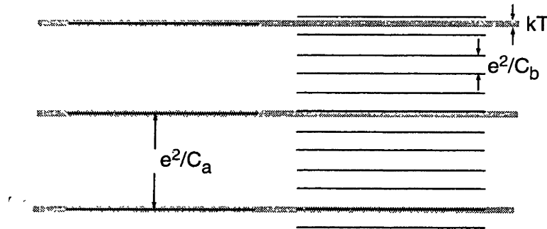
Figure 3-17: Energy ladders for a double dot system. The left ladder shows the smaller dot, the right the larger dot. Note that the two ladders move with different speed when the gate voltage is changed, according to the difference in capacitive lever arms.
