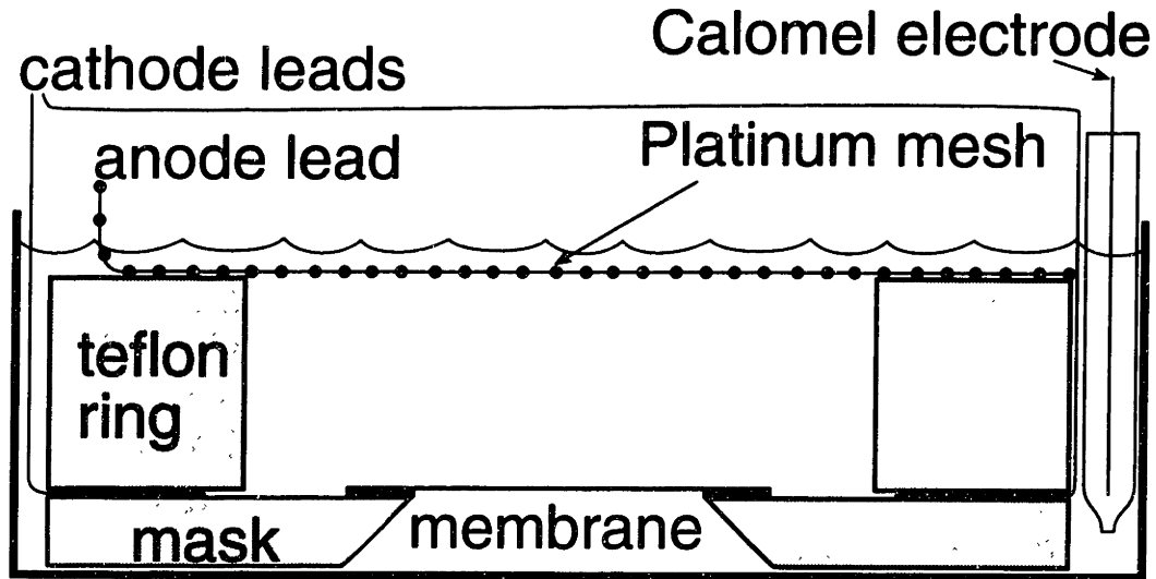
Figure 2-11: Schematic of the fixture used for plating of x-ray masks. A pyrex beaker is used to contain the plating solution, limiting the amount of plating solution to about 250 ml.
