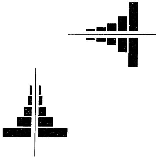
Figure E-6: Proximity effect test structure in the diagnostic pattern.
