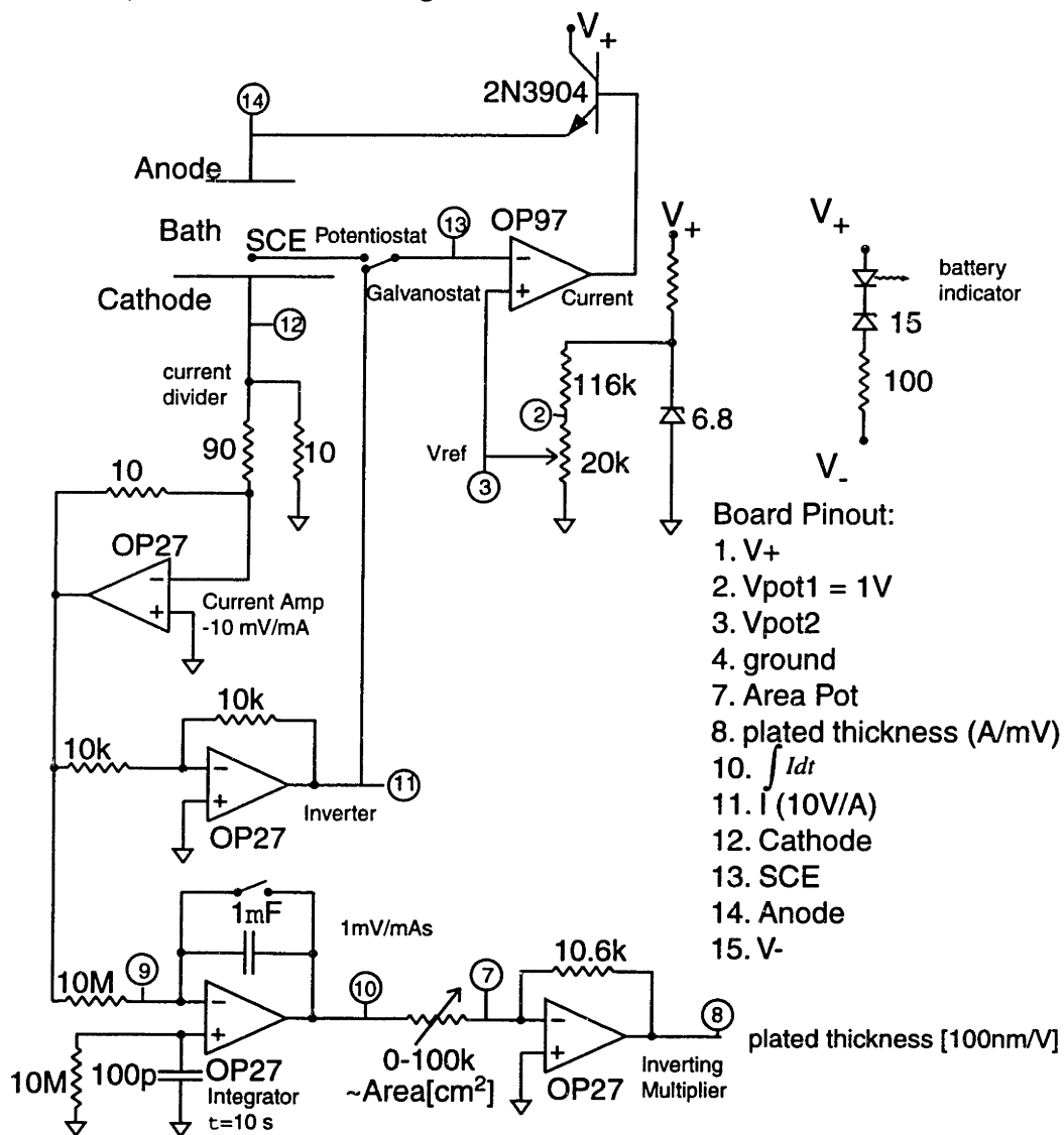
Figure C-1: Schematic circuit diagram of the plating power supply.
