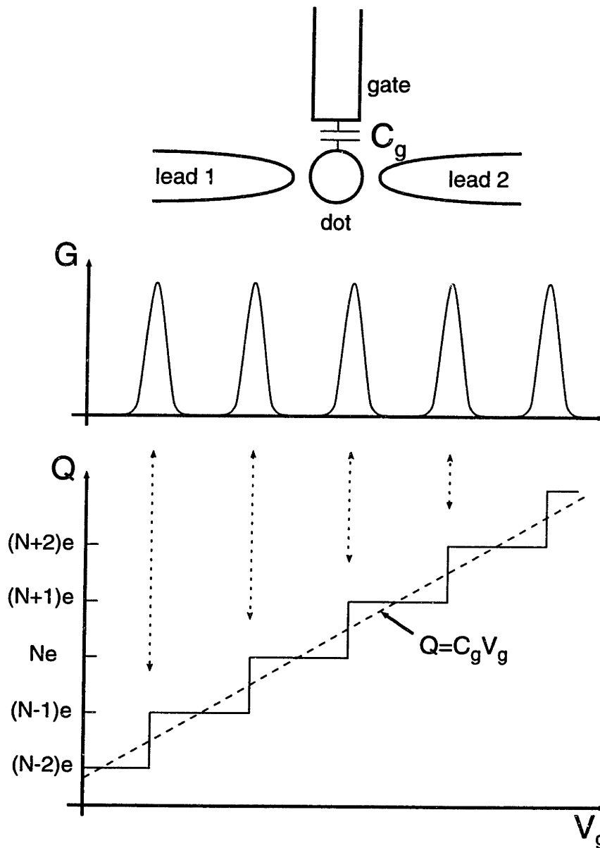
Figure 3-2: Explanation of Coulomb oscillations using the total charge of the dot. After ref. [71].
