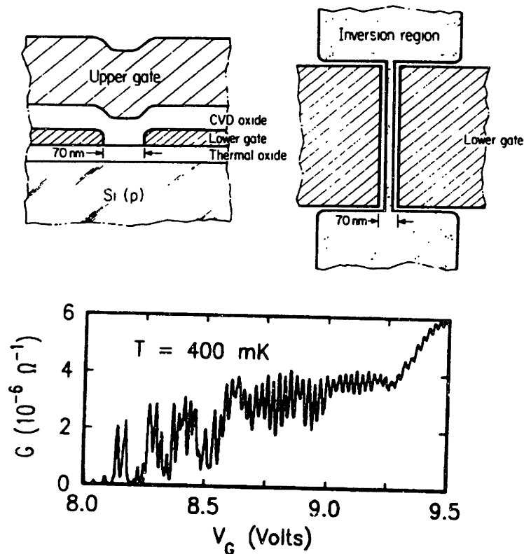
Figure 3-1: Devices in which the discovery of Coulomb blockade in semiconductor devices was made. The bottom gate was used to define a long, diffusive wire in the silicon, while the top gate was used to sweep the chemical potential within the wire. The graph on the bottom shows the conductance of the wire. After ref. [67].
