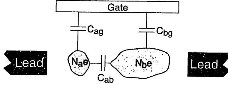
Figure 3-16: Easiest case for coupling of two quantum dots.
