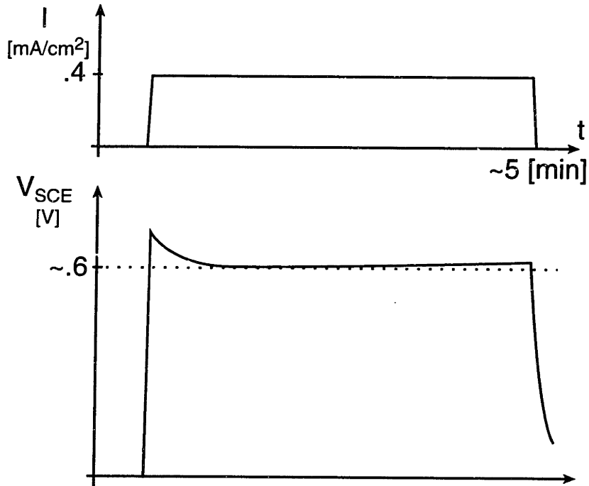
Figure C-2: Qualitative description of the SCE voltage as a function of time and plating current density.
