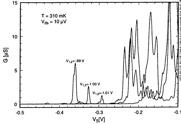
Figure 3-32: Shift of the peak associated with the smaller dot.
