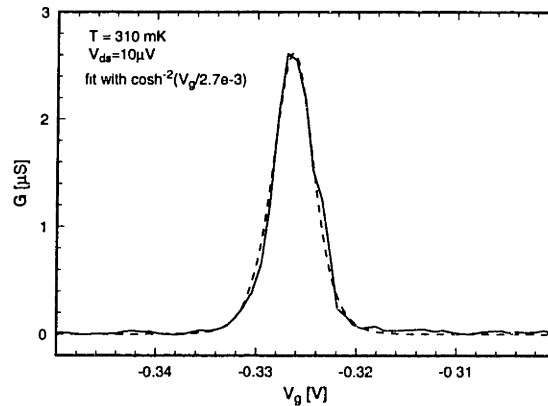
Figure 3-30: Fit of the first conductance peak in the double dot case with the Fermi function.
