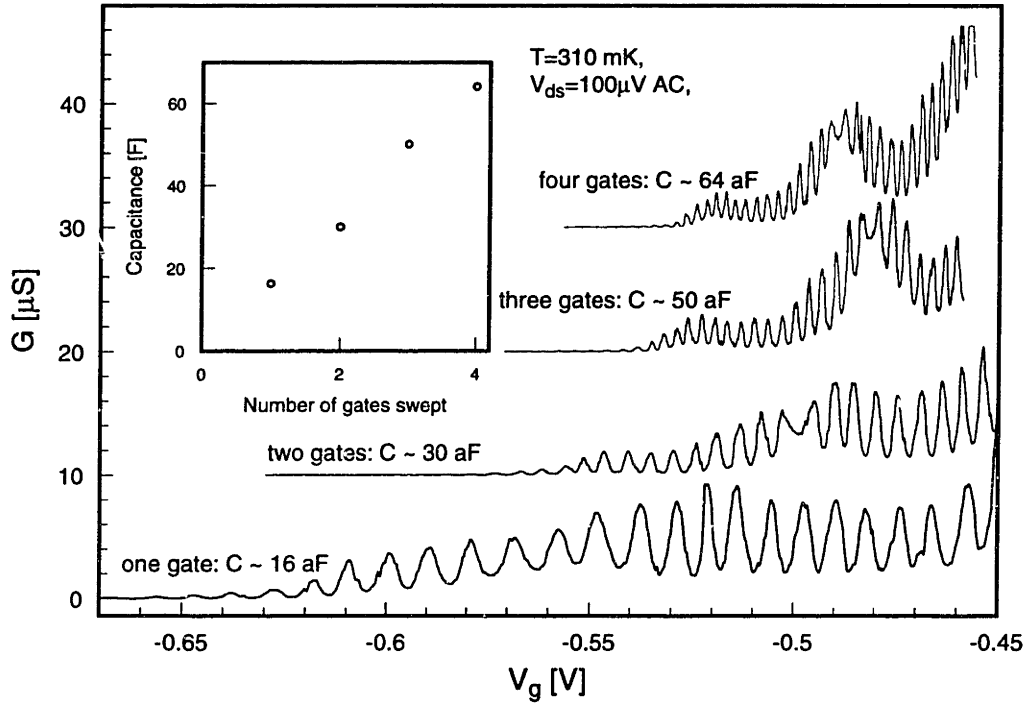
Figure 3-11: Conductance of a 600 nm dot with one, two, three and all four inner gates swept.
