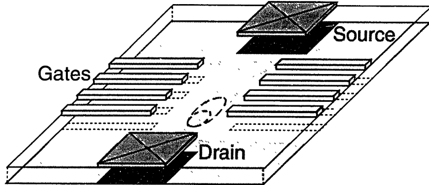
Figure 3-8: Schematic of biasing conditions for different dot sizes. Dots of various sizes can be made by pinching off two pairs of the four consecutive quantum point contacts. Each pair of quantum point contacts has an opening of 300 nm, the distance from one pair to the next is 300 nm. The maximum possible length of the dot is 600 nm.
