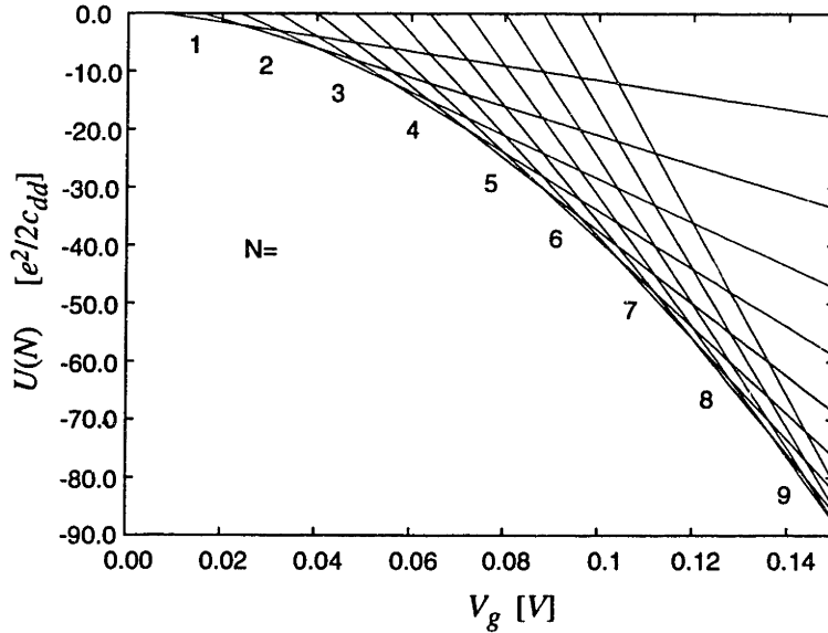
Figure 3-4: Charging Energy of the dot as a function of gate potential for C_{dg} = 10 aF. The system is in the state that minimizes the charging energy. After ref. [77].
