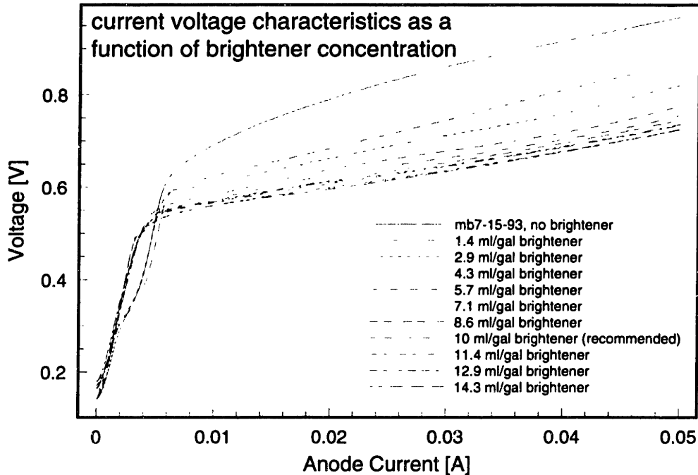
Figure 2-9: Current-voltage-characteristic of a plating bath as a function of brightener concentration. The plot shows the voltage of the cathode with respect to a saturated Calomel electrode. The recommended brightener concentration is 10 ml per gallon. The cathode area in this experiment was about 25\text{ cm}^2 , so that typical current densities used during plating correspond to between 10 and 20 mA in this plot.
