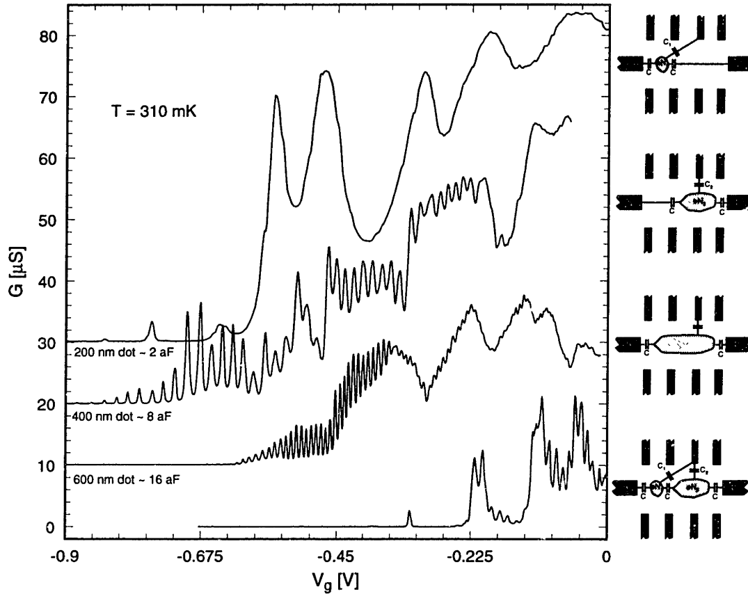
Figure 3-29: Conductance as a function of gate voltage for separate dots of 200, and 400 nm length and a 200 and 400 nm dot in series. For comparison, the conductance for the 600 nm long dot is plotted as well.
