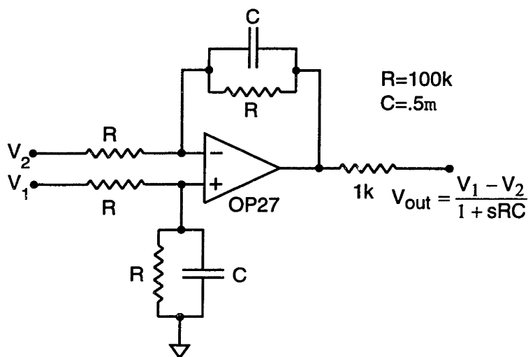
Figure H-2: Circuit diagram of gate filter.
