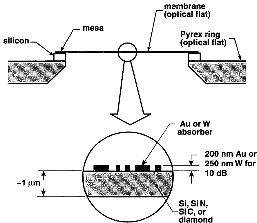
Figure 2-1: Schematic of the mask commonly used for soft x-ray proximity lithography at \lambda=1.3 nm. In this case, the membrane consists of SiN, the absorber of Au. Other materials are possible, as indicated. Courtesy of Bill Chu.
