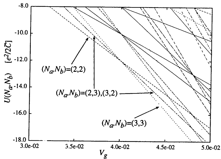
Figure 3-19: Close-up of Fig. 3-18. The energy levels that contribute to current flow are labeled.
