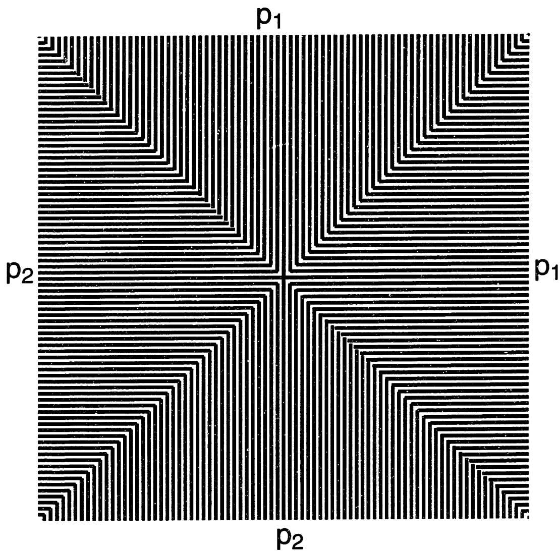
Figure F-1: Example of a Moiré alignment mark. Written with an e-beam, the outer dimension of the alignment mark would be 80\ \mu\text{m} . The horizontal periodicity is 1\ \mu\text{m} , and the vertical is 1.05\ \mu\text{m} in this case.
