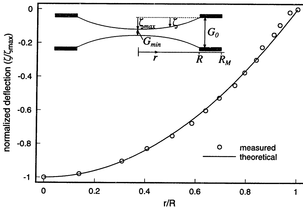
Figure 2-6: Plot of normalized deflection as a function of normalized radius. Measured values are indicated with circles, the line shows the fit using eq. (2.4). The inset shows a schematic of the system, indicating the variables used in the calculations.
