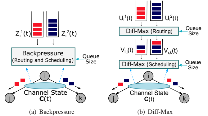
Fig. 1. Example topology consisting of three nodes; i, j, k , and two flows; 1, 2. Note that this small topology is a zoomed part of a large multi-hop wireless network. The source and destination nodes of flows 1 and 2 are not shown in this example, i.e. , nodes i, j, k are intermediate nodes which route and schedule flows 1 and 2. (a) Backpressure: Node i constructs per-flow queues; Z_i^1 and Z_i^2 , and determines the queue backlog differences at time t ; D_{i,j}^s(t) = Z_i^s(t) - Z_j^s(t) , D_{i,k}^s(t) = Z_i^s(t) - Z_k^s(t) , where s \in \{1, 2\} . Based on the differences as well as the channel state of the network, C(t) , backpressure makes joint routing and scheduling decisions. (b) Diff-Max: Node i constructs per-flow queues; U_i^1 and U_i^2 in the network layer, and per-link queue sizes; V_{i,j} and V_{i,k} in the link layer, and makes routing decision based on the queue backlog differences at time t ; \tilde{D}_{i,j}^s(t) = U_i^s(t) - U_j^s(t) - V_{i,j}(t) , \tilde{D}_{i,k}^s(t) = U_i^s(t) - U_k^s(t) - V_{i,k}(t) , where s \in \{1, 2\} . Separately, node i makes the scheduling decision based on V_{i,j}(t) , V_{i,k}(t) , and C(t) .
