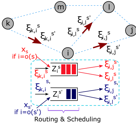
Fig. 3. Backpressure system model in a wireless mesh network. Per-flow queues inside node i are shown in detail. Z_i^s and Z_i^{s'} are the per-flow queues for flows s and s' , respectively. The backpressure routing & scheduling algorithm operates jointly over the per-flow queues.
