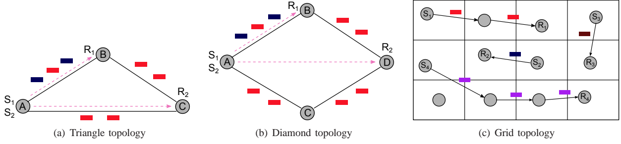
Fig. 5. Topologies used in simulations. (a) Triangle topology. There are two flows between sources; S_1, S_2 and receivers; R_1, R_2 , i.e., from node A to B ( S_1 - R_1 ) and from node A to C ( S_2 - R_2 ). (b) Diamond topology. There are two flows between sources; S_1, S_2 and receivers; R_1, R_2 , i.e., from node A to B ( S_1 - R_1 ) and from node A to D ( S_2 - R_2 ). (c) Grid topology. 12 nodes are randomly placed over 4 \times 3 grid. An example node distribution and possible flows are illustrated in the figure.
