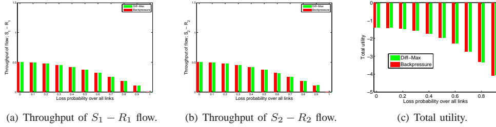
Fig. 7. Numerical results for the triangle topology shown in Fig. 5(a). The loss is over all links. (a) Throughput of S_1 - R_1 flow. (b) Throughput of S_2 - R_2 flow. (c) Total utility.
