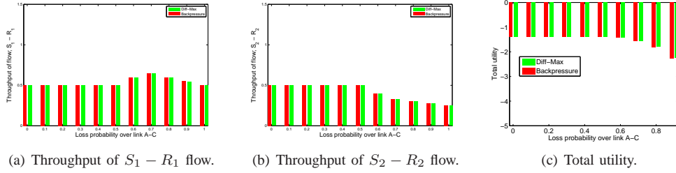
Fig. 6. Numerical results for the triangle topology shown in Fig. 5(a). The loss is over link A - C . (a) Throughput of S_1 - R_1 flow. (b) Throughput of S_2 - R_2 flow. (c) Total utility.
