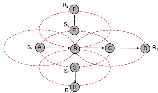
Fig. 15. A topology that we consider for the flow in the middle problem. There are three flows; Flow 1 from S_1 to R_1 , Flow 2 from S_2 to R_2 , and Flow 3 from S_3 to R_3 . Each dashed ellipse shows a transmission and interference range of the node that is located in the center of the ellipse. In this scenario, Flow 1 suffers from the flow in the middle problem.
