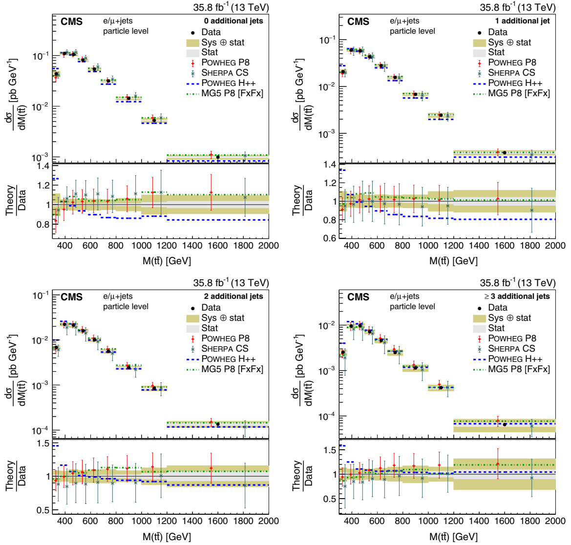
FIG. 32. Differential cross sections at the particle level as a function of M(\bar{t}\bar{t}) in bins of the number of additional jets. The data are shown as points with light (dark) bands indicating the statistical (statistical and systematic) uncertainties. The cross sections are compared to the predictions of POWHEG combined with PYTHIA8 (P8) or HERWIG++ (H++) and the multiparton simulations MG5_ams@NLO (MG5)+PYTHIA8 FxFx and SHERPA. The ratios of the various predictions to the measured cross sections are shown at the bottom of each panel.
