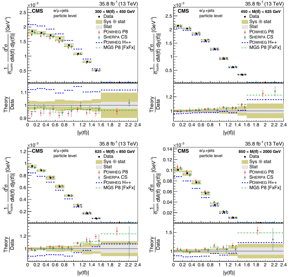
FIG. 25. Normalized double-differential cross section at the particle level as a function of M(\bar{t}\bar{t}) vs. |y(\bar{t}\bar{t})| . The data are shown as points with light (dark) bands indicating the statistical (statistical and systematic) uncertainties. The cross sections are compared to the predictions of POWHEG combined with PYTHIA8 (P8) or HERWIG++ (H++) and the multiparton simulations MG5_AMC@NLO (MG5)+PYTHIA8 FxFx and SHERPA.
