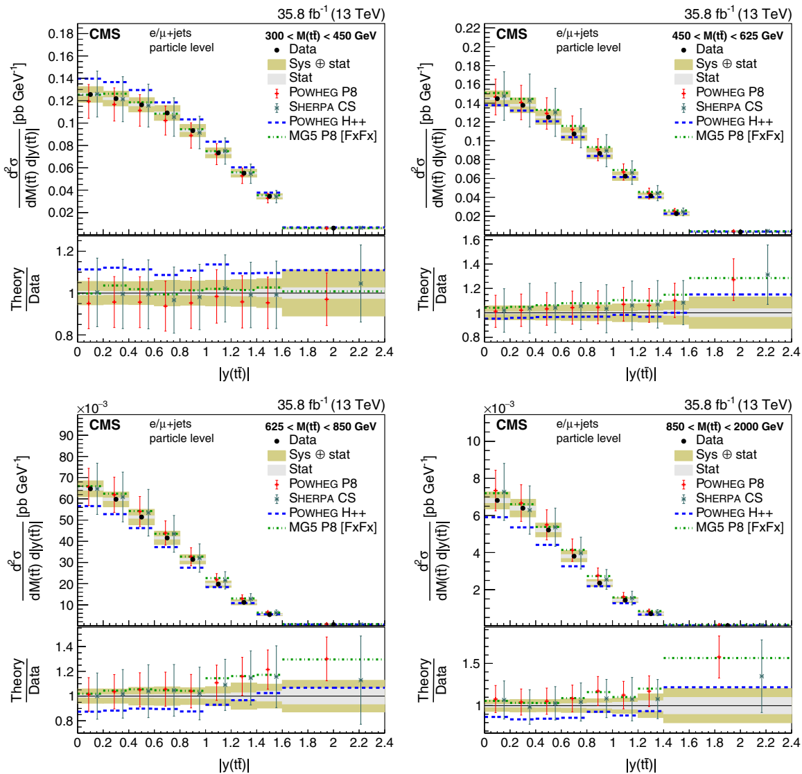
FIG. 24. Double-differential cross section at the particle level as a function of M(\bar{t}\bar{t}) vs. |y(\bar{t}\bar{t})| . The data are shown as points with light (dark) bands indicating the statistical (statistical and systematic) uncertainties. The cross sections are compared to the predictions of POWHEG combined with PYTHIA8 (P8) or HERWIG++ (H++) and the multiparton simulations MG5_amc@NLO (MG5)+PYTHIA8 FxFx and SHERPA. The ratios of the various predictions to the measured cross sections are shown at the bottom of each panel.
