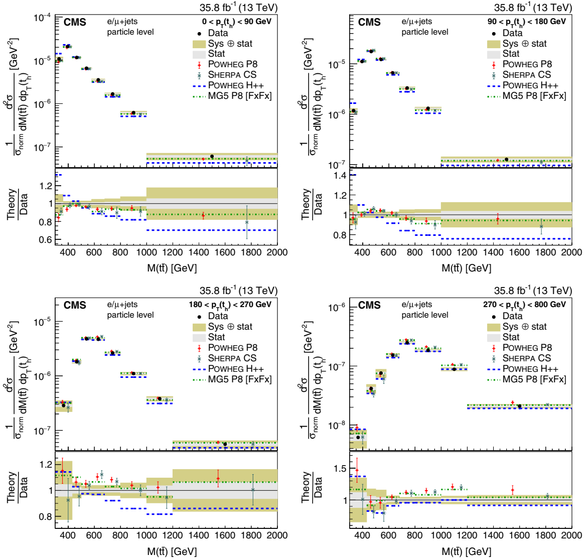
FIG. 29. Normalized double-differential cross section at the particle level as a function of p_T(t_h) vs. M(\bar{t}\bar{t}) . The data are shown as points with light (dark) bands indicating the statistical (statistical and systematic) uncertainties. The cross sections are compared to the predictions of POWHEG combined with PYTHIA8 (P8) or HERWIG++ (H++) and the multiparton simulations MG5_aMC@NLO (MG5)+PYTHIA8 FxFx and SHERPA. The ratios of the various predictions to the measured cross sections are shown at the bottom of each panel.
