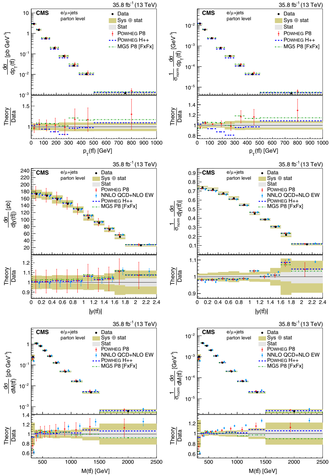
FIG. 16. Absolute (left) and normalized (right) differential cross sections at the parton level as a function of p_T(\bar{t}\bar{t}) (upper), |y(\bar{t}\bar{t})| (middle), and M(\bar{t}\bar{t}) (lower). The data are shown as points with light (dark) bands indicating the statistical (statistical and systematic) uncertainties. The cross sections are compared to the predictions of POWHEG combined with PYTHIA8 (P8) or HERWIG++ (H++), the multiparton simulation MG5_aMC@NLO (MG5)+PYTHIA8 FxFx, and the NNLO QCD + NLO EW calculations. The ratios of the various predictions to the measured cross sections are shown at the bottom of each panel.
