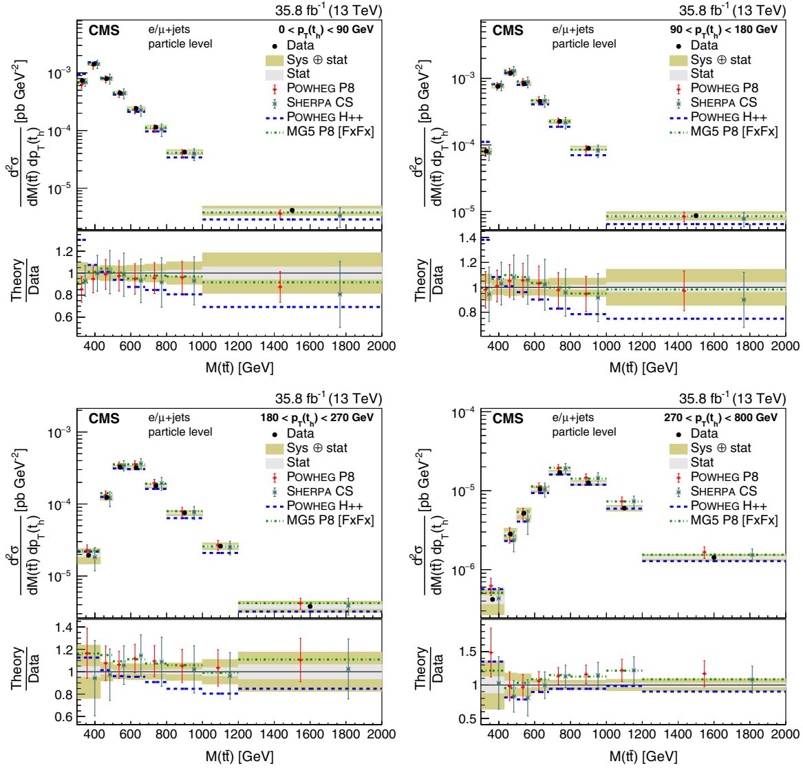
FIG. 28. Double-differential cross section at the particle level as a function of p_T(t_h) vs. M(\bar{t}\bar{t}) . The data are shown as points with light (dark) bands indicating the statistical (statistical and systematic) uncertainties. The cross sections are compared to the predictions of POWHEG combined with PYTHIA8 (P8) or HERWIG++ (H++) and the multiparton simulations MG5_amc@NLO (MG5)+PYTHIA8 FxFx and SHERPA. The ratios of the various predictions to the measured cross sections are shown at the bottom of each panel.
