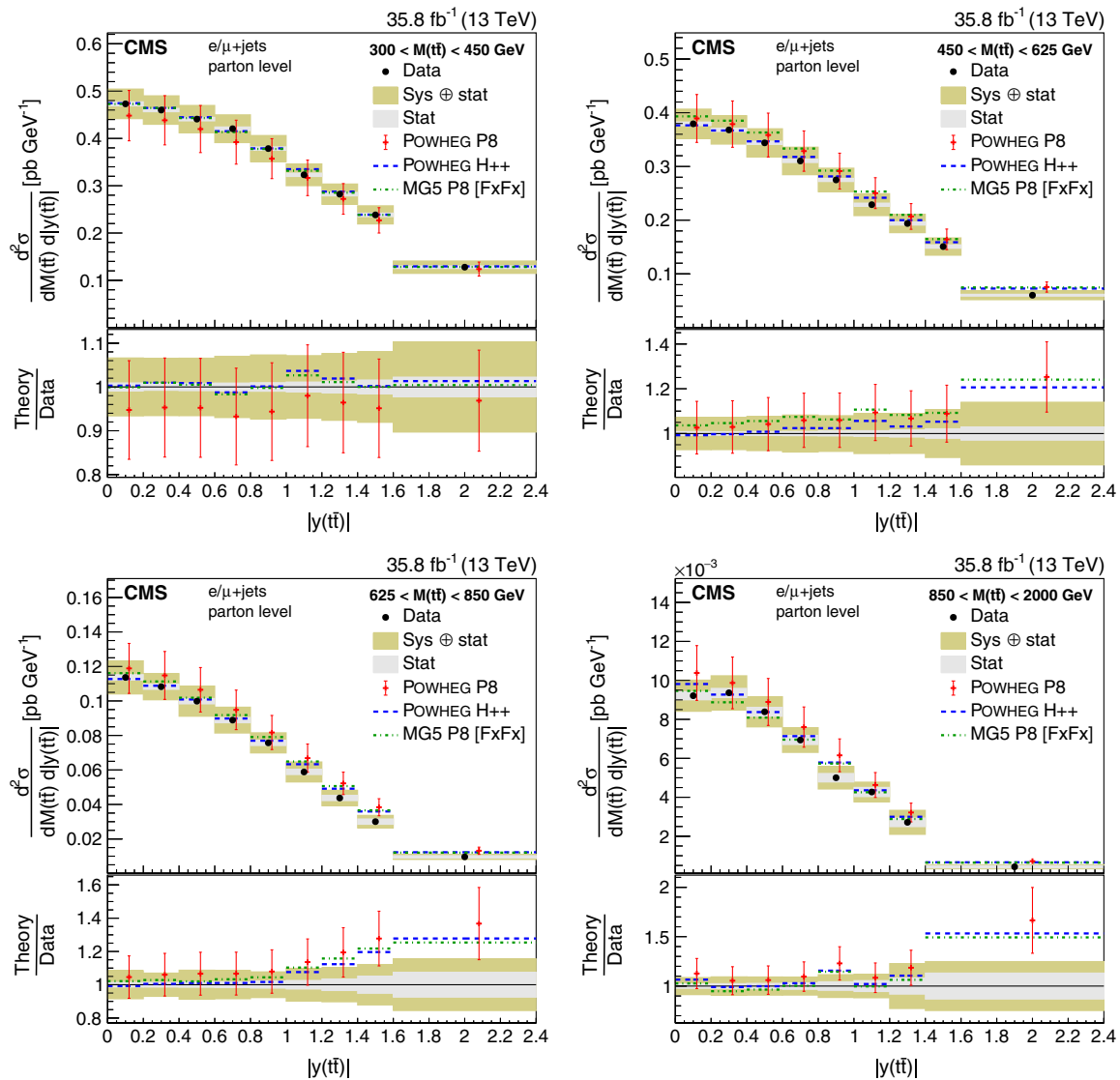
FIG. 22. Double-differential cross section at the parton level as a function of M(\bar{t}t) vs. |y(\bar{t}t)| . The data are shown as points with light (dark) bands indicating the statistical (statistical and systematic) uncertainties. The cross sections are compared to the predictions of POWHEG combined with PYTHIA8 (P8) or HERWIG++ (H++), and the multiparton simulation MG5_ams@NLO (MG5)+PYTHIA8 FxFx. The ratios of the various predictions to the measured cross sections are shown at the bottom of each panel.
