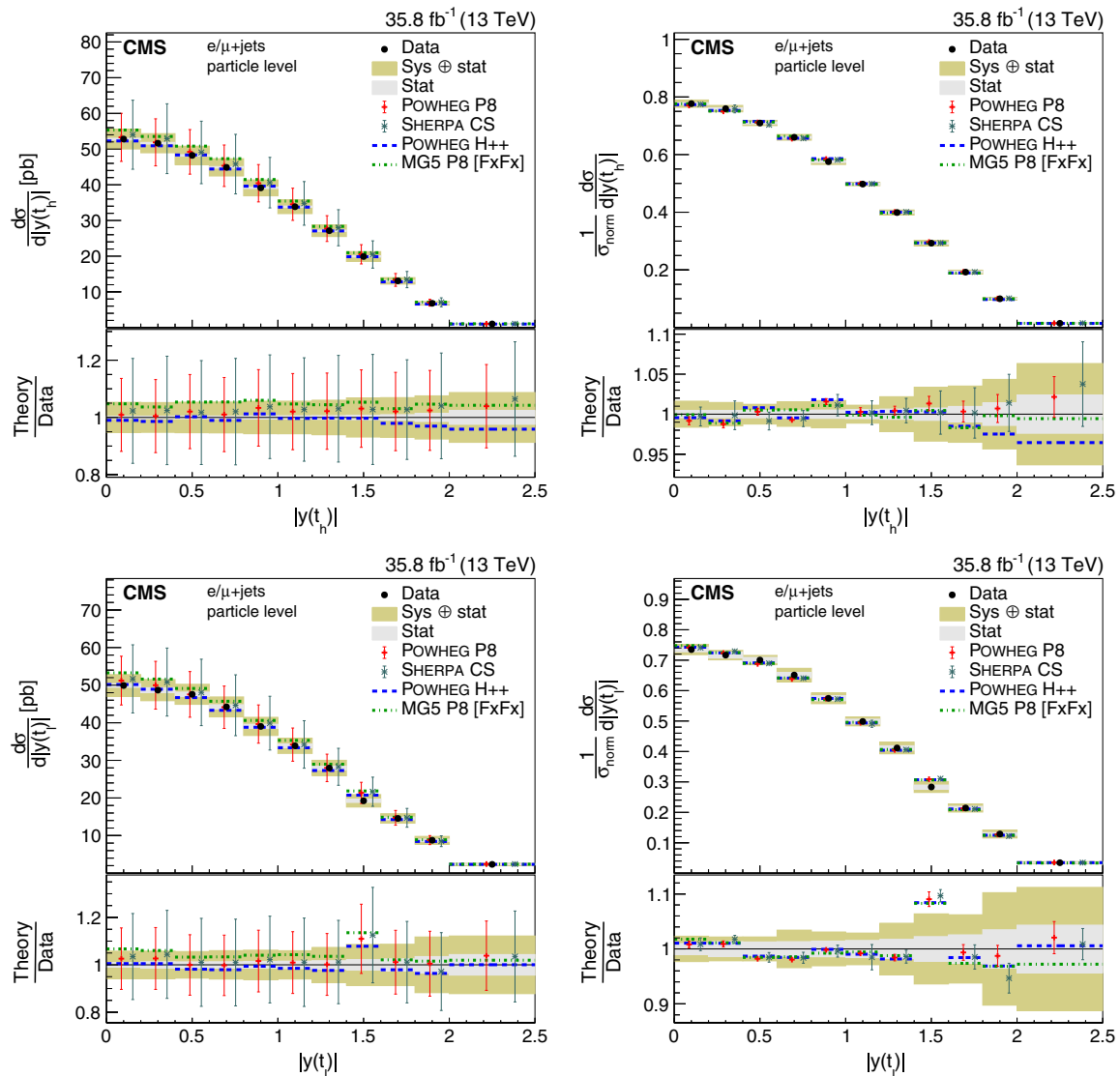
FIG. 14. Absolute (left) and normalized (right) differential cross sections at the particle level as a function of |y(t_h)| (upper) and |y(t_l)| (lower). The data are shown as points with light (dark) bands indicating the statistical (statistical and systematic) uncertainties. The cross sections are compared to the predictions of POWHEG combined with PYTHIA8 (P8) or HERWIG++ (H++) and the multiparton simulations MG5 AMC@NLO (MG5)+PYTHIA8 FxFx and SHERPA. The ratios of the various predictions to the measured cross sections are shown at the bottom of each panel.
