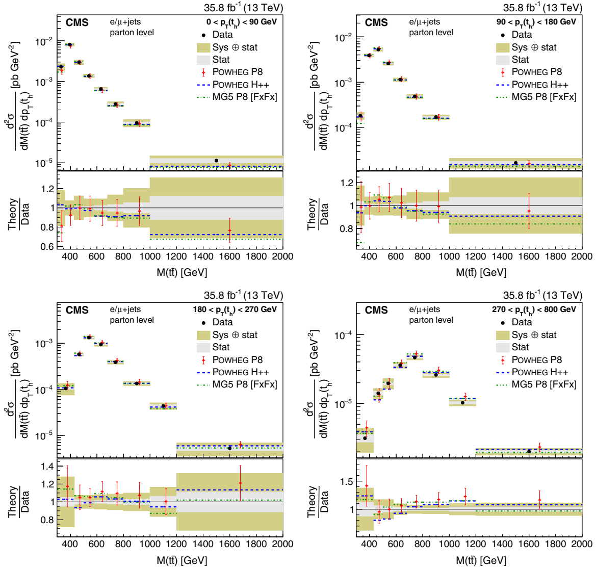
FIG. 26. Double-differential cross section at the parton level as a function of p_T(t_h) vs. M(\tilde{t}\bar{t}) . The data are shown as points with light (dark) bands indicating the statistical (statistical and systematic) uncertainties. The cross sections are compared to the predictions of POWHEG combined with PYTHIA8 (P8) or HERWIG++ (H++), and the multiparton simulation MG5_AMC@NLO (MG5)+PYTHIA8 FxFx. The ratios of the various predictions to the measured cross sections are shown at the bottom of each panel.
