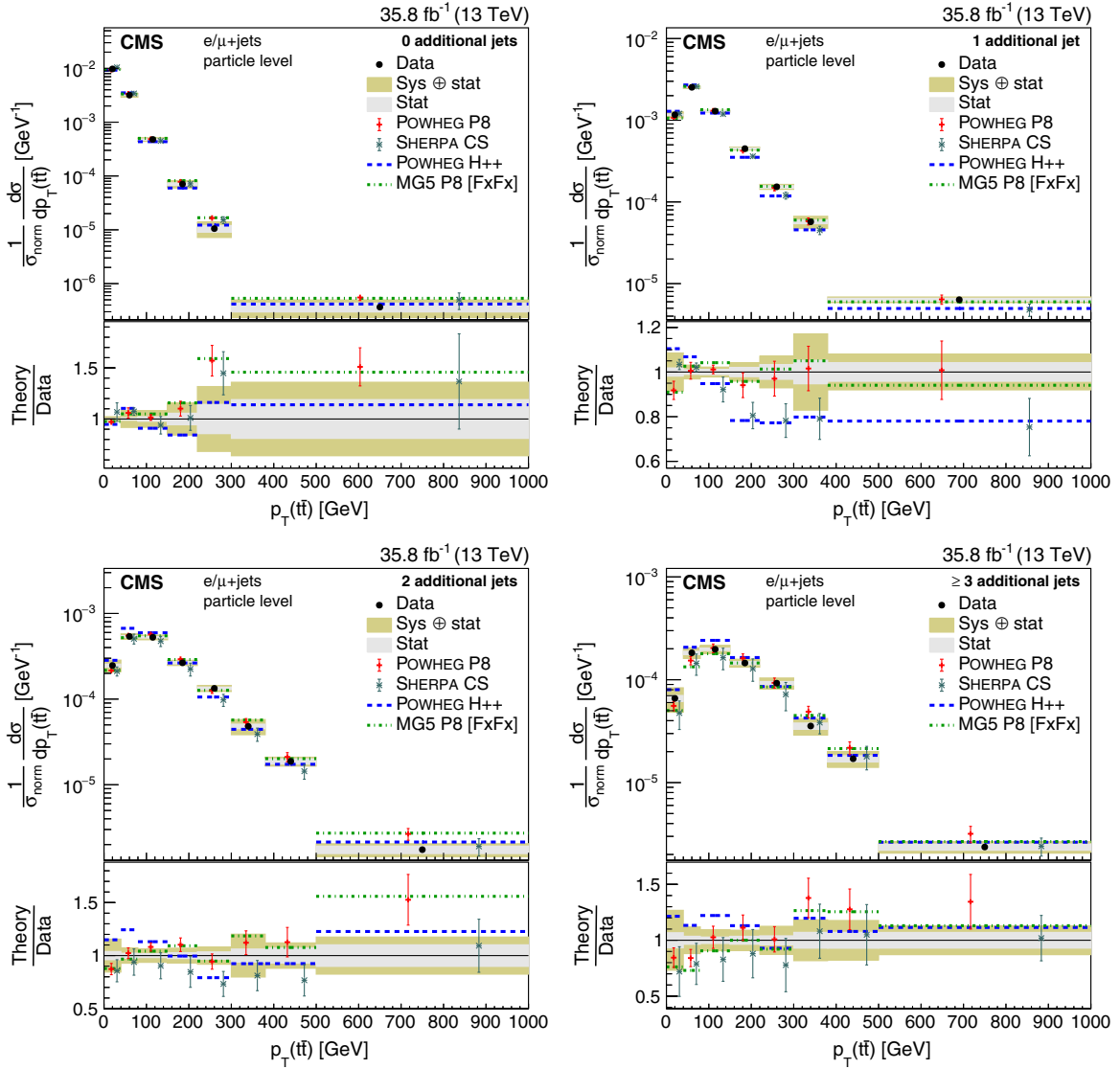
FIG. 35. Differential cross sections at the particle level normalized to the sum of the cross sections \sigma_{\text{norm}} in the measured ranges as a function of p_T(\tilde{t}\bar{t}) in bins of the number of additional jets. The data are shown as points with light (dark) bands indicating the statistical (statistical and systematic) uncertainties. The cross sections are compared to the predictions of POWHEG combined with PYTHIA8 (P8) or HERWIG++ (H++) and the multiparton simulations MG5_AMC@NLO (MG5)+PYTHIA8 FxFx and SHERPA. The ratios of the various predictions to the measured cross sections are shown at the bottom of each panel.
