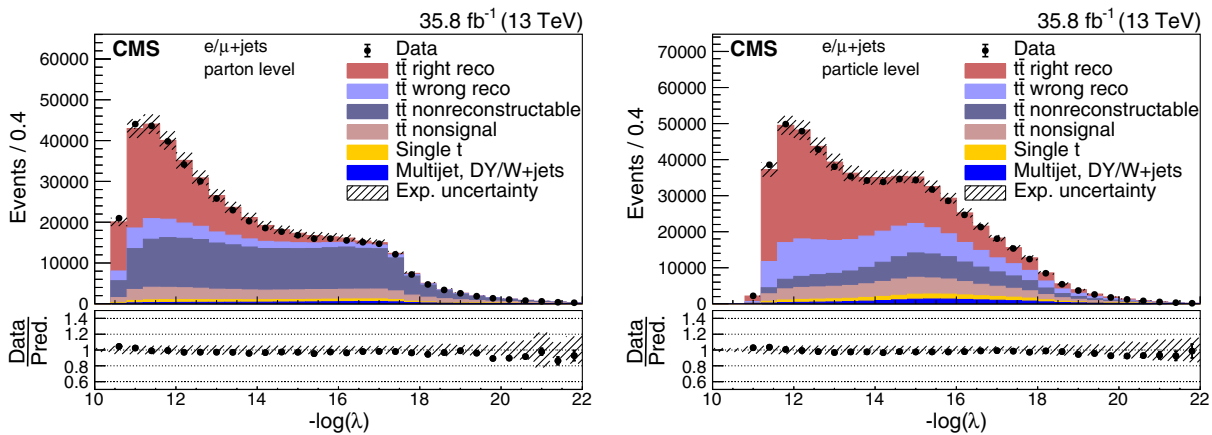
FIG. 4. Distribution of the negative log-likelihood for the selected best permutation in the (left) parton- and the (right) particle-level measurements in data and simulations. Events generated with POWHEG+PYTHIA8 are used to describe the t\bar{t} production. The contribution of multijet, DY, and W boson plus jets background events is extracted from the data (cf. Sec. VII). Combined experimental (cf. Sec. IX) and statistical uncertainties (hatched area) are shown for the total predicted yields. The data points are shown with statistical uncertainties. The ratios of data to the sum of the predicted yields are provided at the bottom of each panel.
