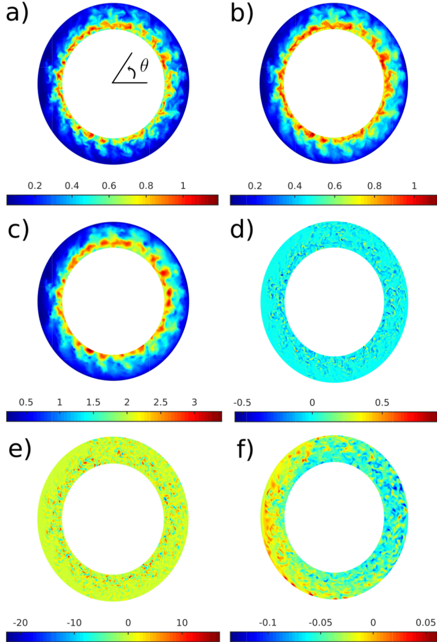
FIG. 1. Snapshots of plasma turbulence in the standard ISTTOK simulation on a poloidal cross section halfway between the limiter plate ( \varphi = \pi ). We show: (a) plasma density n/n_0 , (b) electron temperature T_e/T_{e0} , (c) electrostatic potential \phi/eT_{e0} , (d) vorticity \omega = \rho_{s0}^2 \nabla_\perp^2 \phi/eT_{e0} , (e) electron V_{\parallel e}/c_{s0} , and (f) ion V_{\parallel i}/c_{s0} parallel velocities.
