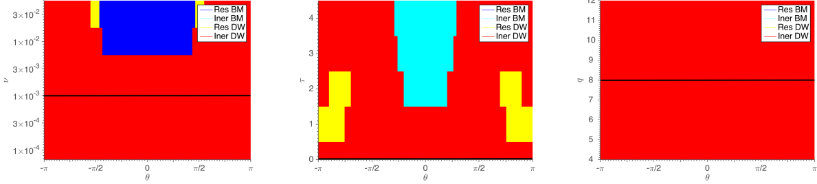
FIG. 8. Turbulent regimes as a function of the poloidal angle \theta and normalised resistivity, \nu (upper left panel), ion to electron temperature ratio \tau (middle panel), and safety factor q (right panel). The Resistive BM driven turbulence is in dark blue, Inertial BM in light blue, Resistive DW in yellow, and Inertial DW in red. The black lines represent the standard ISTTOK case.
