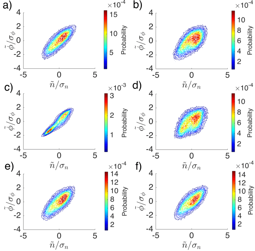
FIG. 5. Probability of correlation between density and electric potential fluctuations normalized to their respective standard deviation, resulting from GBS simulations with standard ISTTOK parameters (top), and when DW (middle) or BM (bottom) are removed from the system. The HFS (left) and LFS (right) are shown.
