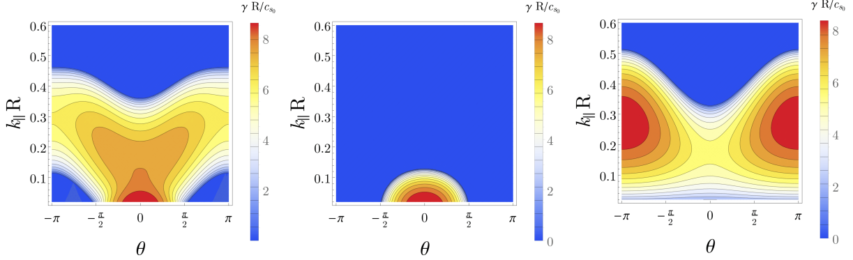
FIG. 4. Linear growth rate as a function of the poloidal angle, \theta , and of the parallel wavenumber normalized to the major radius k_{\parallel}R . From left to right: the solution of the full dispersion relation that couples inertial DW and BM, Eq. (8); the solution of Eq. (10) for the pure BM; and the solution of Eq. (11) for the pure DW.
