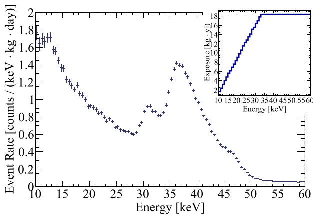
Fig. 5 Efficiency-corrected energy spectrum of CUORE-0 from 10 to 60 keV corresponding to an exposure ranging from 1.6 kg year at 10 keV up to 18.56 kg year at 35 keV, as shown in the inset
