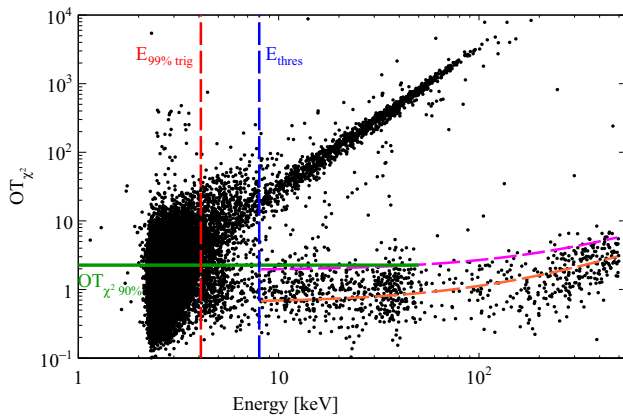
Fig. 2 A typical distribution of OT_{\chi^2} as a function of energy for one BoDs. Physical events due to the particle interactions in the \text{TeO}_2 crystals are distributed in a nearly-horizontal band around OT_{\chi^2} \sim 1 . Non-physical events such as electronic noise and tower vibrations, as well as particle interactions in the thermistors, follow an oblique distribution. The green solid line corresponds to the 90th percentile of the OT_{\chi^2} distribution ( OT_{\chi^2 90\%} ) calculated in the region [35–50] keV and OT_{\chi^2} < 10 using physics data. The magenta (orange) dashed line corresponds to the 90th (50th) percentile calculated using calibration data in the region [100–500] keV and OT_{\chi^2} < 10 , assuming linear dependence on energy. Red and blue dashed vertical lines represent the trigger threshold E_{99\% \text{ trig}} and the analysis threshold E_{\text{thres}} , respectively
