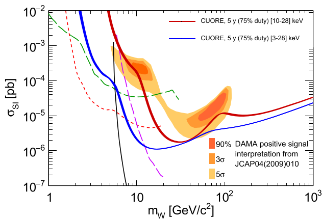
Fig. 6 90% sensitivities on the SI elastic WIMP-nucleon cross section as a function of WIMP mass of CUORE, assuming 5 years of data-taking with 75% of duty cycle and 10 keV threshold (red), as well as 3 keV threshold (blue). Uncertainty on the energy scale dominated by the nuclear quenching factor is taken into account. DAMA/LIBRA positive signal reported in [31] is shown as yellow/dark yellow/orange islands. The results from CRESST-II (dashed green) [32], CDMS Lite (dashed red) [33], XMASS (dashed violet) [34], and LUX (black solid) [35] are also shown
