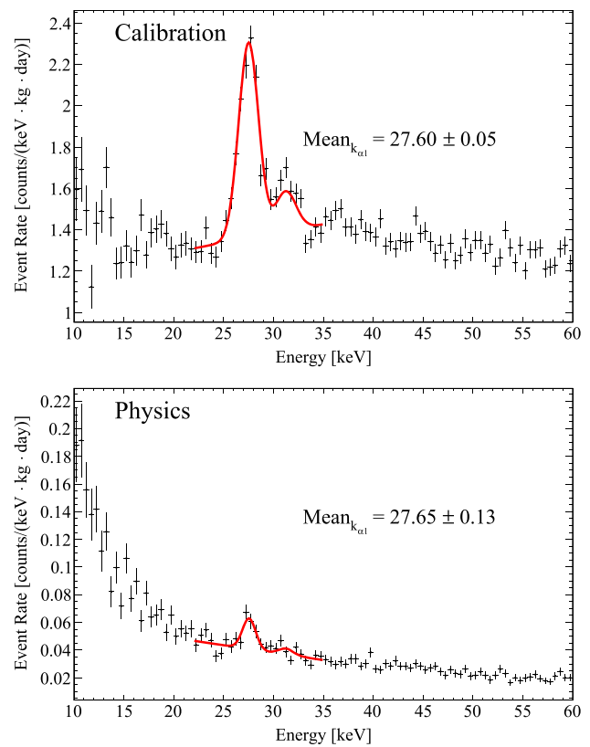
Fig. 4 CUORE-0 summed energy spectra of events with double-crystal coincidence in calibration (top) and physics (bottom) data, along with fits to an eight-Gaussian line shape plus linear background (red solid lines)
