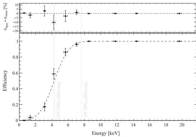
Fig. 1 (Bottom): An example of the trigger efficiency obtained from Eq. 1 as a function of energy (dashed line) and data obtained from low energy pulser measurements (circles). Energies where OT trigger efficiency reaches 50% ( \theta ) and 99% ( E_{99\% \text{ trig}} ) are shown as vertical gray lines. (Top): The difference between the model and the data
