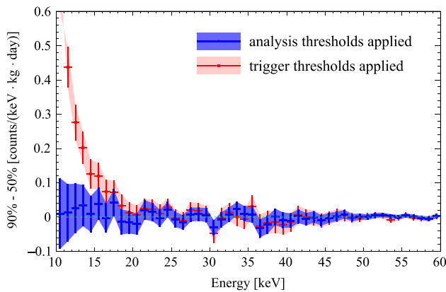
Fig. 3 OT_{\chi^2} selection efficiency corrected rate difference between the background spectra calculated for OT_{\chi^2 90\%} and OT_{\chi^2 50\%} . (See Sect. 4.3 for a description of analysis and trigger thresholds.)
