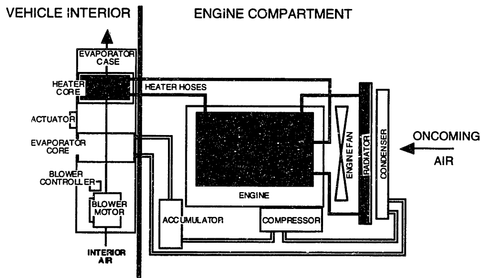
Figure 1: Automotive climate control system component schematic.
