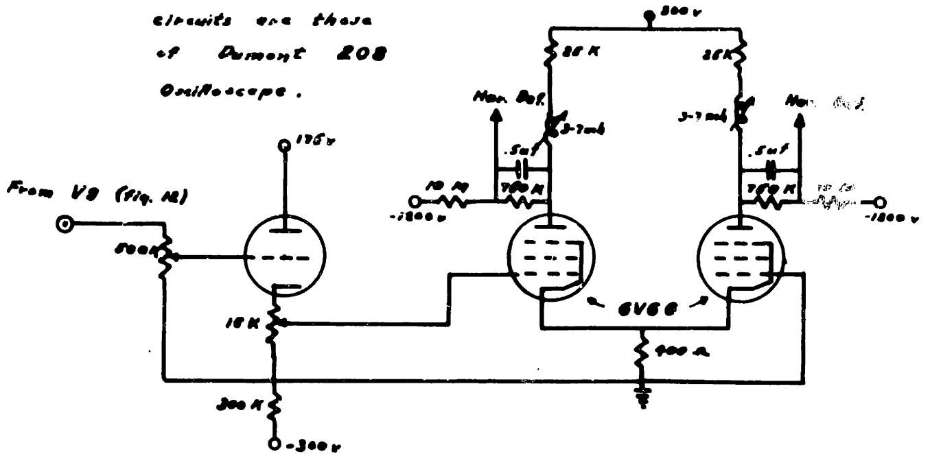
Circuit Diagram for Coder No. 2
