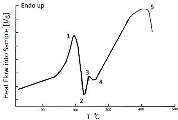
FIGURE 1. SCHEMATIC REPRESENTATION OF DSC SIGNAL BASED ON [6]. PEAKS AND TROUGHS ARE ATTRIBUTED TO DISSOLUTION AND FORMATION OF PRECIPITATES.
