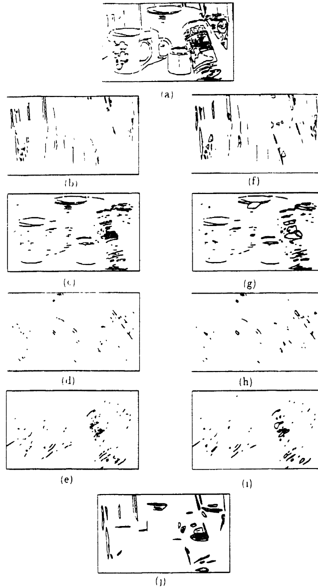
Figure 5.5: Illustration of grouping based on closely-spaced parallelism and salient group detection — Another example. (a) Line segments to be grouped based on closely-spaced parallelism. (b)-(e) Line segments shown along four major orientations, namely, vertical, horizontal, obtuse, and acute orientations. (f)-(i) The line groups formed using the algorithm shown also along the respective major orientations for clarity. The thresholds used were t_{\text{across}} = 6 , t_{\text{along}} = 5 , t_{\text{local-orient}} = 6^\circ , t_{\text{global-orient}} = 10^\circ . (j) The 40 most salient groups among the line groups of (f) - (i) found using the saliency measure. Note that only two of the salient groups span more than one object.
