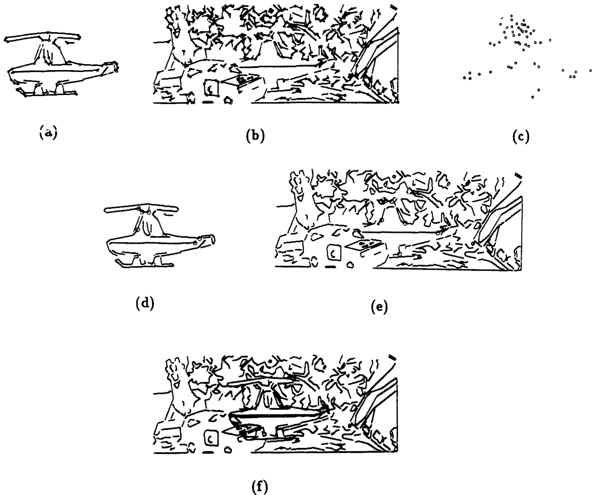
Figure 8.4: Illustration of recognition within the regions selected by the attention mechanism using only color. (a) The primary view of the model object showing corner (in circles) and line features. (b) An edge image of a scene showing corner (again in circles) and line segments. The model object and the scene are those depicted in Figure 8.3. (c) The corner features in the region selected by the attentional selection mechanism that was indicated in Figure 8.3h. (d) - (e) A set of corner features in the model and image that were declared to be a match using interpretation tree search in the matching stage of the recognition system. (f) The model object projected into the image using the alignment transform computed from the set of matched features shown in (d) and (e). The projected view was verified to be correct by the verification stage of the recognition system.
