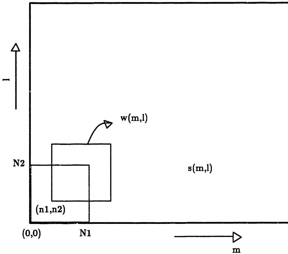
Figure 4.1: Illustration of moving window analysis for computing the short-space Fourier transform.
