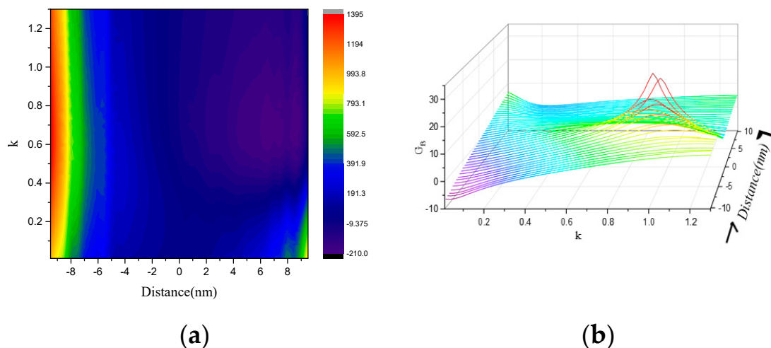
Figure 8. Electric dipole excitation: (a) Purcell factor and (b) Far-field forward-to-backward directionality G_{FS/BS_{max}} versus the coefficient \kappa for different distances.
