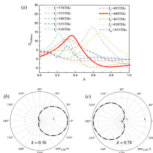
Figure 3. (a) Far-field forward-to-backward directionality G_{FS/BS_{max}} for different frequencies. (b) Scattering pattern for \kappa = 0.36 . (c) Scattering pattern for \kappa = 0.78 .
