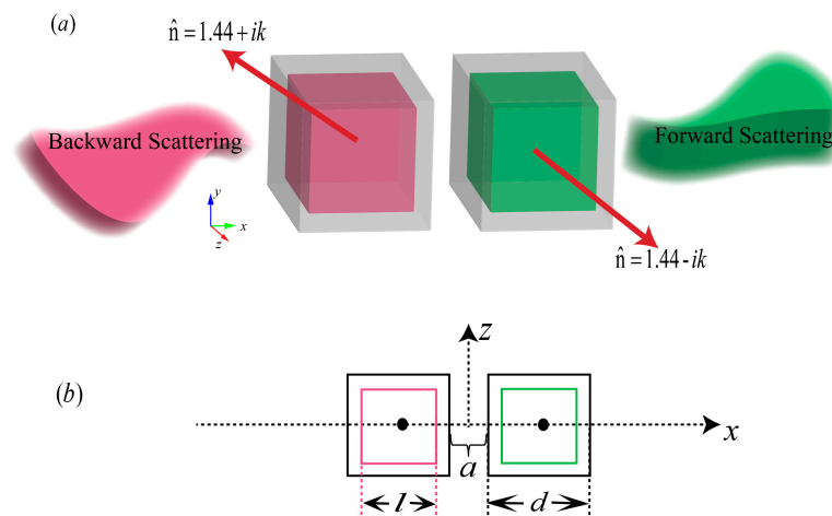
Figure 1. Schematic of the core-shell nanocube dimer with balanced gain and loss. (a) three-dimensional diagram (b) x - z plane graph.
