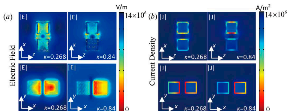
Figure 6. (a) Electric field distribution and (b) Current density of the core-shell nanocube dimer for \kappa = 0.268 and \kappa = 0.84 .
