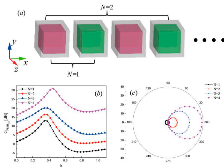
Figure 7. (a) Schematic of the core-shell nanocube dimer in a chain (b) Far-field forward-to-backward directionality G_{FS/BS_{max}} and (c) Scattering patterns of the chained core-shell nanocube dimer for N = 1, 2, 3 , and 4.
