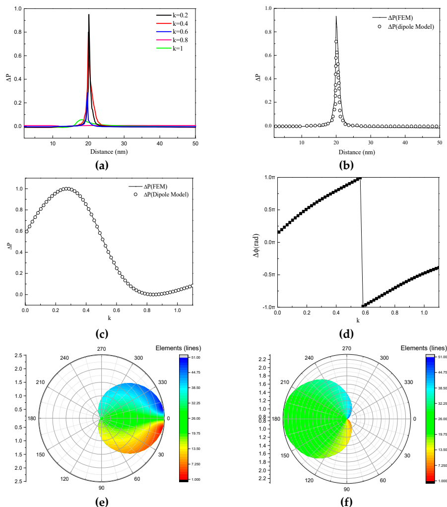
Figure 5. (a) Power difference \Delta P spectrum with face-to-face distance of the core-shell nanocube dimer (b) Power difference \Delta P spectrum with different face-to-face distance obtained by the analytic expression and finite element method (FEM) (c) Power difference \Delta P spectrum with different \kappa obtained by the analytic expression and FEM (d) Phase difference between the electric dipoles (EDs), (e) Far-field distributions at \kappa = 0.268 , and (f) Far-field distributions at \kappa = 0.84 .
