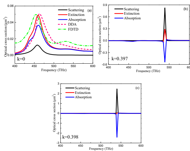
Figure 2. Calculated optical cross-section spectra of the core-shell nanocube dimer with a different coefficient \kappa in the core. (a) \kappa = 0 (b) \kappa = 0.397 (c) \kappa = 0.398 .
