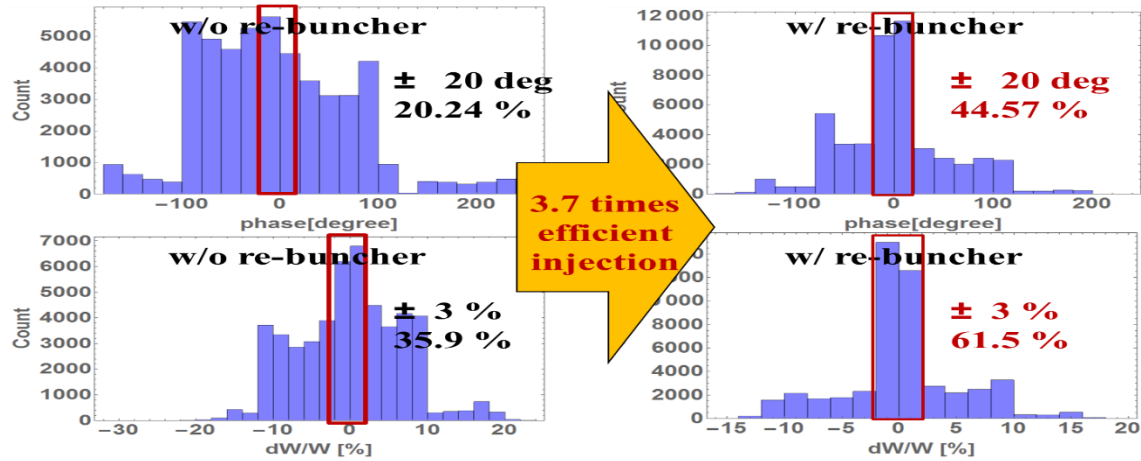
Figure 6 : Comparison result of re-buncher effects on the particle distributions
