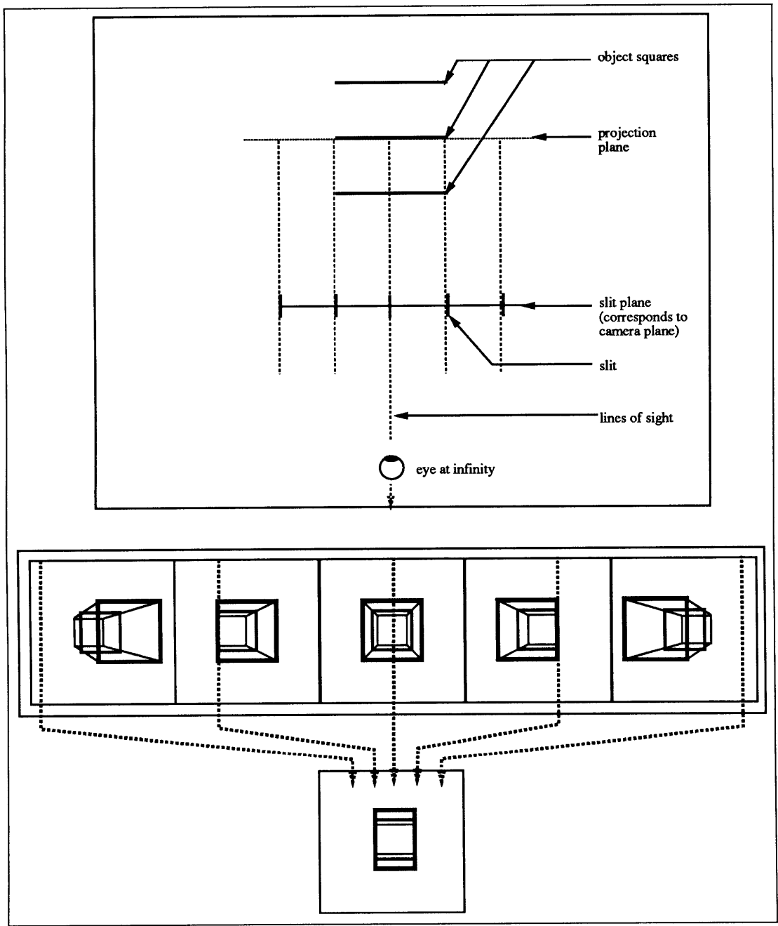
Figure 4.3: When the stereogram is viewed from an infinite view distance, the viewer sees the parts of the projection screen located directly in front of each camera during capture. The result is that the three squares have the same horizontal extent: the front square has shrunk and the rear square has stretched horizontally.
