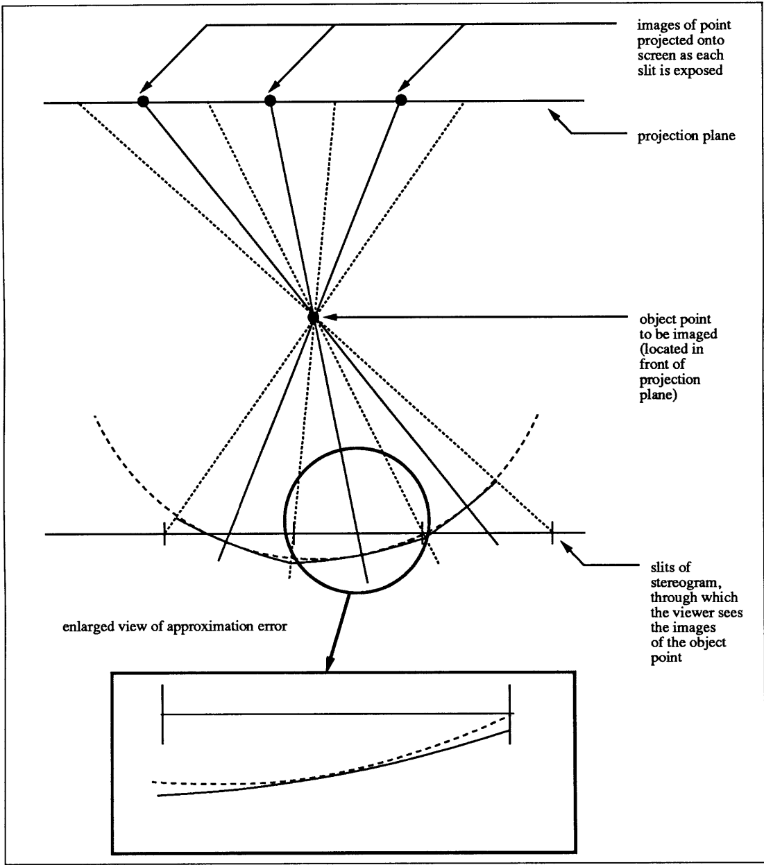
Figure 2.15: Object points in front of the projection plane are approximated by wavefront segments of lesser curvature than the actual wavefront.
