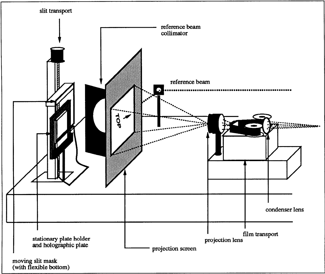
Figure 2.9: Holographic table layout for a recentered stereogram.
