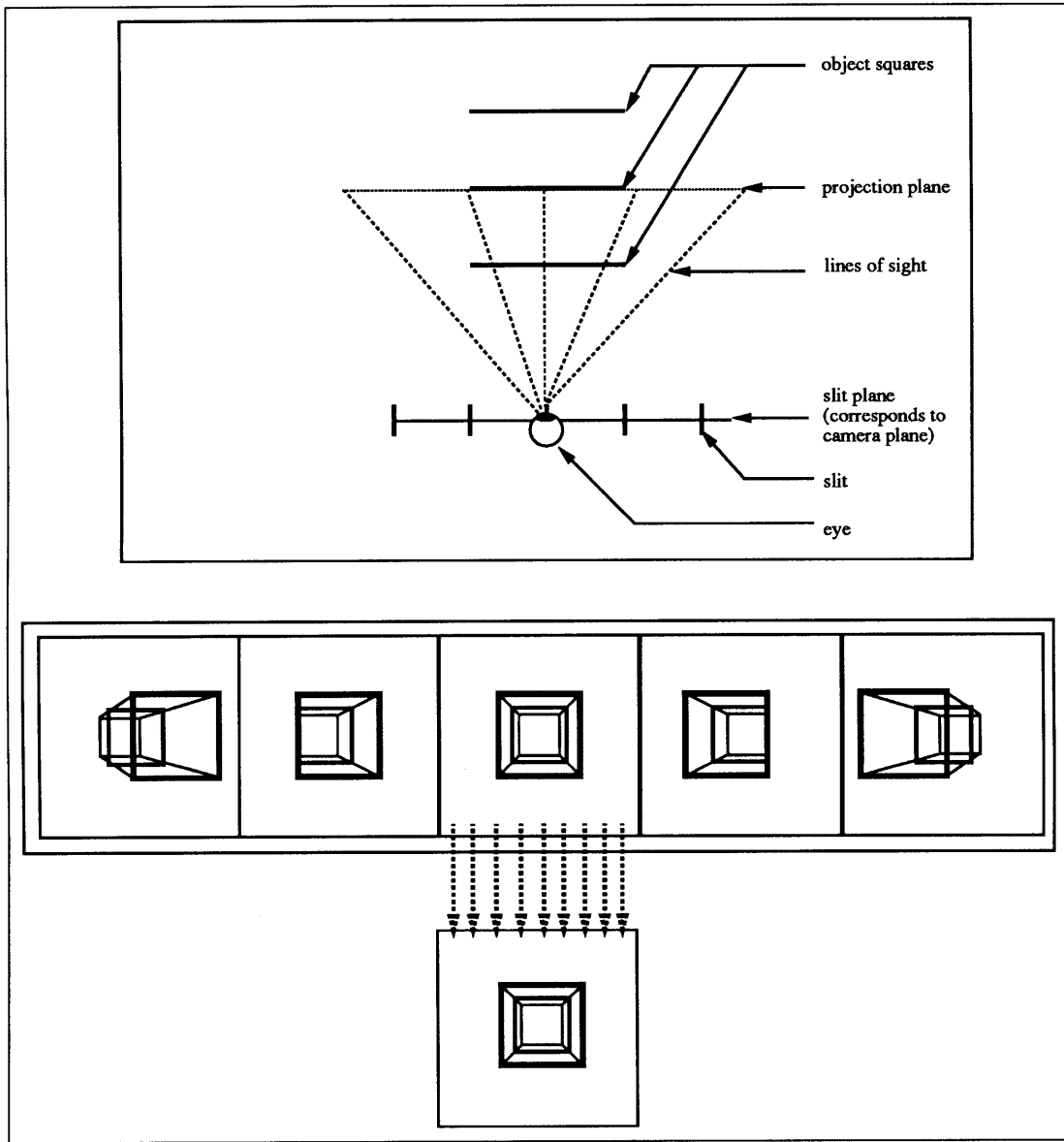
Figure 4.2: When the viewer is located at the slit plane of the stereogram, only one camera view is visible. The presented image, shown at the bottom, is identical to one of the images of the sequence.
