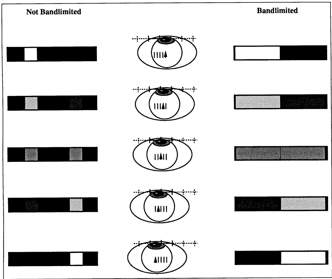
Figure 3.4: Bandlimiting of a stereogram image eliminates the gaps between the images of object points when the viewer's eye falls within more than one slit.
