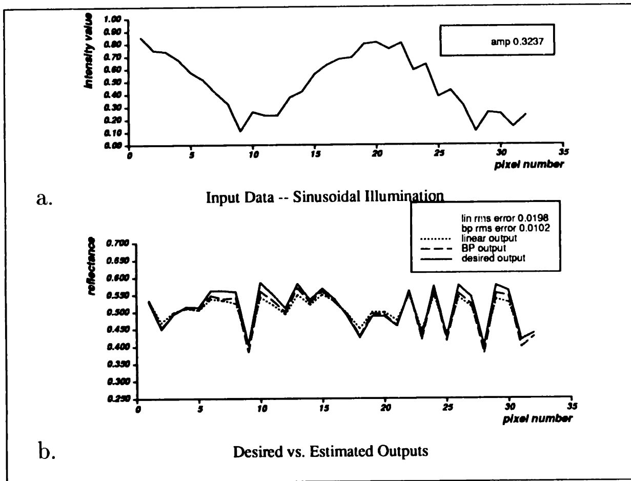
Figure 5.6: (a) Input data, a one-dimensional vector 32 pixels long, consisting of Mondrian reflectance pattern added to sinusoidally varying illumination gradient. (b) Outputs of linear operator (dotted line) and BP operator (dashed line) trained on the same set of 10000 examples under sinusoidal illumination gradients, of which (a) was not one, compared with correct output (solid line).
