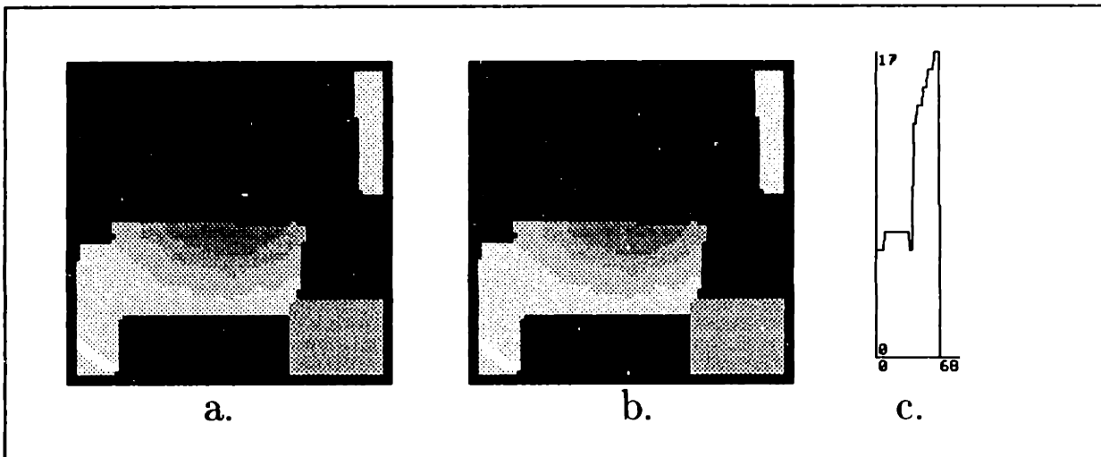
Figure 6.5: Images obtained after (a) five and (b) ten iterations of the winner-take-all scheme on the “v” image, using the Canny edges of the intensity image (see Figure 6.8(b)) as edge input. Note that even after ten iterations, the regions within intensity edges still are not smooth, because the initial discretization into bins cannot be overcome. (c) Vertical slice through (a), showing clearly the discrete levels.
