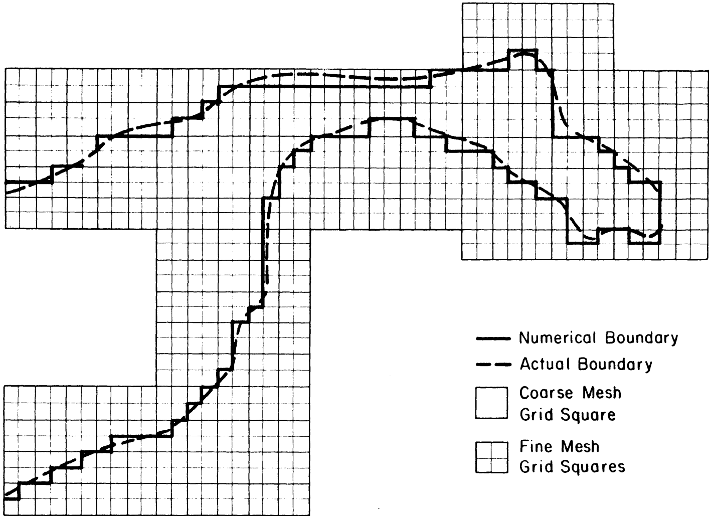
Fig. 6.1.1 The Grid Mesh and Numerical Watershed Boundary
