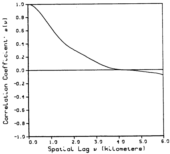
Spatial Correlation
