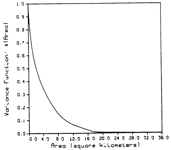
Variance Function
