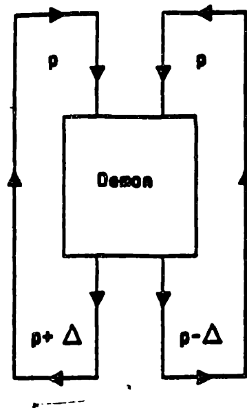
Figure 1.15: A Maxwell demon, creating a 'pressure' difference between two vessels initially at equal pressure
