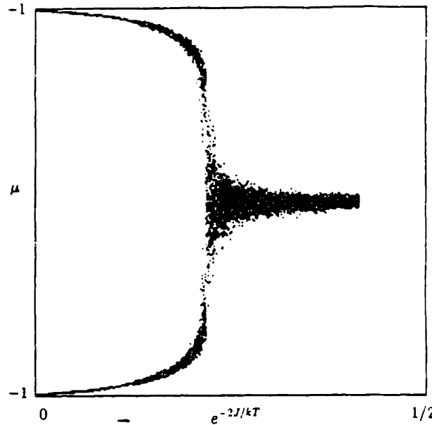
Figure 7.10: Magnetization \mu in the canonical-ensemble model, versus the Monte Carlo acceptance probability. Note the sharp transition at the critical temperature T_{crit} .
