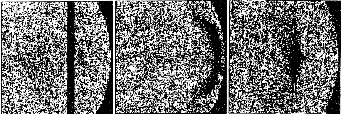
Figure 7.5: A plane pulse traveling towards a concave mirror (a) is shown right after the reflection (b) and approaching the focal point (c).
