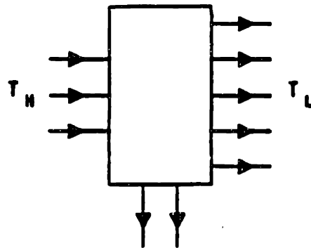
Figure 1.16: Hot (ball-rich) inputs come in from the left, cooler (ball-poorer) outputs leave to the right, while some number of streams of balls (constant 1's) leave from the bottom
