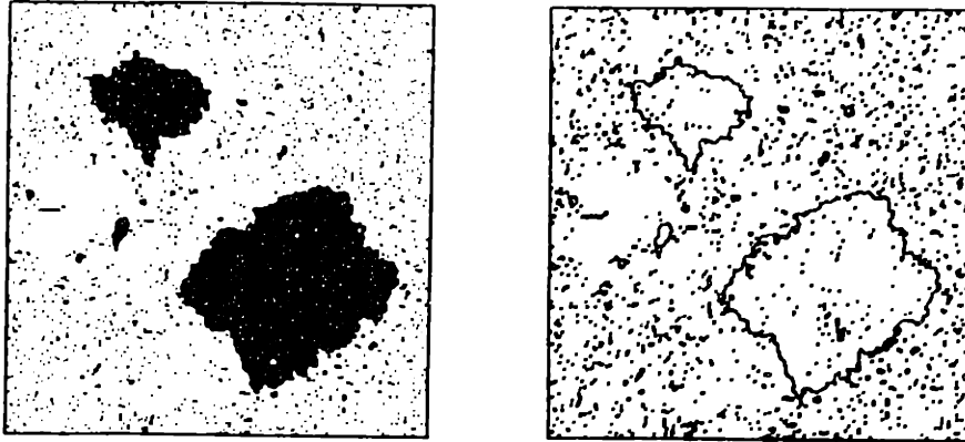
Figure 7.9: (a) A typical spin configuration; (b) the same configuration, but displaying the energy rather than the spins.
