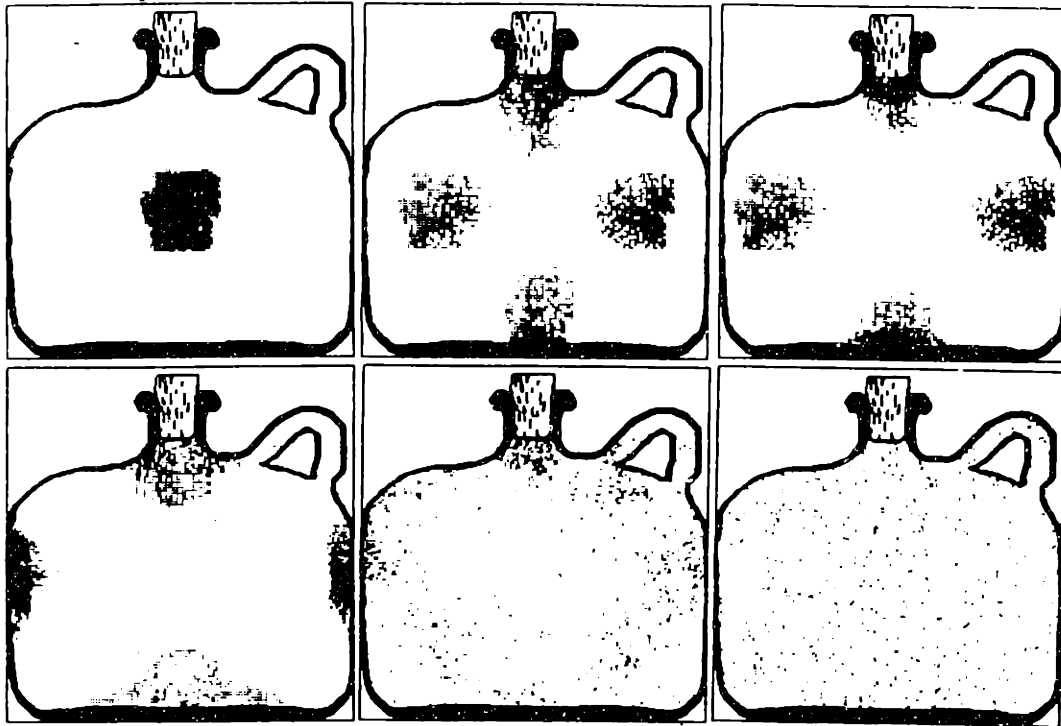
Figure 7.4: Expansion of a TM-GAS cloud in a vacuum. Repeated collisions between particles and with container's walls eventually lead to thorough thermalization.
