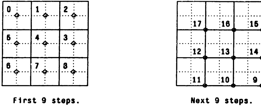
Figure 6.2: A 6 \times 6 lattice with periodic boundaries. All 2 \times 2 blocks in the solid partition are updated, and then all blocks in the dotted partition. Because of periodicity, 9 through 17 mark the centers of dotted blocks.
