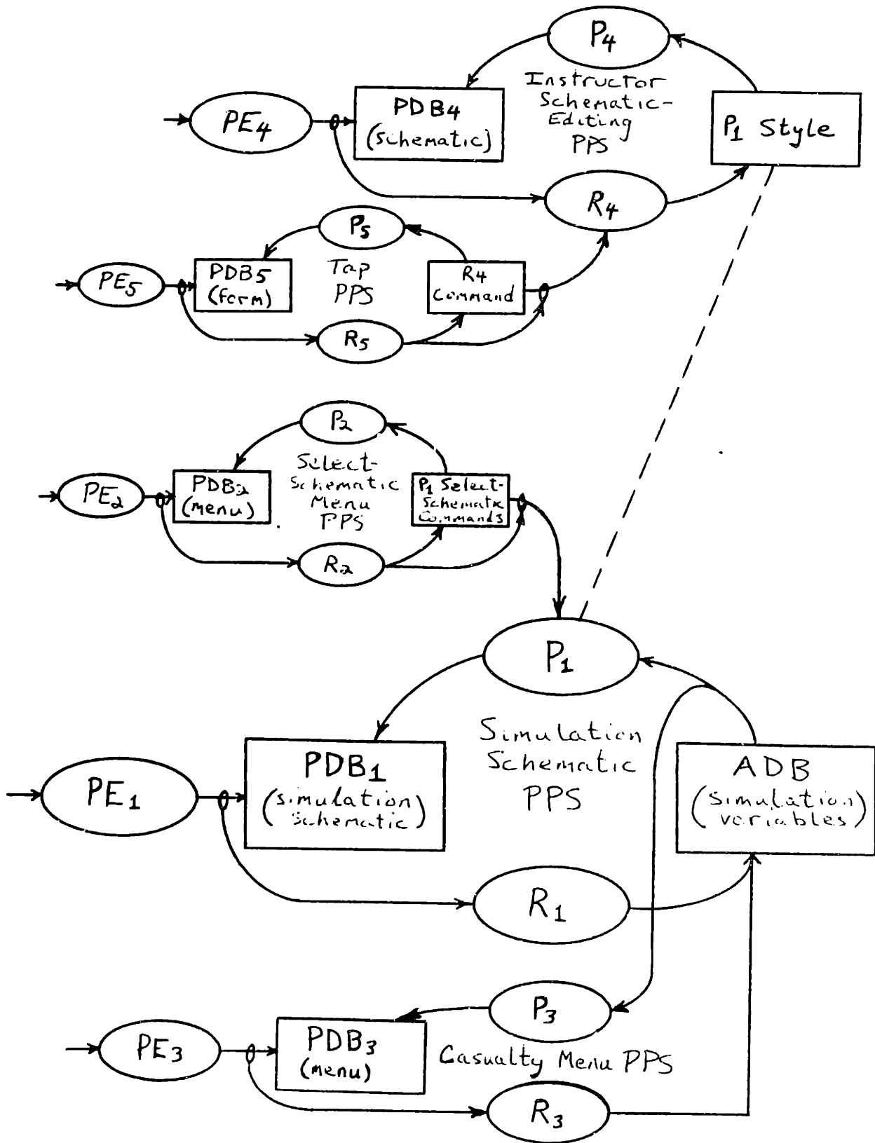
Figure 4-11: Steamer Model
