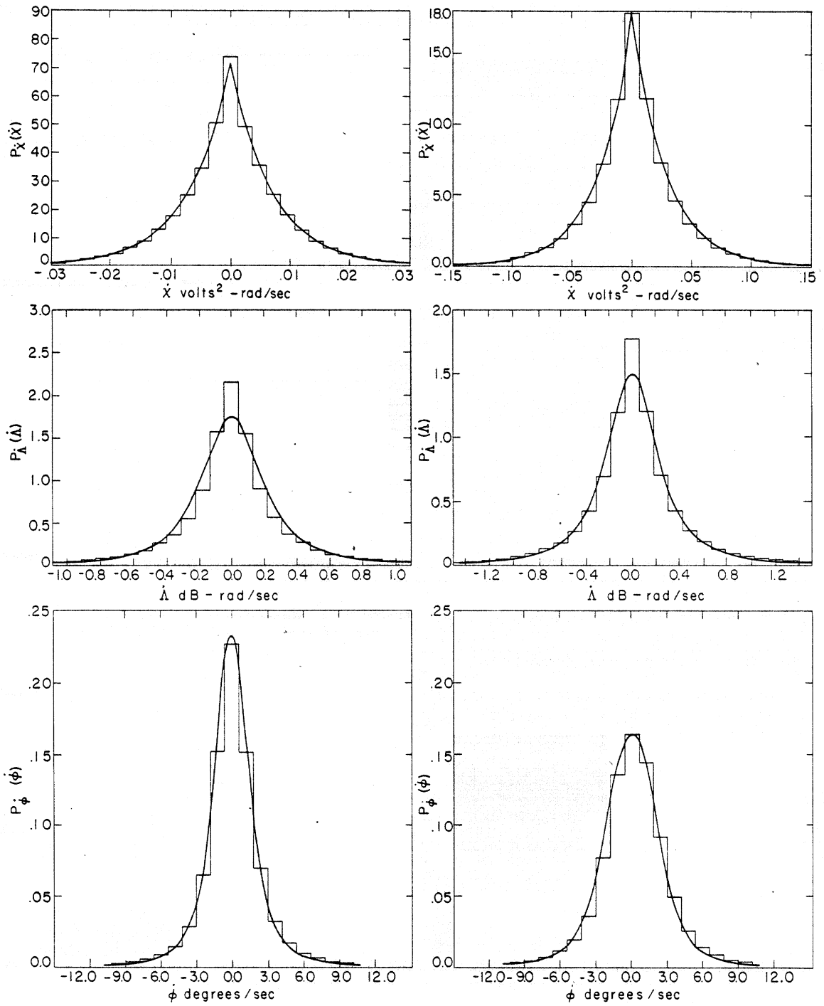
Fig. 59 Histograms from Record 424 for \dot{X} , \dot{A} , and \dot{\phi} , and the least chi-square fit of eqs (1.4), (1.7) and (1.176), respectively. Results for 220 Hz are on the left, and 406 Hz on the right.
