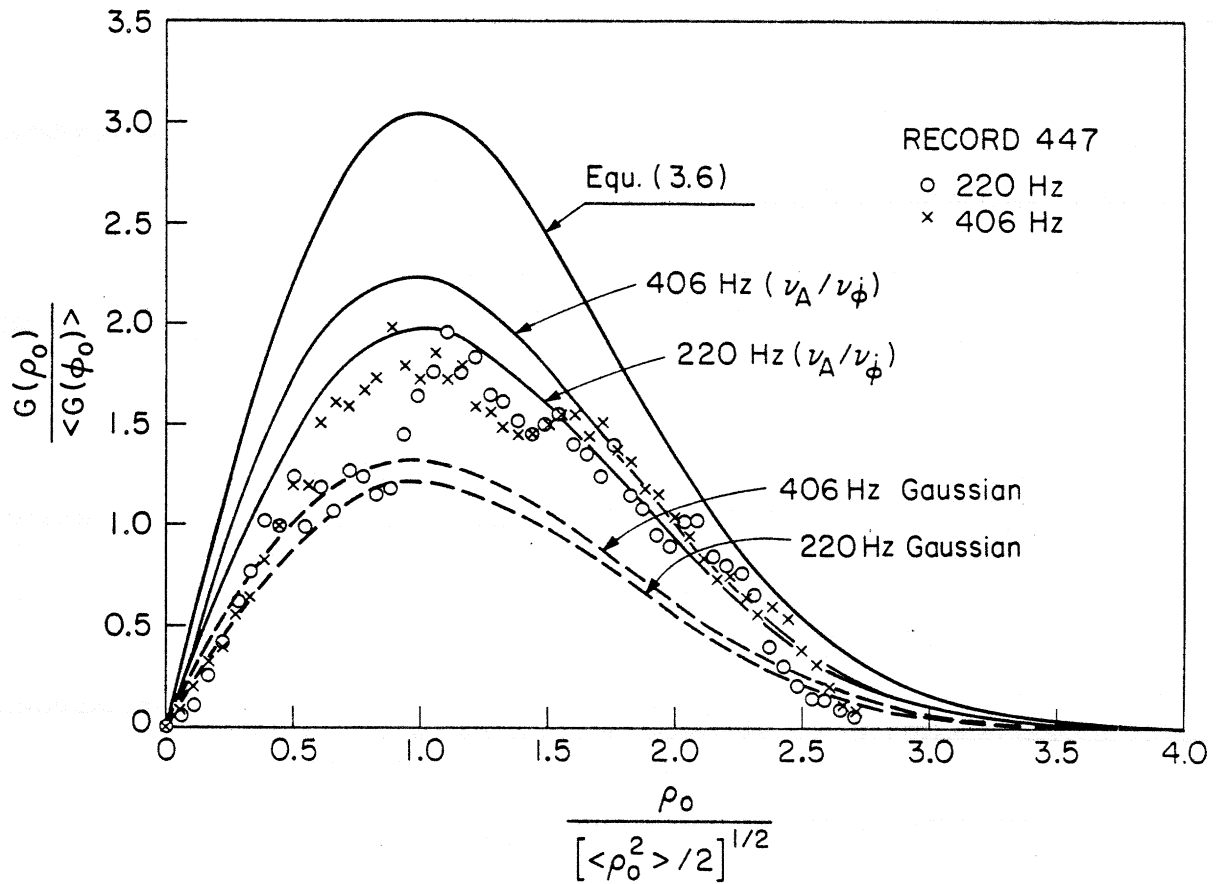
Fig.64 Ratio of phase period to amplitude period, versus amplitude, for record 447. Equ. (3.6) is the theoretical ratio for a non-modulated narrowband source. The correction factors \nu_A/\nu_\phi (Table XV), and Equ. (1.209) (Gaussian modulation) have been applied to obtain the corrected curves for 220Hz and 406Hz accounting for the modulation.
