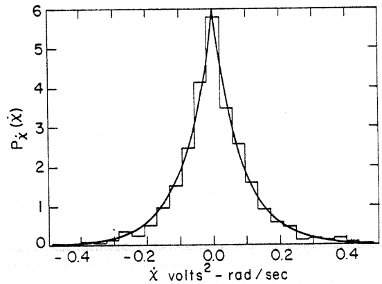
Fig. 18 Computer generated histogram of \dot{X} for N=12 paths and equ. (1.4).
