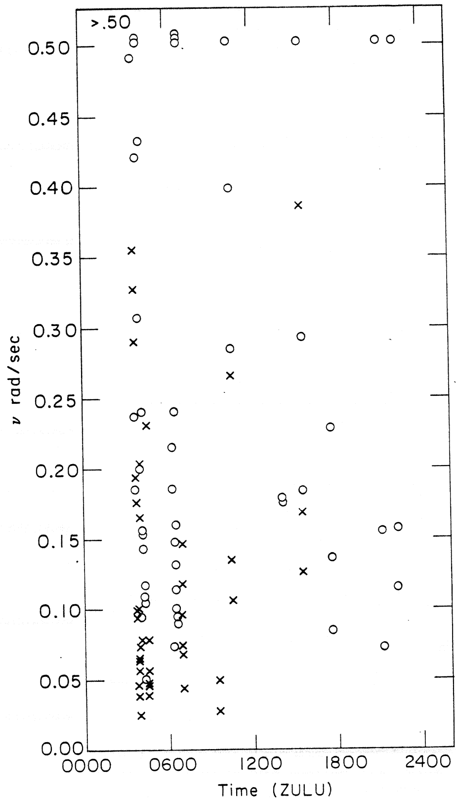
Fig. 77 A plot of \nu vs. time of day. The circles represent 15 Hz, the x's 33 Hz.
