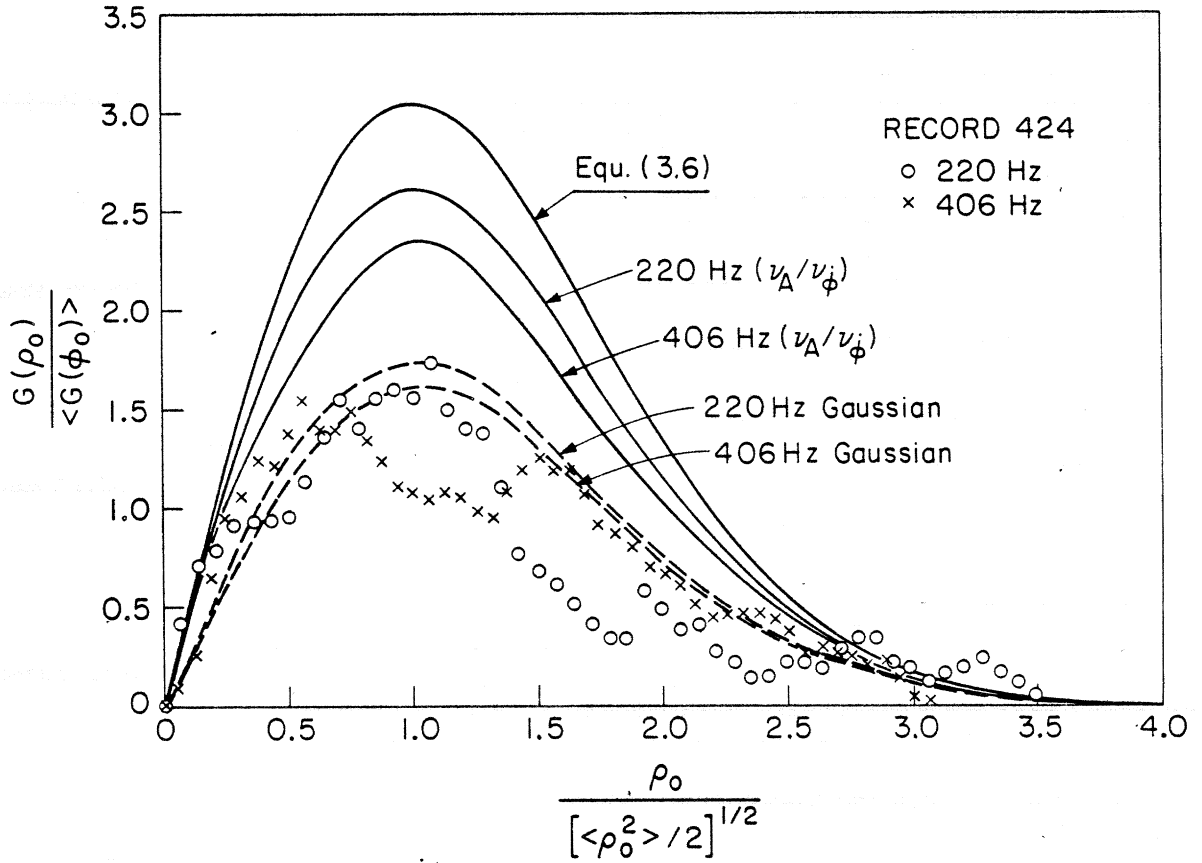
Fig. 67 Ratio of phase period to amplitude period, versus amplitude, for record 424. Equ. (3.6) is the theoretical ratio for a non-modulated narrowband source. The correction factors \nu_A/\nu_\phi (Table XV), and Equ. (1.209) (Gaussian modulation) have been applied to obtain the corrected curves for 220 Hz and 406 Hz accounting for the modulation.
