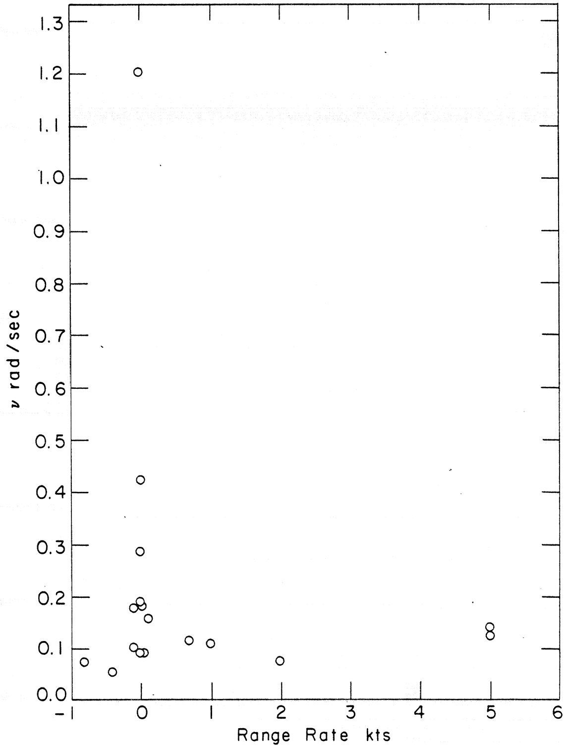
Fig. 83 A plot of \nu vs. range rate for the 15 Hz signal measured at receiver 1.
