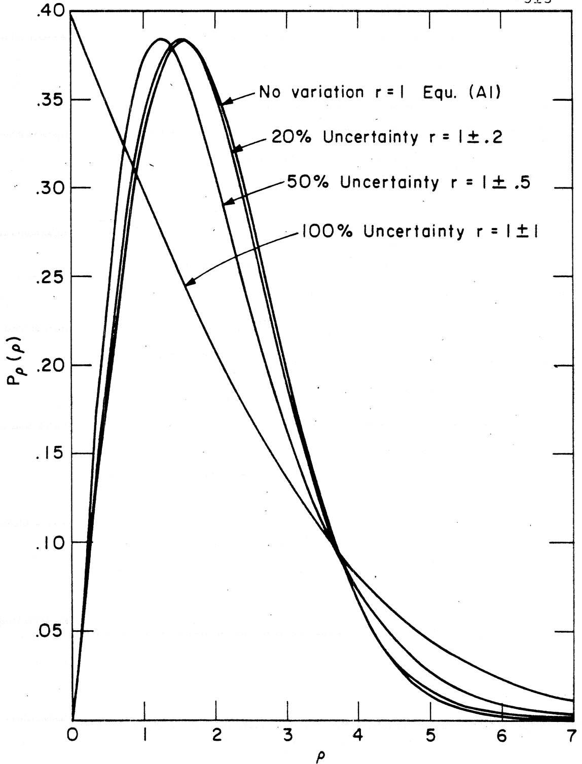
Fig. D1 Comparison plot of the effect of amplitude variation on the pdf for \rho . Equ (A1) is plotted with equ (D3) with various levels of uncertainty. N = 5 paths.
