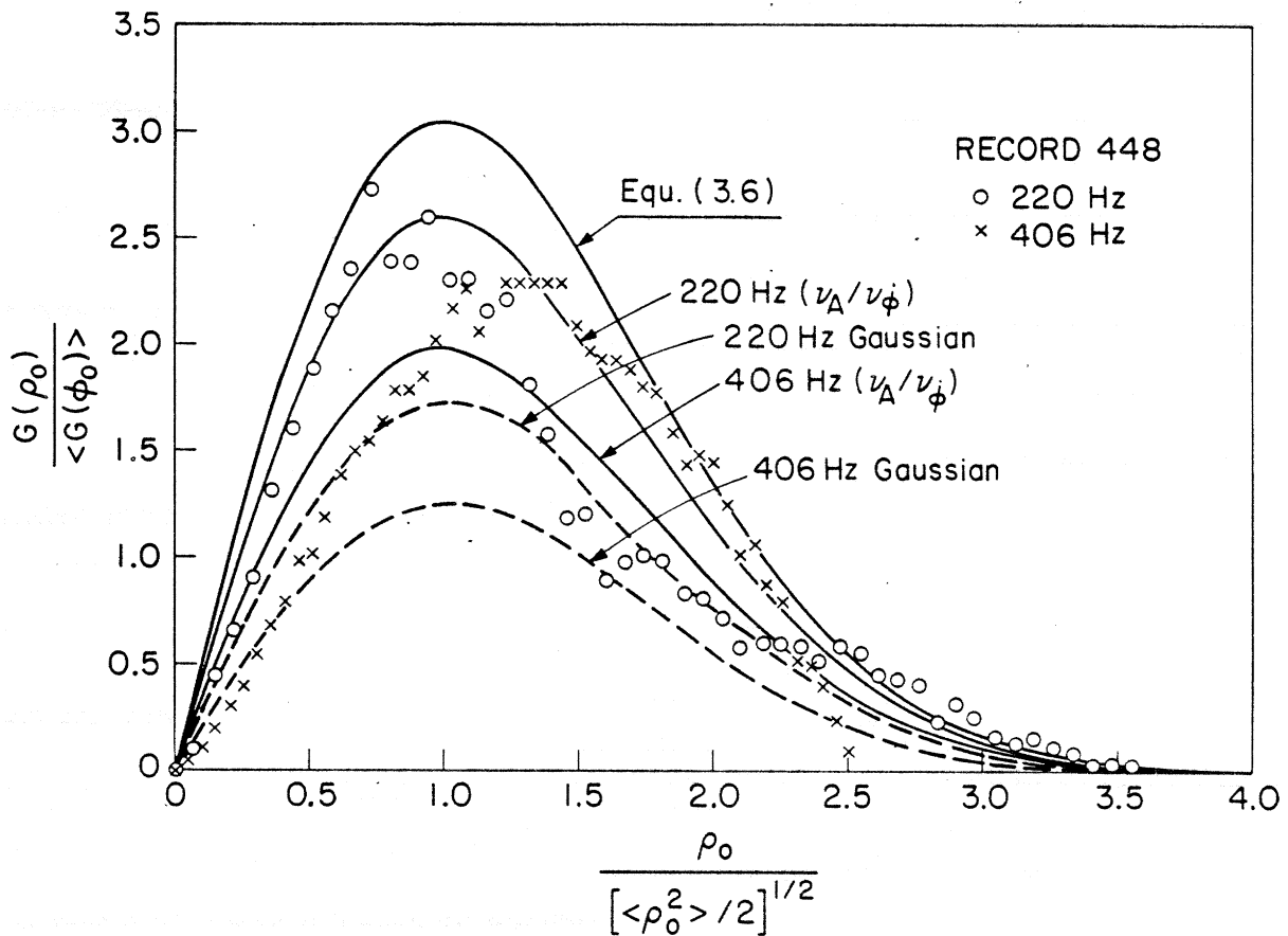
Fig. 65 Ratio of phase period to amplitude period, versus amplitude, for record 448. Equ. (3.6) is the theoretical ratio for a non-modulated narrowband source. The correction factors \nu_A/\nu_\phi (Table XV), and Equ. (1.209) (Gaussian modulation) have been applied to obtain the corrected curves for 220Hz and 406 Hz accounting for the modulation.
