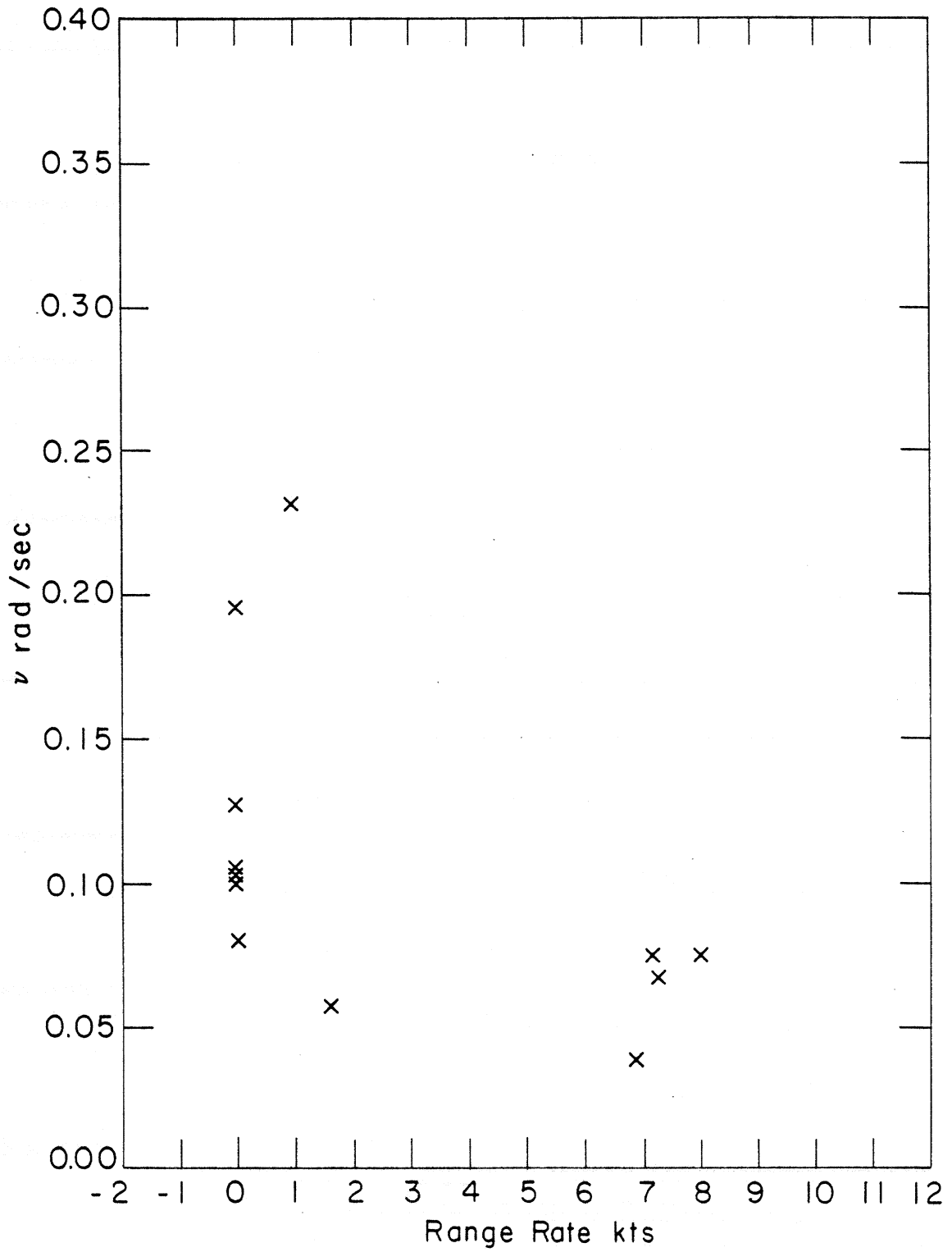
Fig. 82 A plot of \nu vs. range rate for the 33Hz signal measured at receiver 3.
