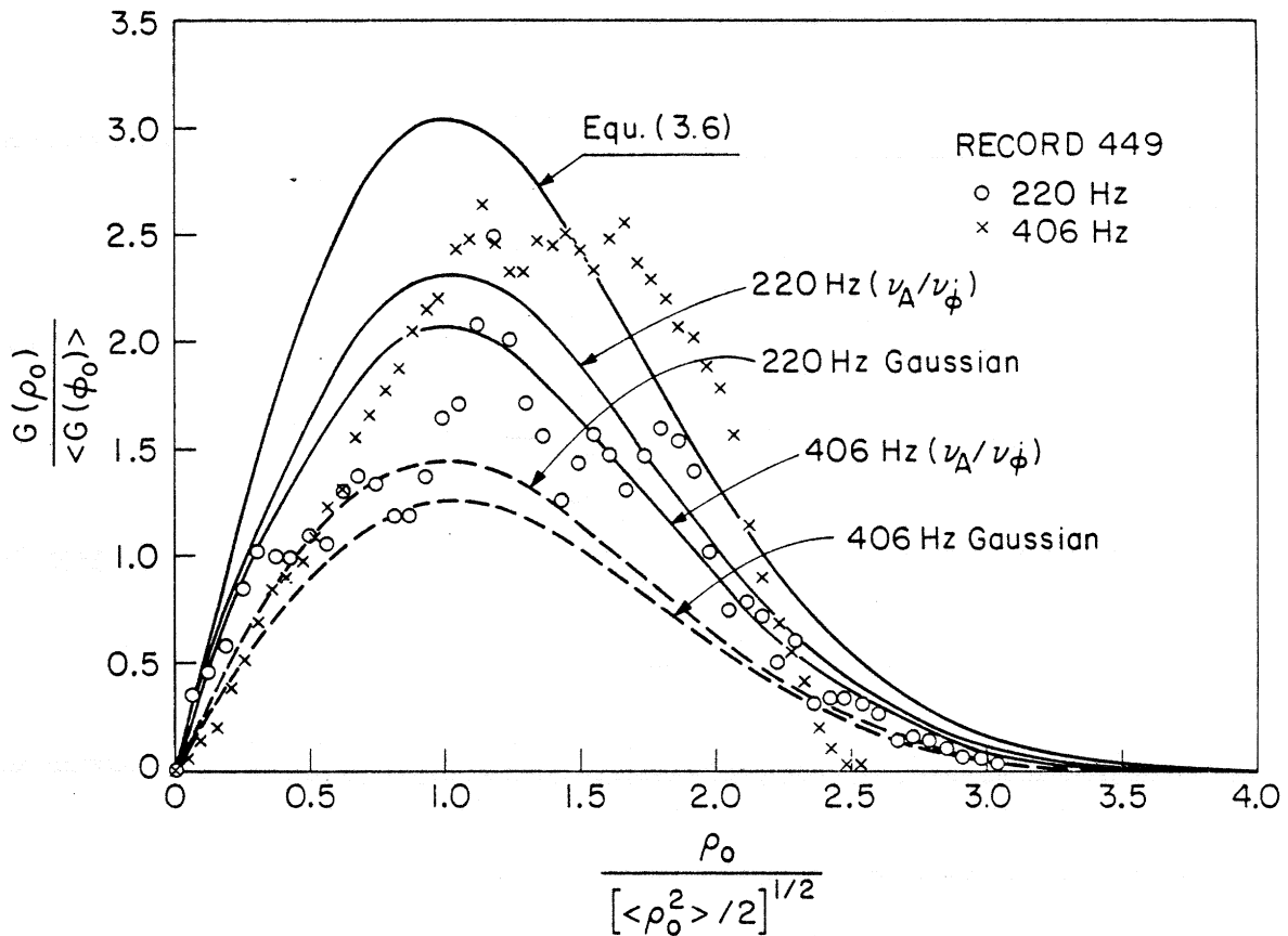
Fig. 66 Ratio of phase period to amplitude period, versus amplitude, for record 449. Equ. (3.6) is the theoretical ratio for a non-modulated narrowband source. The correction factors \nu_A/\nu_\phi (Table XV), and Eq. (1.209) (Gaussian modulation) have been applied to obtain the corrected curves for 220Hz and 406 Hz accounting for the modulation.
