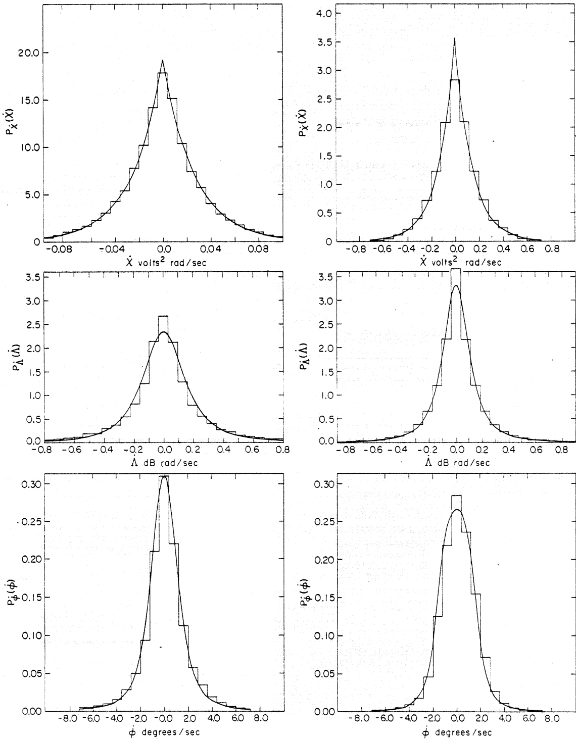
Fig. 57 Histograms from Record 448 for \dot{X} , \dot{\Lambda} , and \dot{\phi} , and the least chi-square fit of eqs. (1.4), (1.7), and (1.176), respectively. Results for 220 Hz are on the left, and 406 Hz on the right.
