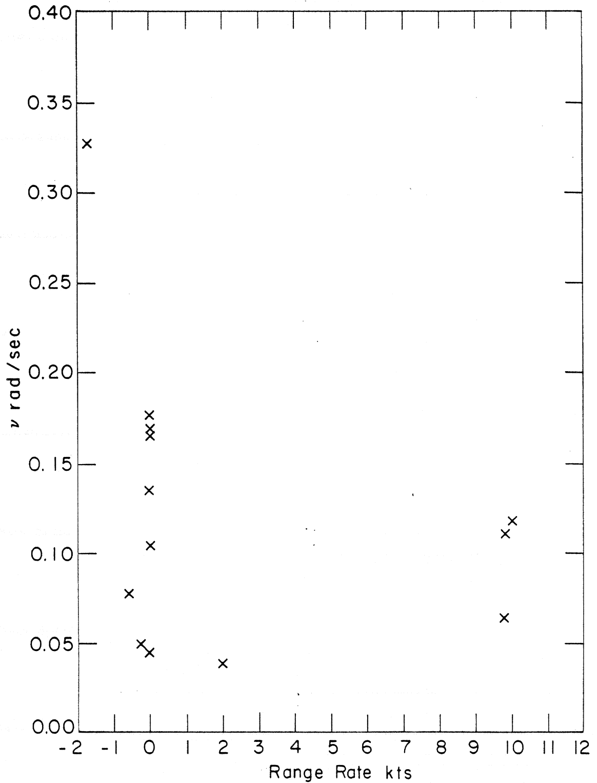
Fig. 80 A plot of \nu vs. range rate for the 33 Hz signal measured at receiver I.
