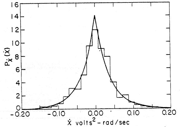
Fig. 17 Computer generated histogram of \dot{X} for N=5 paths and equ. (1.4).
